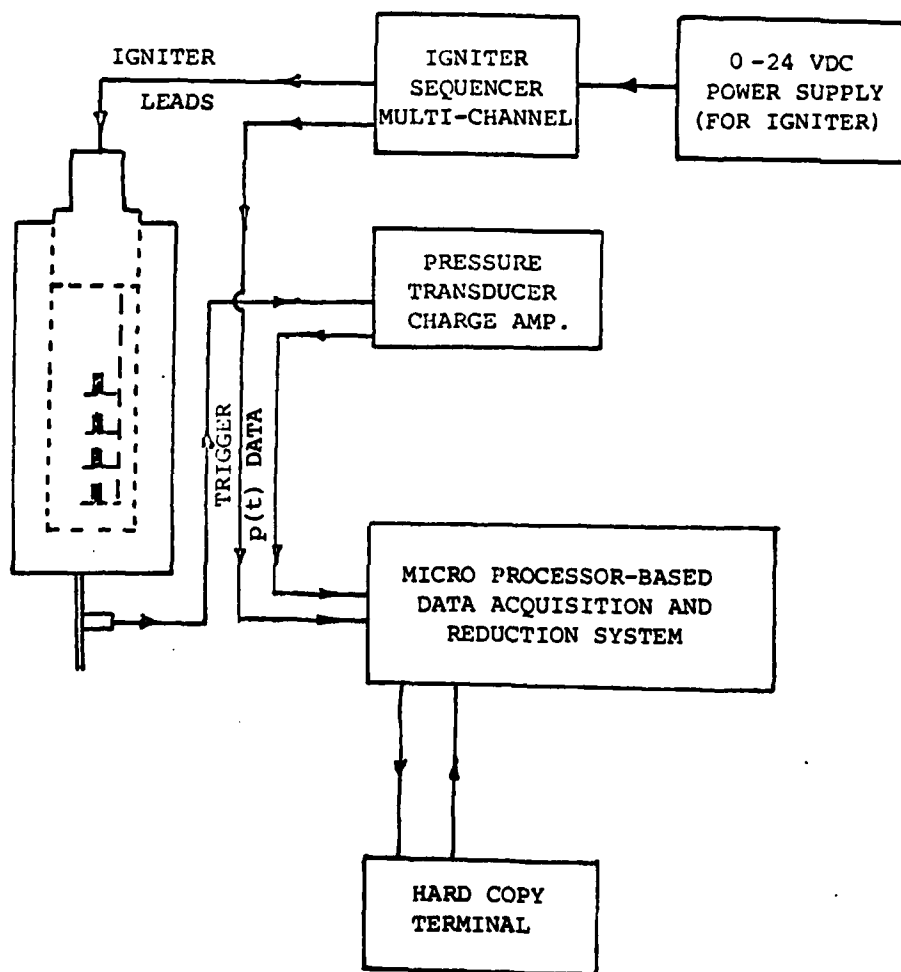
Fig. C-2 Instrumentation Approach 2 -- Microprocessor-based data acquisition and reduction system. Burning time intervals and mean pressure are calculated from the raw data and displayed on the hard copy terminal.
