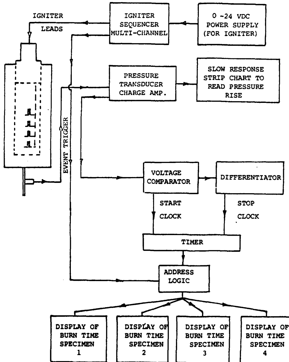
Fig. C-3 Instrumentation Approach 3 -- Dedicated multi-specimen timers. Burning times are displayed digitally for each specimen and mean pressure during each test is taken directly from slow response strip chart recorder.
