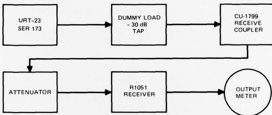
Figure 15. Transmitter noise measurement configuration.
