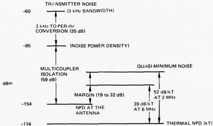
Figure 8. Power budget for transmitter broadband noise isolation (2-6 MHz).
