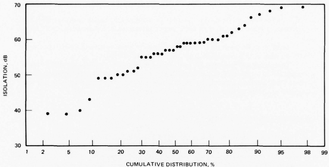
Figure 9. SRA-56 multicoupler isolation at 15% frequency separation: cumulative distribution.
