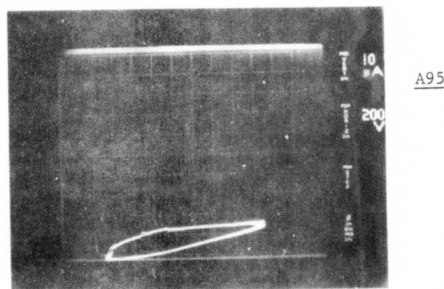
Figure 5. Two-point probe characteristics of undoped layers.
