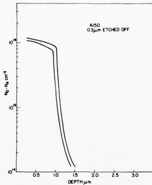
Figure 10. Carrier profile of Al50 from automatic profile plotter (CV measurement).
