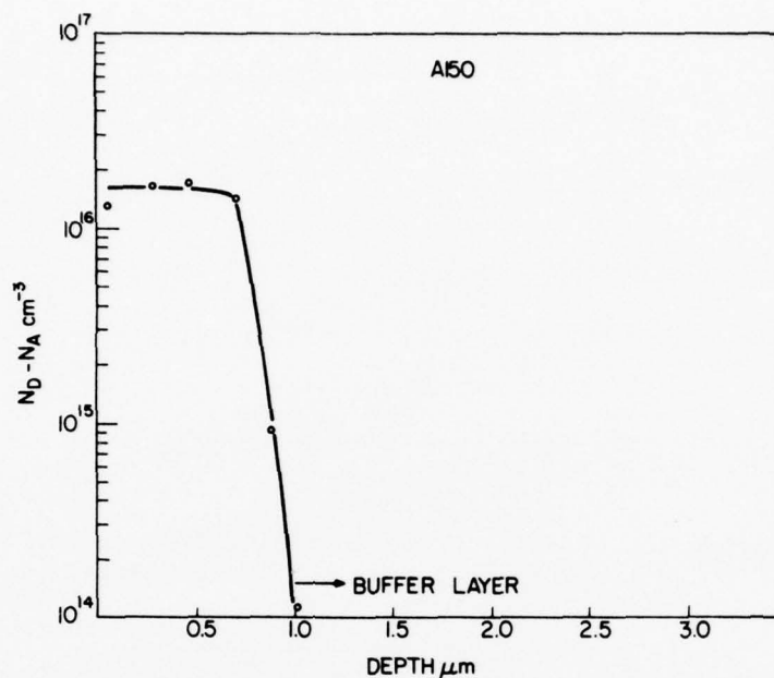
Figure 9. Carrier profile of Al50 n-layer/buffer layer wafer deduced from conductivity measurements.
