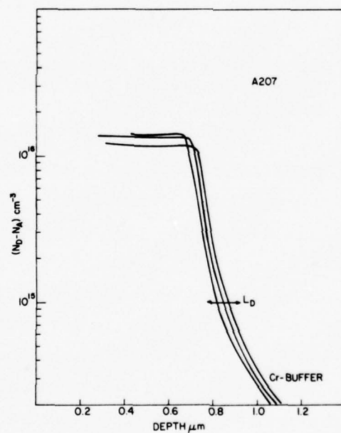
Figure 11. Carrier profile of n-buffer layer wafer. Note sharp boundary.
