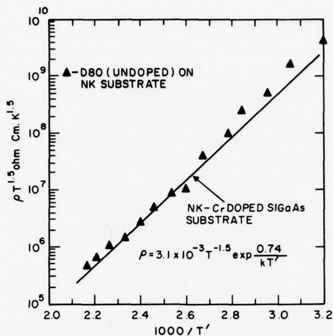
Figure 23. \rho T^{1.5} data points for D80 on NK substrate. The straight line is the characteristic of the substrate alone.
