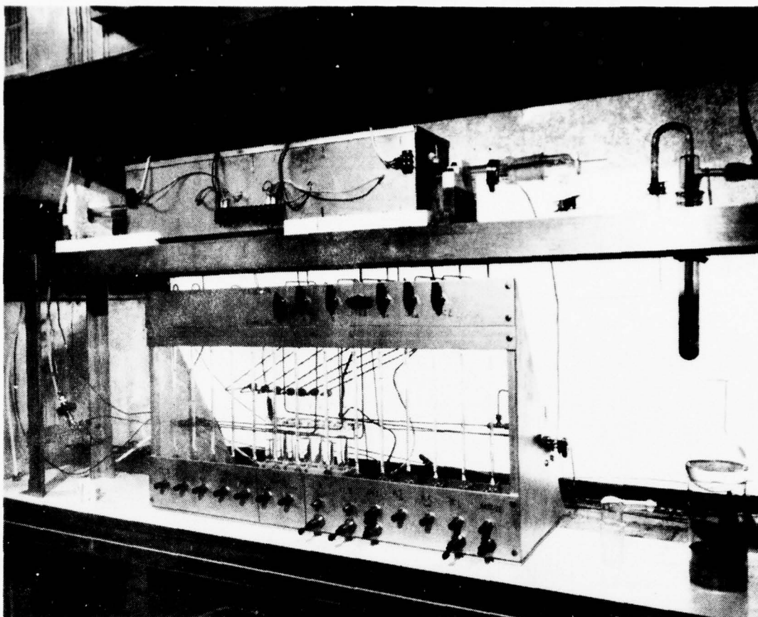
Figure 4. Photograph of reactor.
