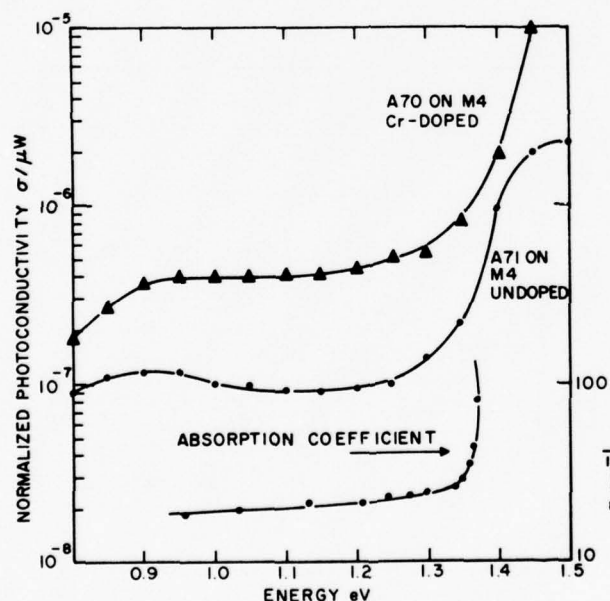
Figure 18. Photoconductive response of high resistivity epi layers on SI GaAs substrate (M4). Absorption coefficient plot also shown.
