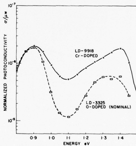
Figure 17. Nominally O-doped and Cr-doped SI GaAs substrates. Note similar photoconductive response.
