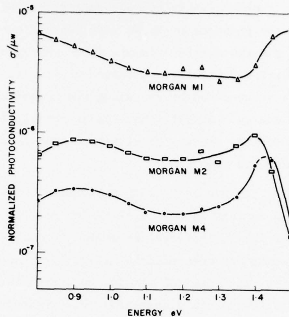
Figure 16. Photoconductive response of three Morgan Cr-doped SI GaAs substrates.
