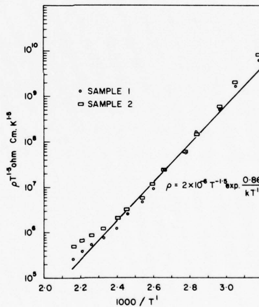
Figure 20. \rho T^{1.5} as a function of 1000/T' for Morgan M4 substrates.
