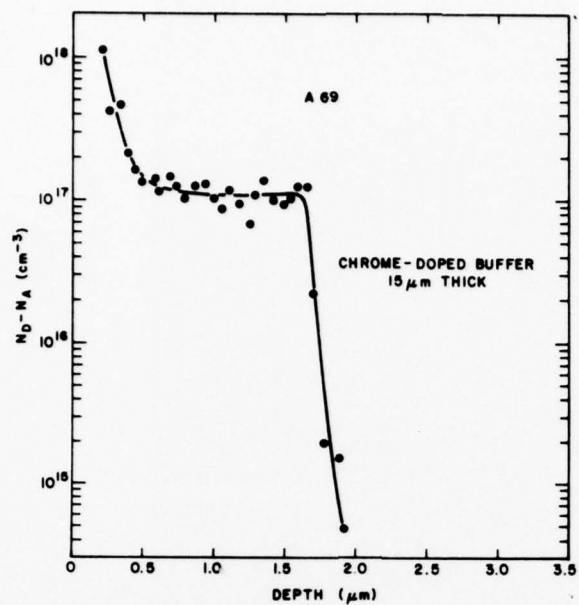
Figure 7. Carrier-concentration profile of wafer A69.
