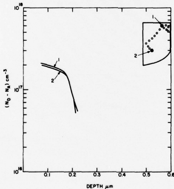
Figure 27. Carrier density profile for double Si implant. 1.5 \times 10^{12} \text{ cm}^{-2} at 70 keV and 3 \times 10^{12} \text{ cm}^{-2} at 200 keV.
