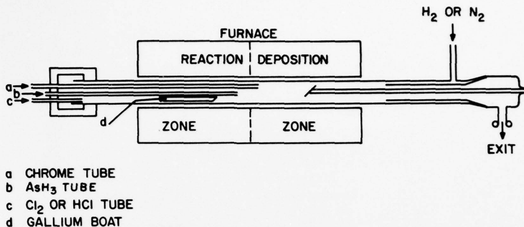
Figure 3. Schematic diagram of reactor tube/furnace assembly.
