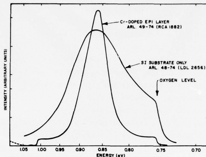
Figure 1. Photoconductivity response of bulk Cr-doped substrate and epitaxial Cr-doped buffer layer. Measurement made at AFAL, Dayton, Ohio.
