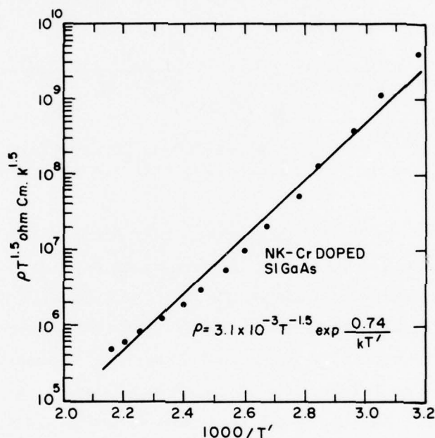
Figure 22. \rho T^{1.5} as a function of 1000/T' for NK SI GaAs substrate.
