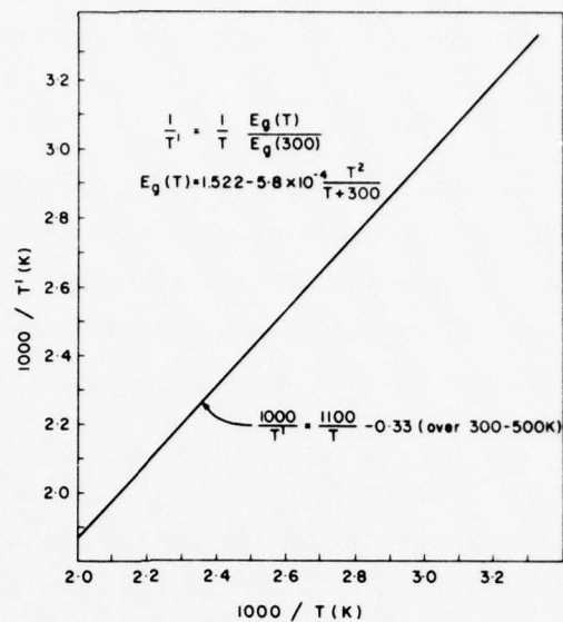
Figure 19. Plot of 1000/T' as a function of 1000/T .
