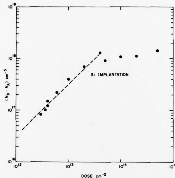
Figure 28. Carrier concentration as function of dose for Si implantation.
