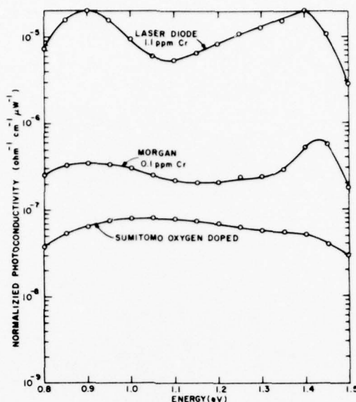
Figure 14. Room temperature photoconductivity response of SI GaAs substrate. Note evolution of a peak at \sim 0.9 eV as Cr-content increases.
