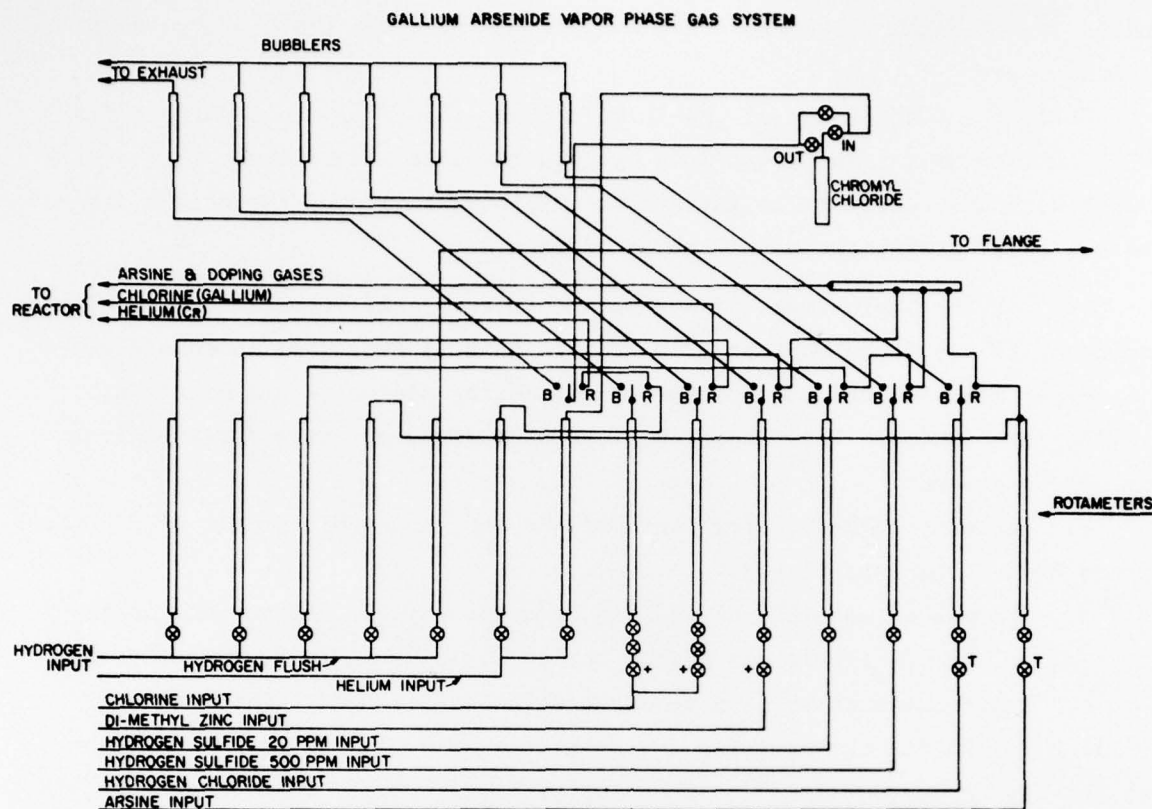
Figure 2. Schematic diagram of reactor gas-handling system.
