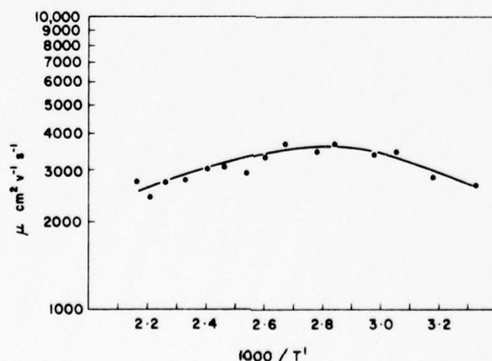
Figure 21. Hall mobility as a function of 1000/T' for Morgan M4 substrate.
