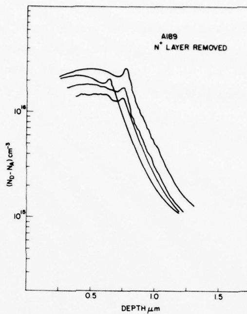
Figure 12. Profile of N^+ -n-buffer layer wafer grown with silane.
