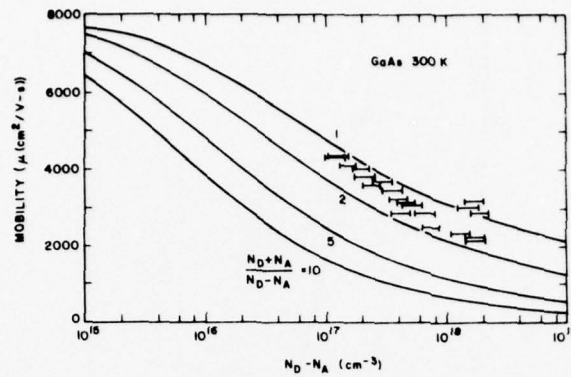
Figure 24. Electron mobility-carrier density plot for S implantation.
