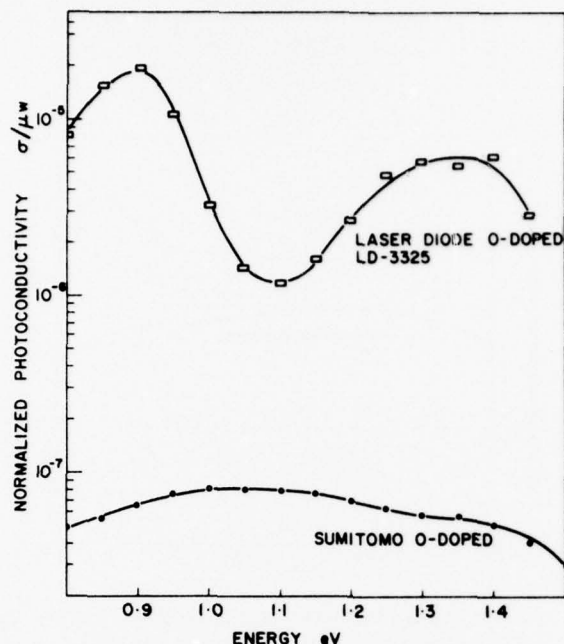
Figure 15. Photoconductive response of two nominally O-doped SI GaAs substrates.
