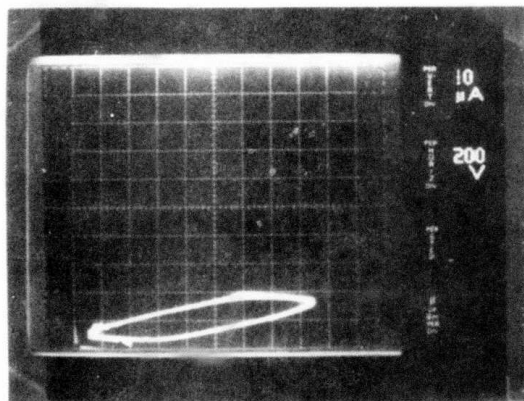
Figure 6. Two-point-probe data for Cr-doped epi layers.
