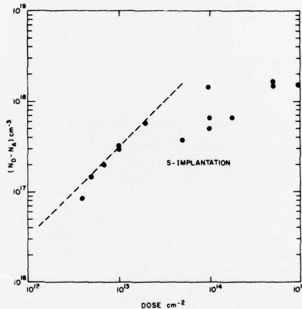
Figure 25. Carrier concentration as a function of dose for S-implantation.
