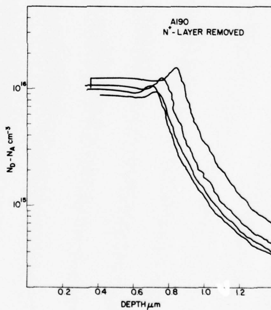
Figure 13. Profile of N^+ -n-buffer layer wafer. N^+ layer grown using silane.
