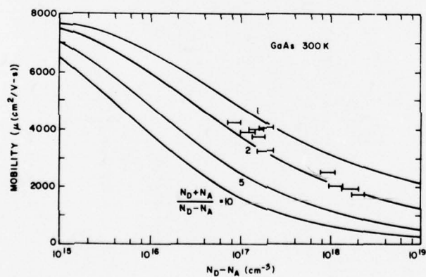
Figure 29. Electron mobility-carrier density plot for Si implantation.
