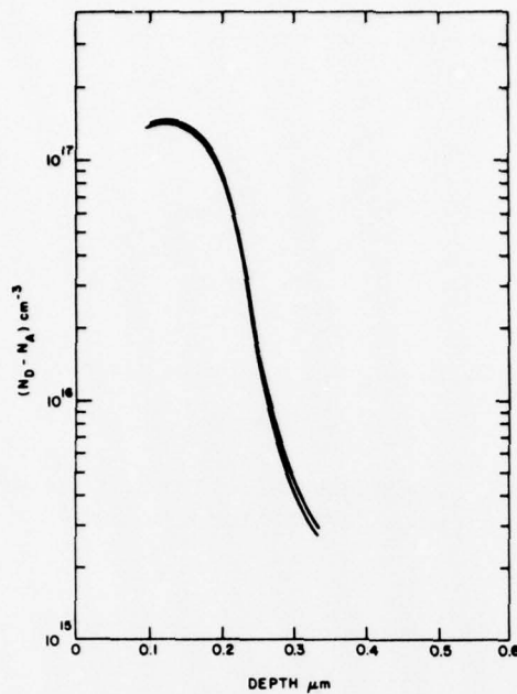
Figure 26. Carrier density profile for single Si implant 3.5 \times 10^{12} \text{ cm}^{-2} at 200 keV.
