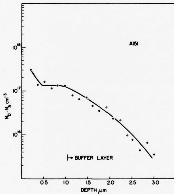
Figure 8. Carrier profile of A151 showing washed out buffer layer.
