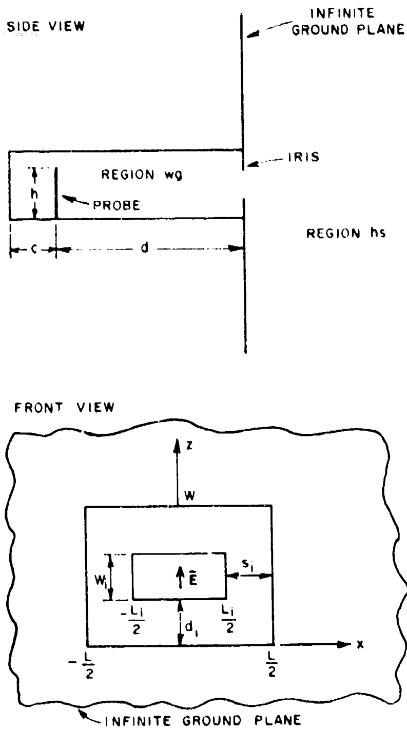
Figure 3-2. Rectangular waveguide-fed aperture with an iris.
