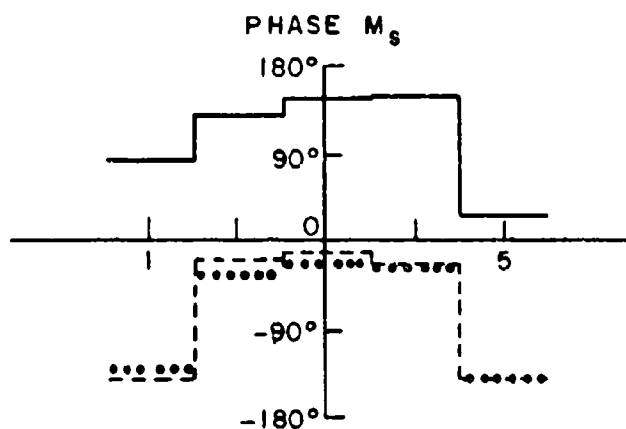
Figure 4-16. Aperture distributions in the vicinity of the array edge along the center column of an 11x11 array of square waveguide-fed elements. Position number one refers to the lower edge of each aperture.
