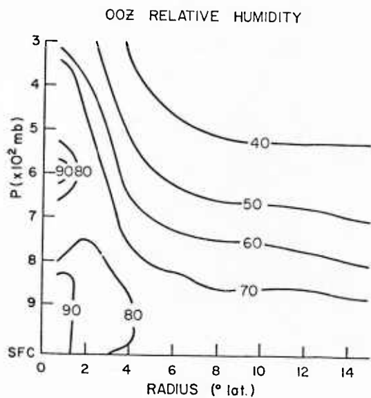
Fig. 29. 00Z relative humidity for the mean steady state hurricane ( \sim 1900 local time).
