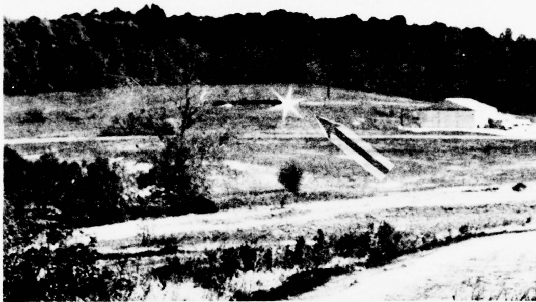
Figure 16. Glint From Soft Mockup of Flat-Plate OH-58 Canopy
