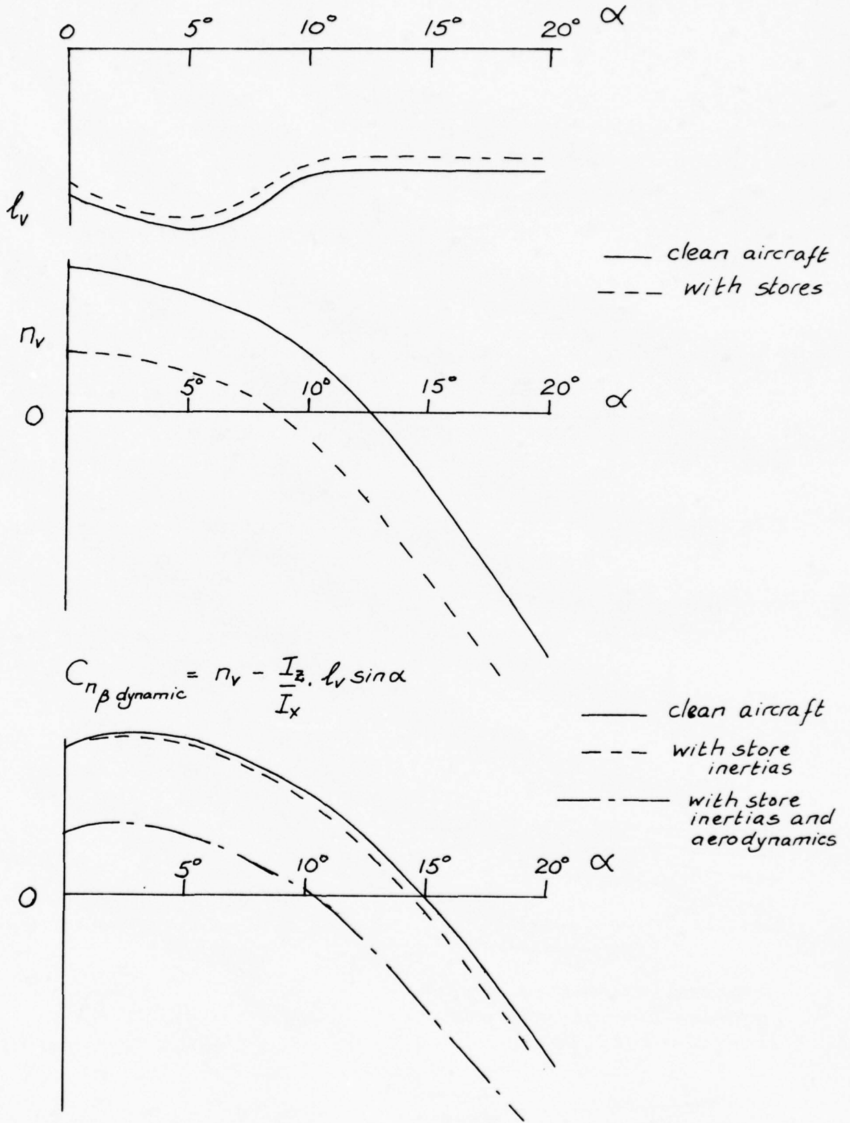
Fig 5 Degradation of lateral stability at high incidence
