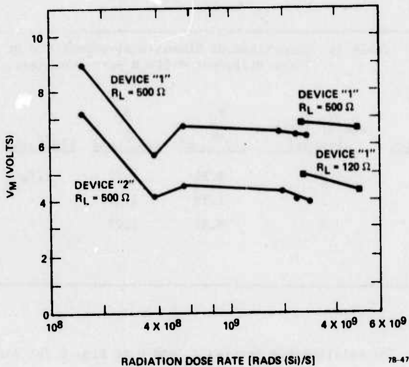
FIG. 6 Maximum voltage V_M for type "B" \text{SiO}_x\text{N}_y -p-n + device as a function of radiation dose rate.
