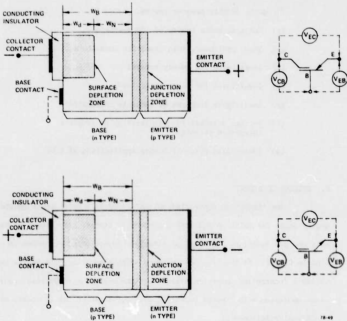
FIG. 1 Cross sectional diagram of basic inversion-controlled switch structures and circuit symbols. Top: M-I-n-p structure. Bottom: M-I-p-n structure.
