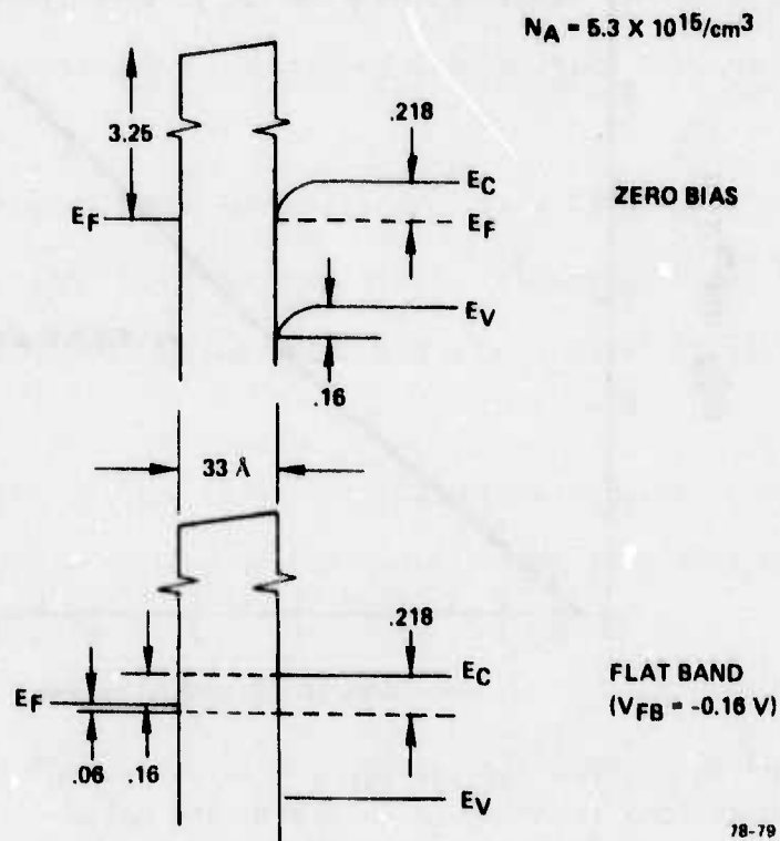
FIG. 31 Energy band diagram of Mo-SiO 2 -n-p + device at surface. Uniform properties of thick SiO 2 layers are assumed.
