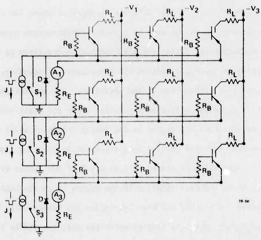
FIG. 8 Circuit diagram of 3 x 3 RAM array with isolated emitter and base rows.
