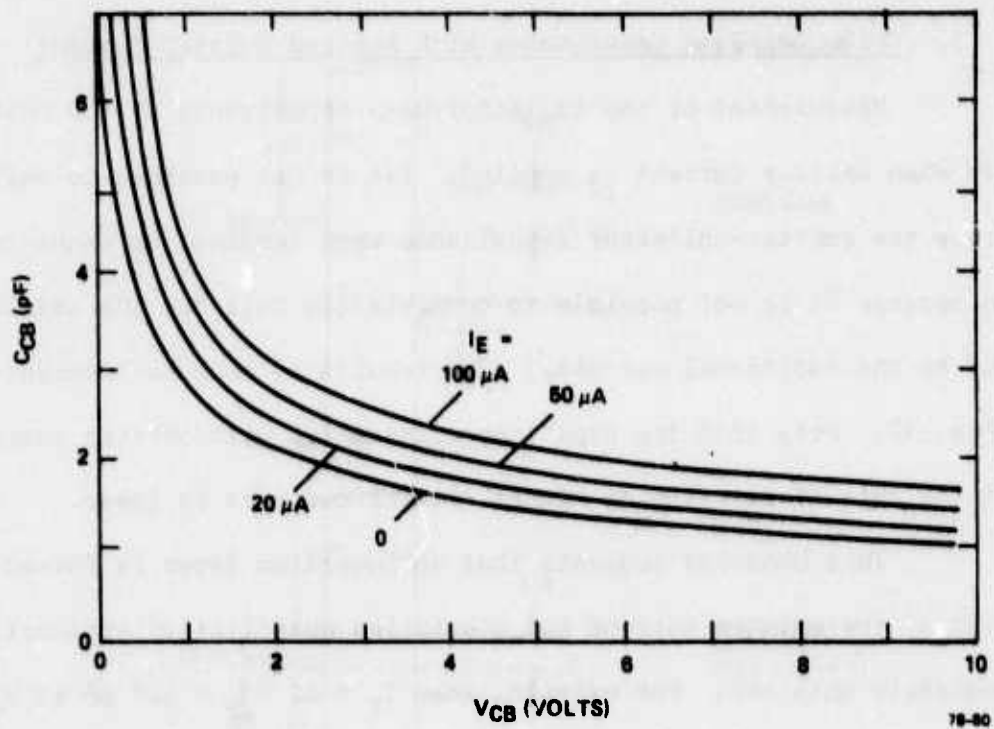
FIG. 32 Capacitance as a function of voltage for collector-base terminals of Mo-SiO 2 -n-p + ICS device. Emitter current is varied in different traces.
