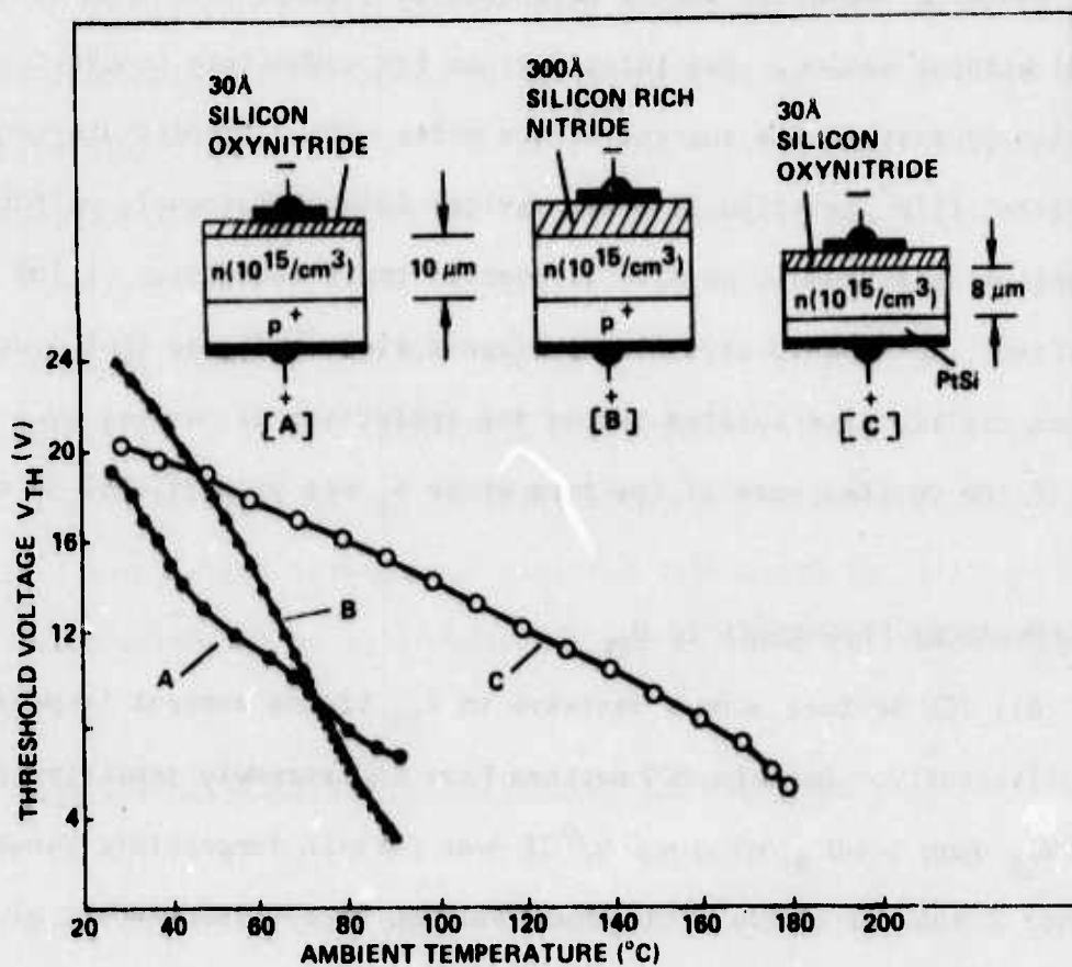
FIG. 6 Diode threshold voltage V_{TH} as a function of ambient temperature for three different ICS structures, all fabricated from the same silicon material which had a relatively lightly doped base region.
