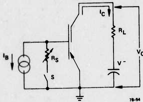
FIG. 6 Circuit used to obtain three-terminal I-V data. Switch S is open for data of Fig. 5; switch S is closed for data of Fig. 7.
