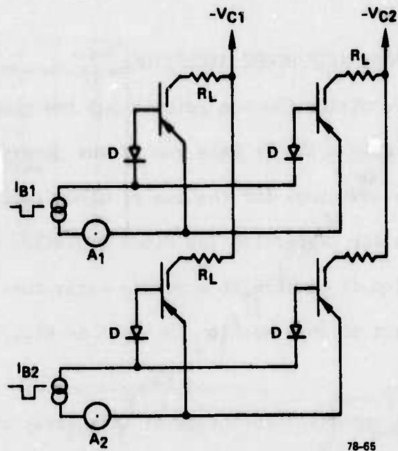
FIG. 17 Memory array with diode isolation between base line and individual base terminals within a row.
