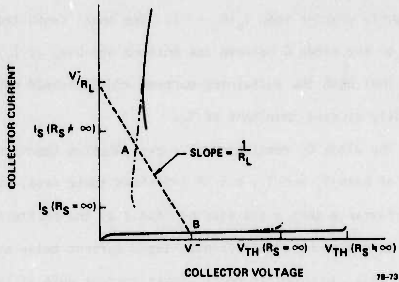
FIG. 25 I-V characteristics of ICS transistor illustrating requirements for nonlatching operation.
