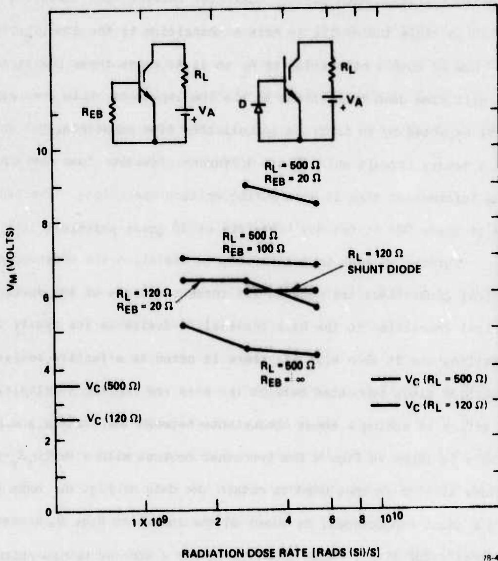
FIG. 9 V_M as a function of radiation dose rate for type "A" \text{Mo-SiO}_x \text{N}_y\text{-p-n}^+ devices for several three terminal circuit arrangements.
