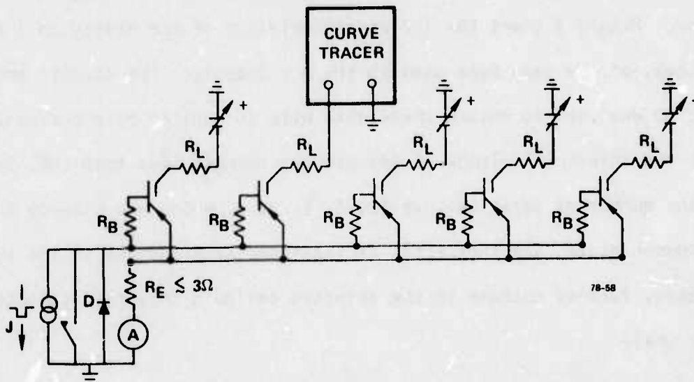
FIG. 10 Circuit used to determine I-V characteristics of a single device in a five-element row.
