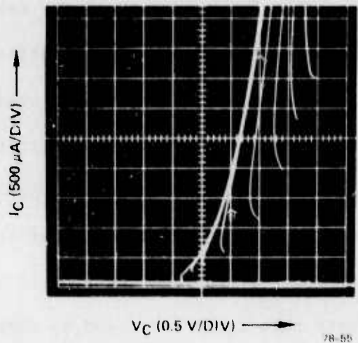
FIG. 7 Grounded emitter characteristics of Mo-SiO 2 -n-p + device with R_s = \infty, 10\text{ K}, 4\text{ K}, 2\text{ K}, 500, 200 and 0\ \Omega . As R_s decreases, I_s and V_s increase.
