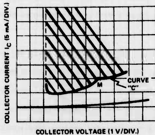
FIG. 7 Grounded base characteristics of same device used in obtaining data of Fig. 6. Straight-line characteristics were produced by a continuous increase of R_S from 10 \Omega until device switched out of low impedance state. Dotted line shows low impedance state characteristic when R_S = 10 \Omega ; the curve C marks the lower limit of the low impedance state.
