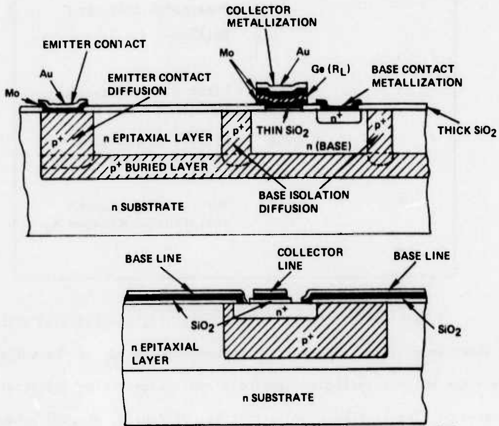
FIG. 20 Cross sectional views of various portions of integrated array.
