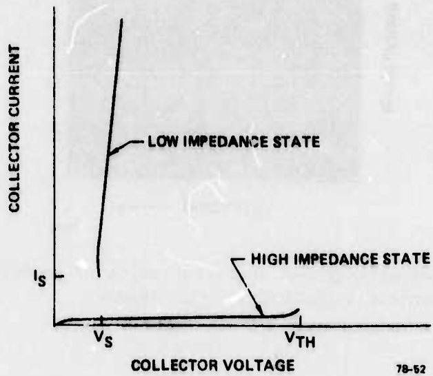
FIG. 4 Current-voltage characteristics of ICS, including graphical definitions of threshold voltage V_{TH} , sustaining voltage V_s and sustaining current I_s .
