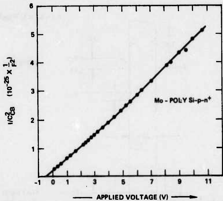
FIG. 30 1/C^2 vs applied voltage for a Mo-poly Si-p-n + ICS device. Terminal connections are made to collector and base.
