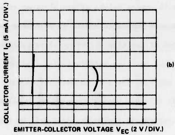
FIG. 3 I-V characteristics of ICS diodes. (a) Two stable impedance states of a metal-silicon oxynitride-p + -n-n + device. (b) Three stable impedance states of a metal-silicon oxynitride-p-n + device.
