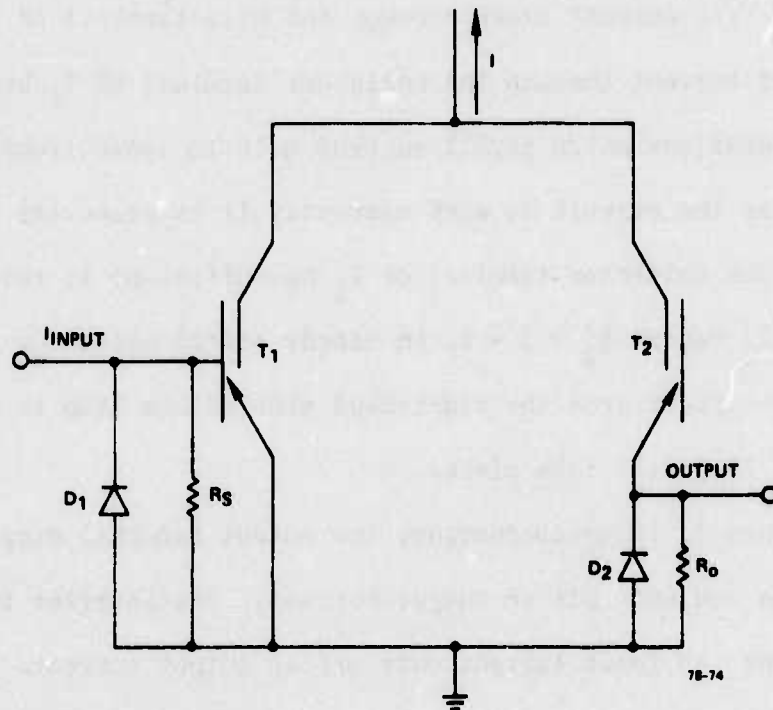
FIG. 26 Diagram of ICS inverter circuit.
