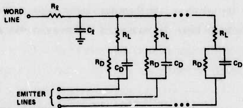
FIG. 24 Approximate equivalent circuit diagram of word-line address.
