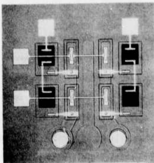
FIG. 21 Photomicrograph of completed 2 x 2 memory array circuit.
