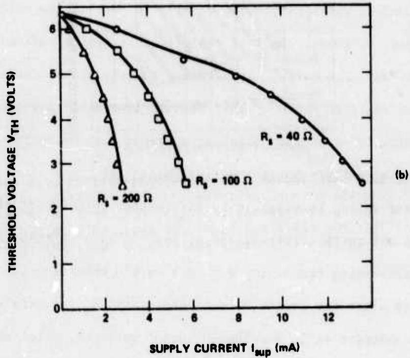
FIG. 8 Effect of emitter current on grounded base threshold voltage of a metal-SiO 2 -p-n-n device.
