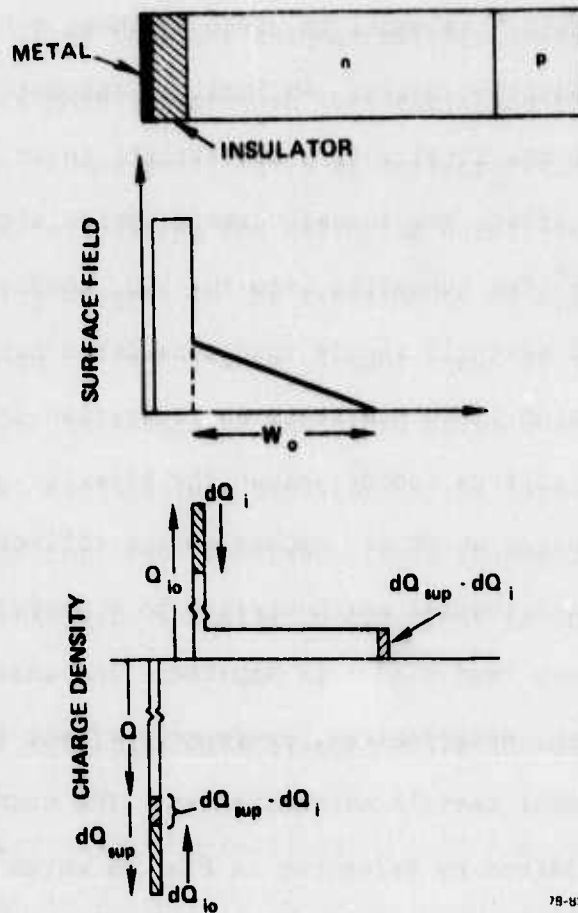
FIG. 33 Charge densities appearing on collector, inversion layer and edge of depletion layer in capacitance measurement.
