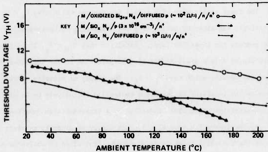
FIG. 7 Diode threshold voltage V_{TH} as a function of ambient temperature for three different ICS structures which had relatively heavily doped base regions.
