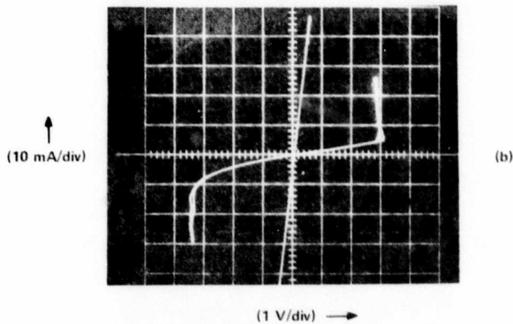
FIG. 3 Current-voltage characteristics of molybdenum – p-type polysilicon – molybdenum device. (a) Virgin state. (b) High and low impedance states.
