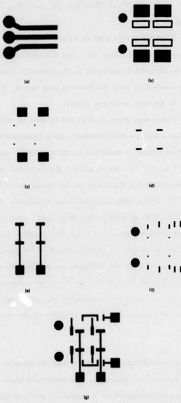
FIG. 19 Photoresist mask patterns used for fabricating 2 x 2 integrated memory array.
