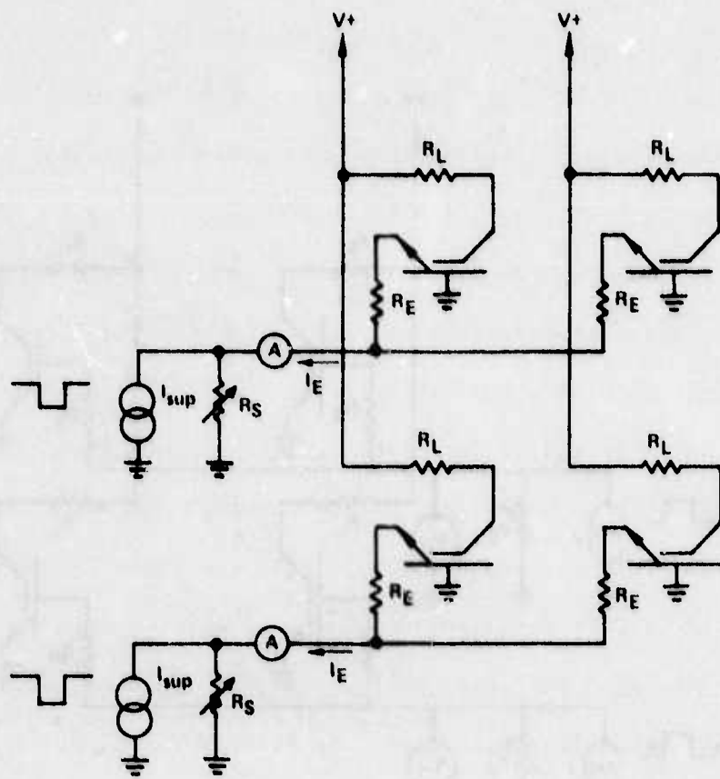
FIG. 3 Grounded base RAM circuit.
