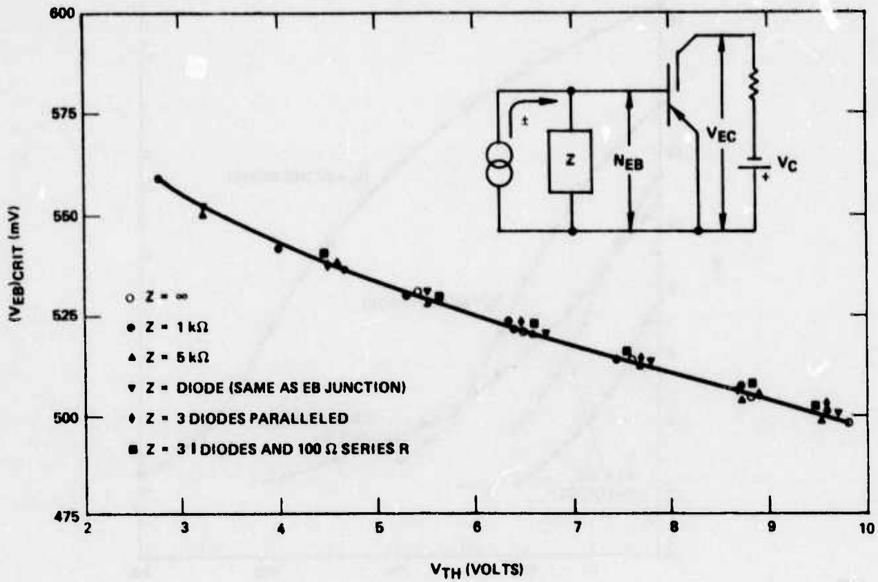
FIG. 13 Critical emitter-base potential when device is biased to V_{EC} = V_{TH} in high impedance state as a function of V_{TH} for various emitter-base shunt impedances.
