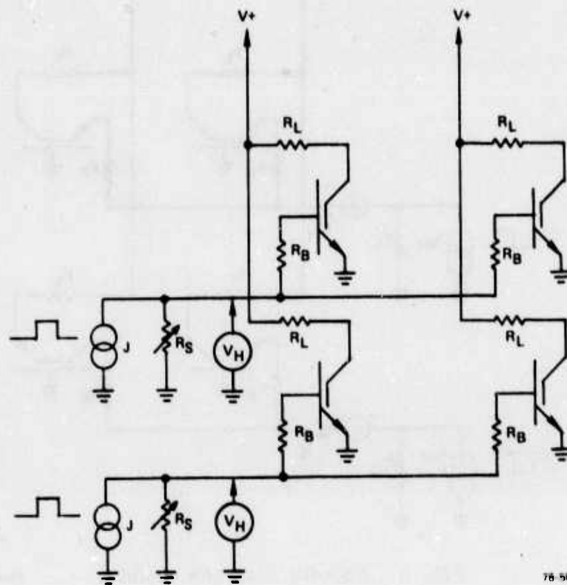
FIG. 2 Grounded emitter RAM circuit.
