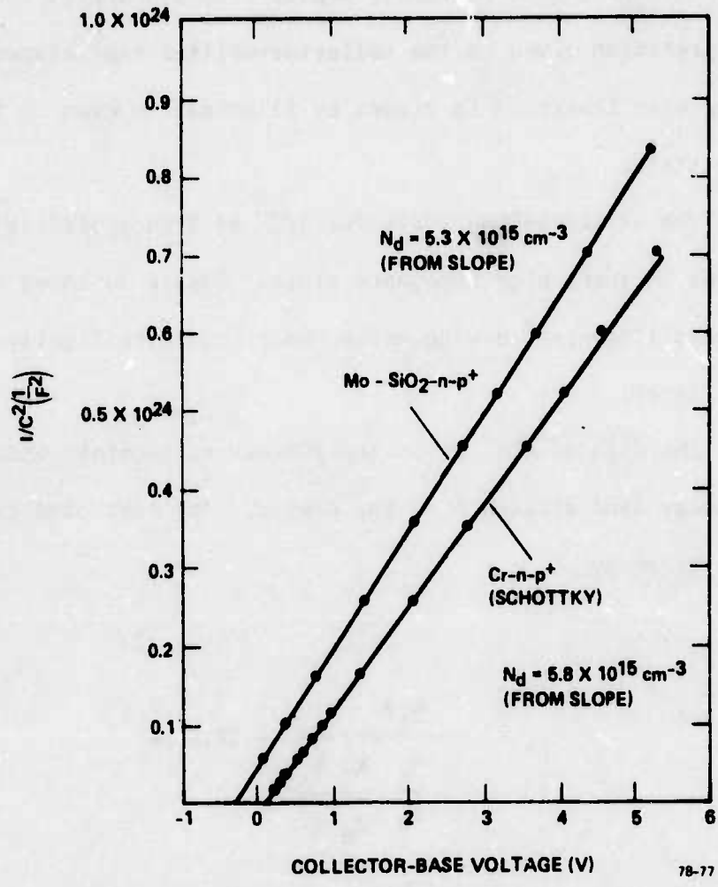
FIG. 29 1/C^2 vs V_{cb} applied voltage for Mo-SiO 2 -n-p + ICS device and a companion Cr-n-p Schottky-barrier device. Terminal connections are made to collector and base with emitter terminal open.
