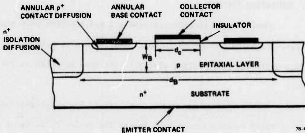
FIG. 3 Cross sectional view of typical ICS device studied, drawn for special case of M-I-P-N + device with epitaxially grown junction.
