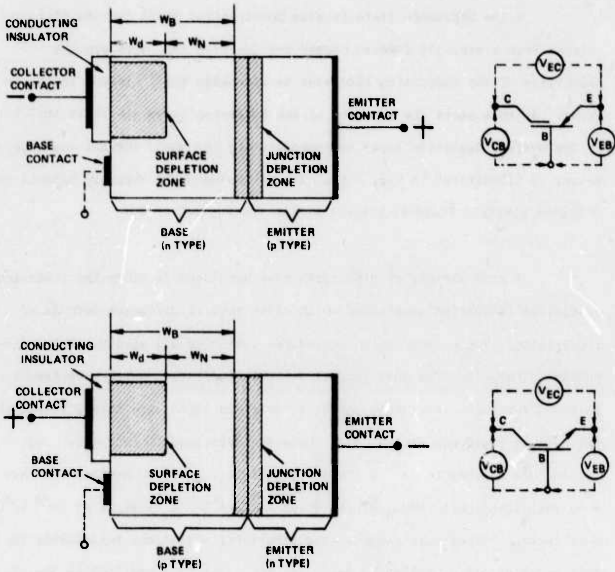
FIG. 1 Structure of inversion-controlled switches and proposed circuit symbols. Diagrams also illustrate definitions of base width W_B , surface depletion layer width W_d , and neutral layer width W_N . Top: M-I-n-p device and symbol with definition of terminal potential differences. Bottom: M-I-p-n device and symbol.
