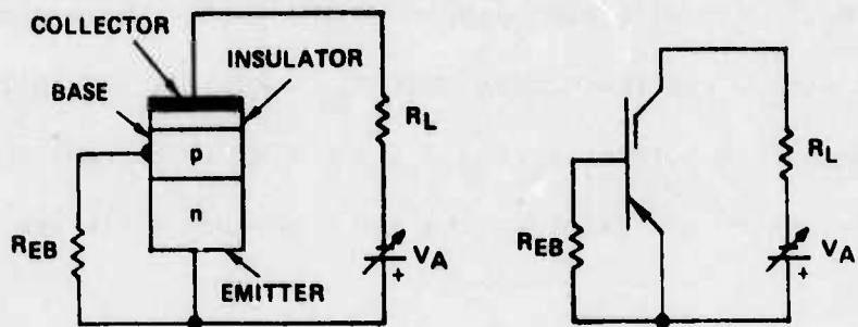
(a) M-INSULATOR -n-p
