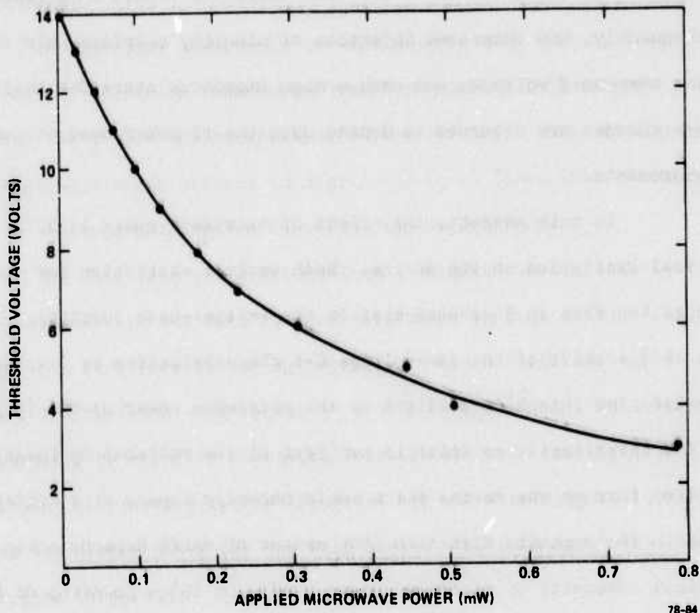
FIG. 35 Variation of Mo-SiO 2 -n-p + device's threshold voltage as a function of microwave power supplied at 2.0 GHz.
