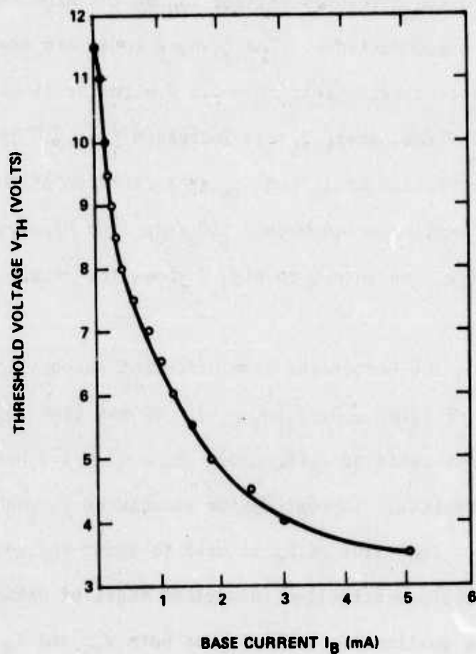
FIG. 2 Variation of grounded emitter threshold voltage V_{TH} as a function of applied base current I_B for a metal-silicon-rich, silicon nitride-p-n device.
