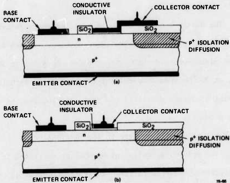
FIG. 18 Cross sectional views of discrete ICS device.
