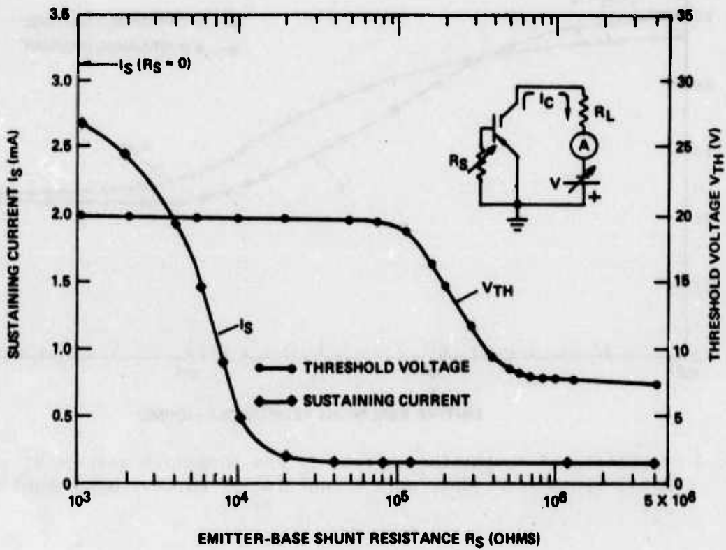
FIG. 3 Variation of sustaining current I_S and threshold voltage V_{TH} of a metal-SiO 2 -n-p + device as a function of emitter-base shunt resistance R_S .
