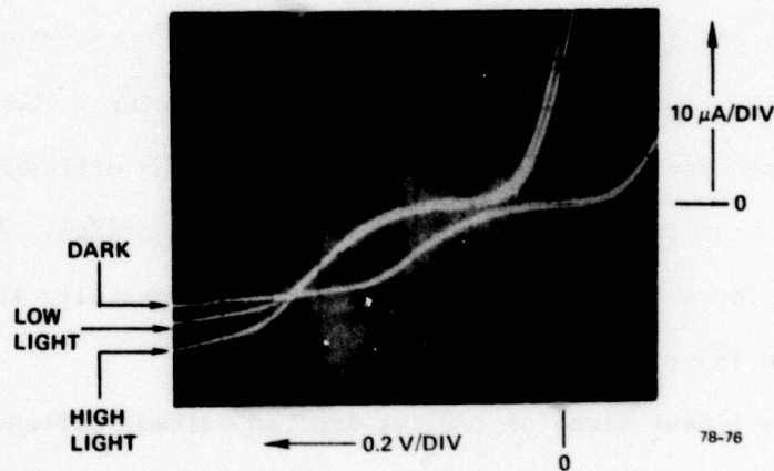
FIG. 28 Emitter-collector I-V characteristics of same device used to obtain data of Fig. 26 with identical conditions of illumination.
