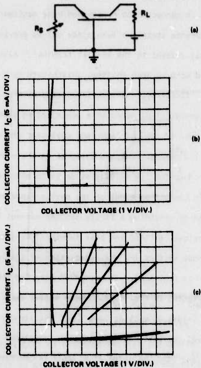
FIG. 6 Grounded base biasing of a metal-SiO x N y -p + -n-n + ICS device. (a) Grounded base circuit. (b) Grounded-emitter I-V characteristics shown for comparison. (c) Grounded-base characteristics with R_S \approx 0, 100, 200 and 400 ohms.
