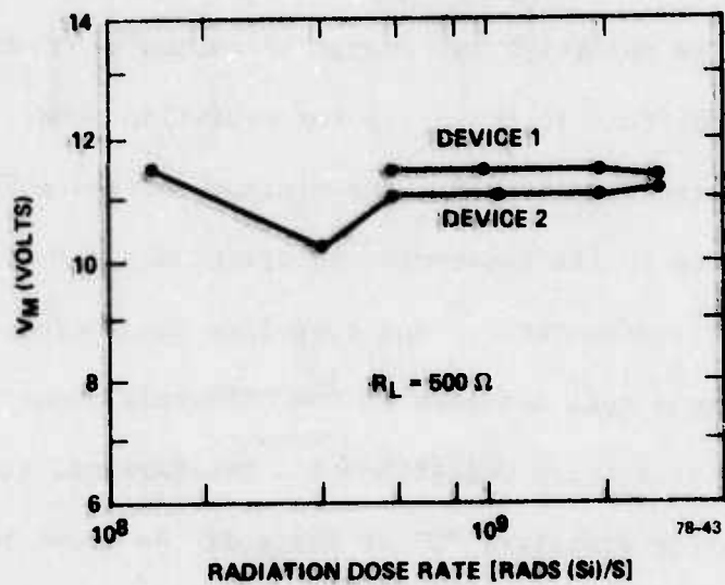
FIG. 10 V_M as a function of radiation dose rate for type "C" Mo-SiO x N y -p-n + devices.
