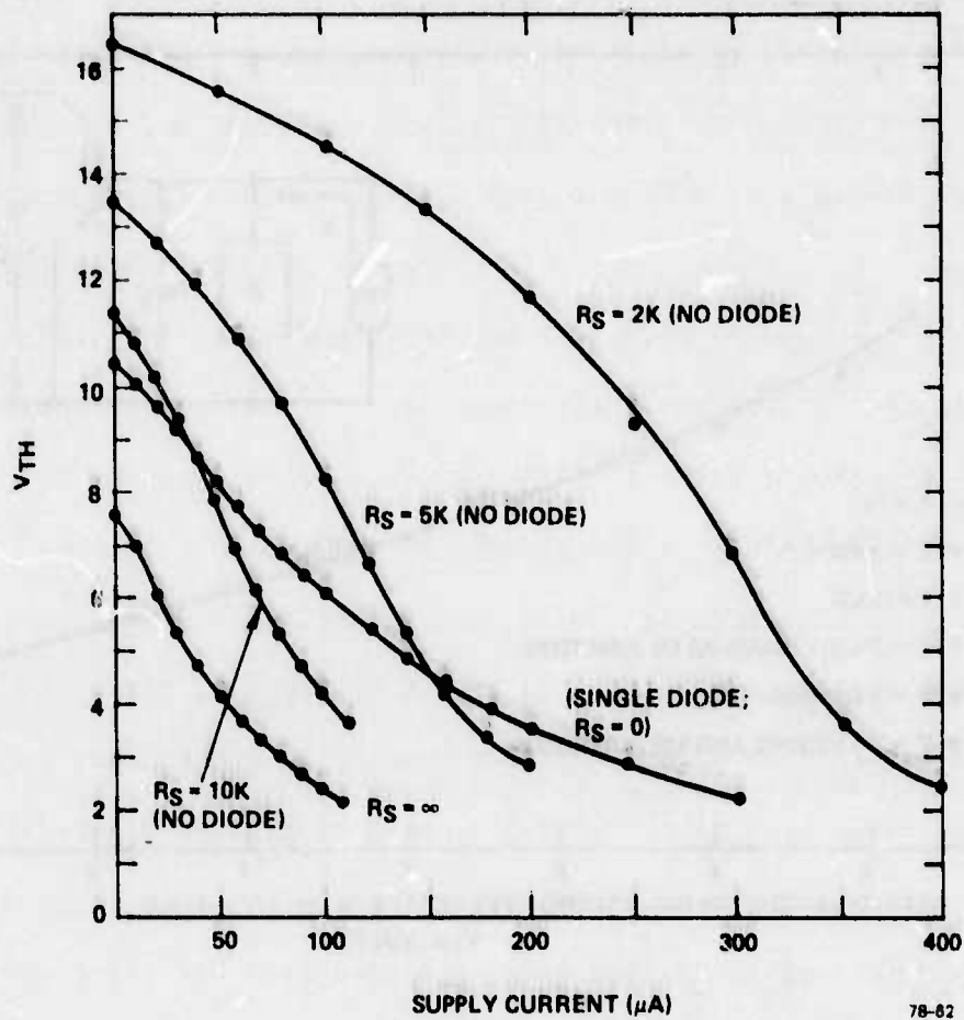
FIG. 14 Threshold voltage V_{TH} as a function of current drawn from base terminal when emitter-base terminals are shunted by various external impedances.
