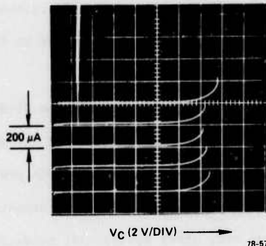
FIG. 9 I-V characteristic of device in row with four other devices with zero base current applied. Offset curves are for 0, 1, 2, 3 and 4 other devices in low impedance state. (Top trace is for no device in low impedance state.)
