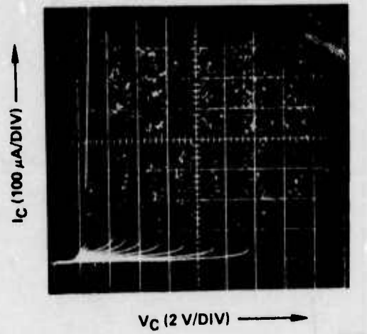
FIG. 5 Grounded emitter I-V characteristics of Mo-SiO 2 -n-p + ICS with base current increased in 5 μA steps.
