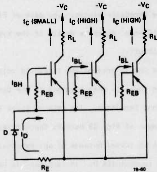
FIG. 12 Circuit diagram of 3-element row of memory array. Note different directions of base current for devices in high and low impedance states.
