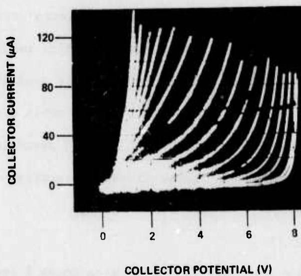
FIG. 37 I-V characteristics of a Mo-SiO 2 -n-p + device in high impedance state with various amounts of 1 2 GHz microwave power applied.
