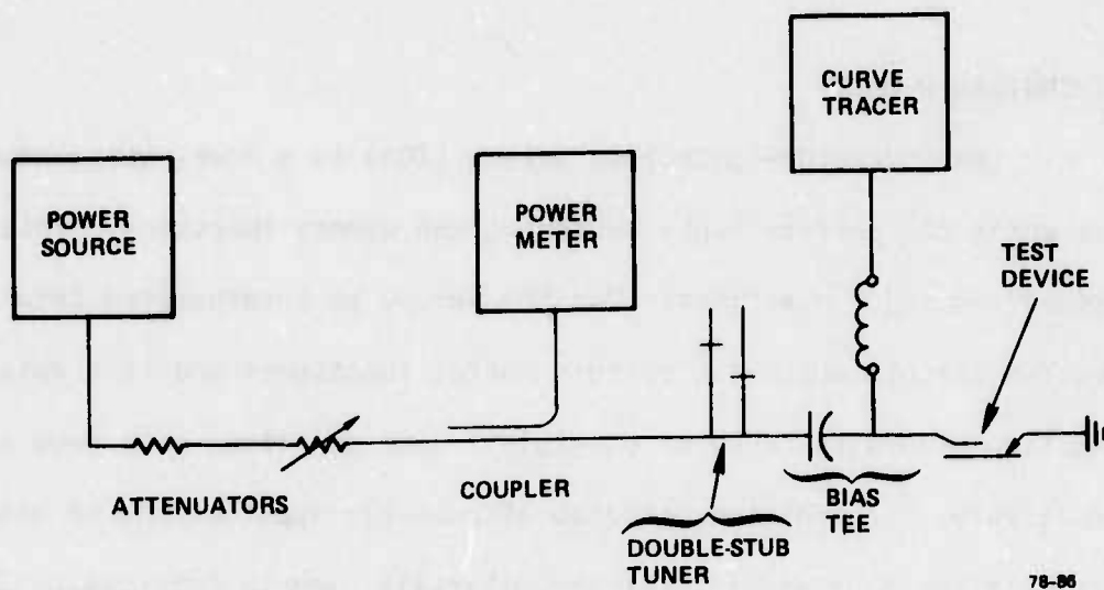
FIG. 36 Diagram of apparatus used to obtain data of Fig. 35.
