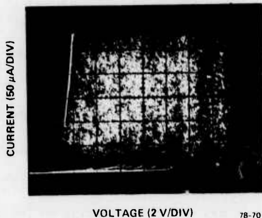
FIG. 22 Output characteristics of integrated device. Voltage is sum of voltage across emitter-collector terminals of the device and germanium collector load resistor. Base current drive (to entire row) is 0, 10, 20, 30, 40 and 50 \mu\text{A} with V_{\text{TH}} suppressed to 8 V from 12.4 V.
