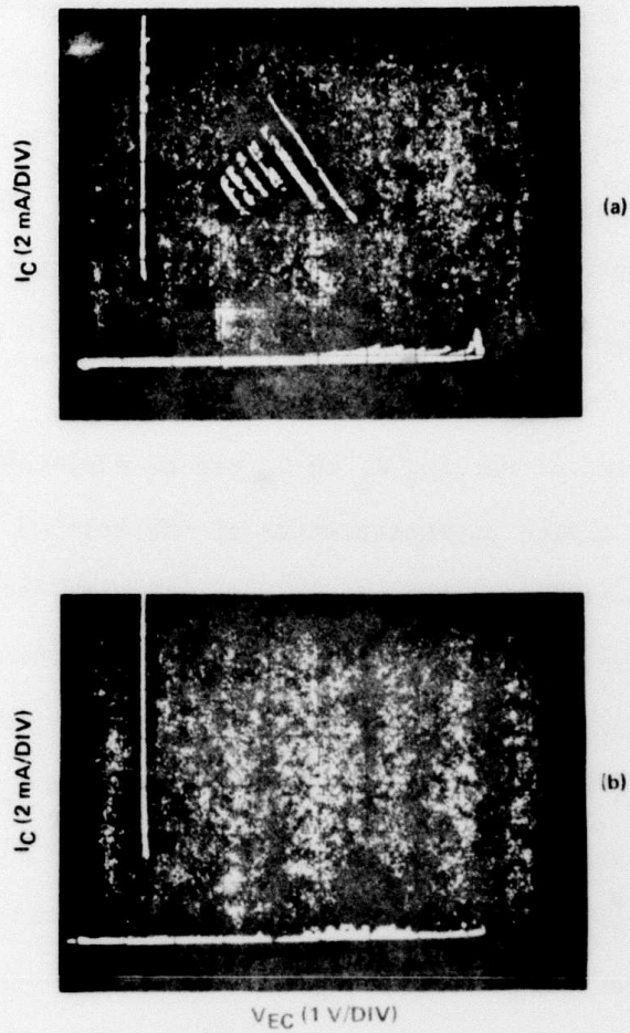
78-46 FIG. 7 Current voltage characteristics of type "A" M-SiO 2 N x -p-n + device. Note differential negative resistance characteristics only when R_L = 500 \Omega . (a) R_L = 500 \Omega . (b) R_L = 120 \Omega .
