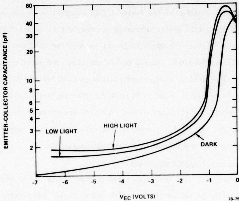
FIG. 27 Capacitance-voltage characteristics of Mo-SiO 2 -n-p + ICS device. Capacitance is measured across emitter and collector terminals with base terminal open.
