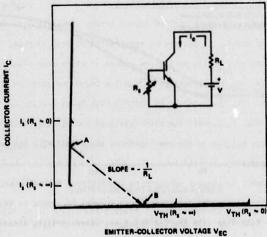
FIG. 5 I-V characteristics of grounded-emitter ICS device for large and small values of base shunt resistance R_S . Transition from point A to point B is possible by only lowering R_S (without changing V or R_L ).
