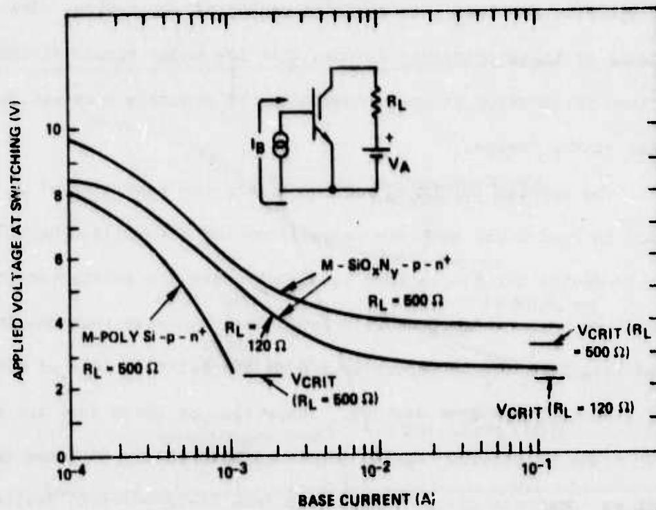
FIG. 5 Voltage applied to device and series load resistance at switching as a function of applied base current.
