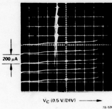
FIG. 11 I-V characteristics of device in row of five devices with 3 mA applied to base row. Offset curves are for 0, 1, 2, 3 and 4 other devices in low impedance state. (Top trace is for 0; bottom trace for 4 low impedance state devices.)
