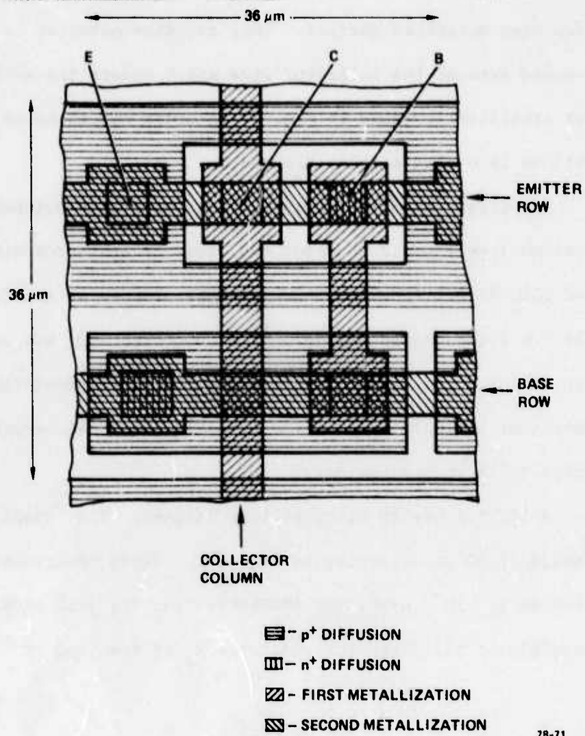
FIG. 23 Layout of proposed small area ICS memory cell.
