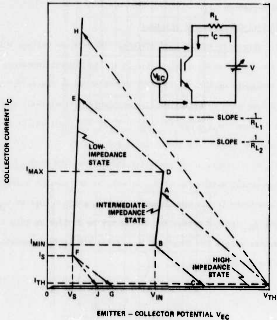
FIG. 4 Definition of critical currents and voltages of ICS diode having three stable impedance states. Load lines show possible transitions between states for unilluminated diode. Note that with a low value of collector load resistance, the intermediate state may not be accessible.
