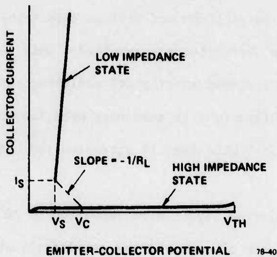
FIG. 2 Current voltage characteristics of ICS and definition of critical currents and voltages.
