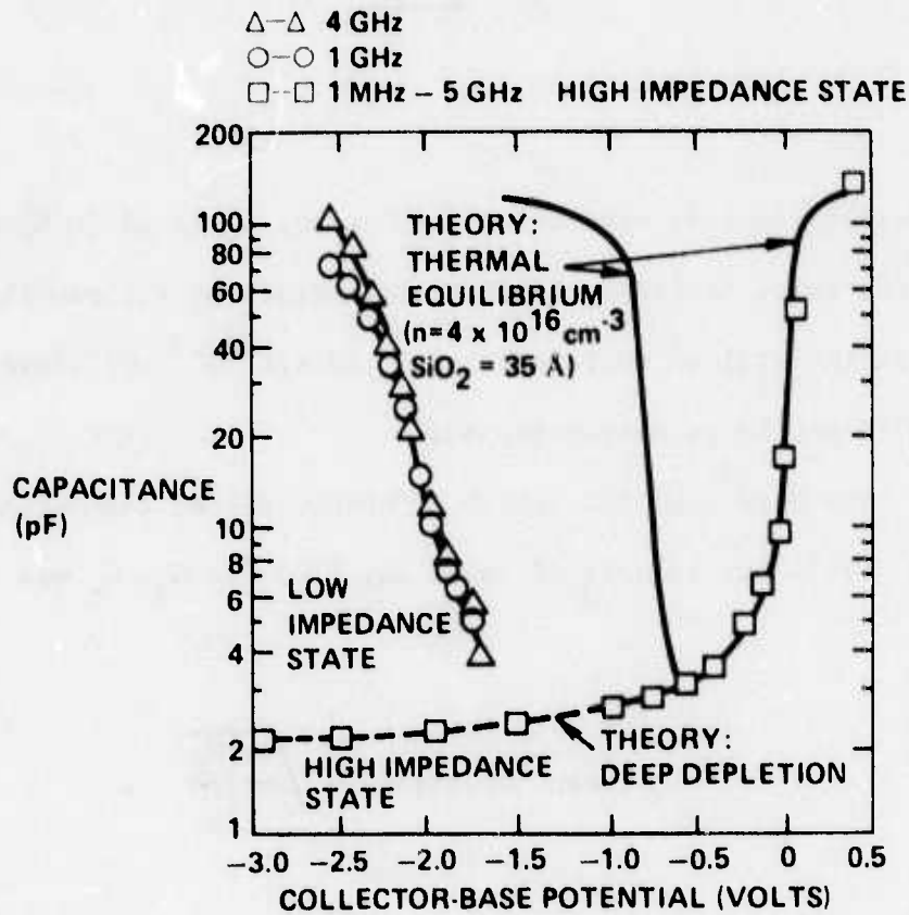
FIG. 34 C-V characteristics of Mo-SiO 2 -n-p + device. Microwave frequency measurements made between emitter and collector and corrected by emitter junction capacitance and voltage drop.
