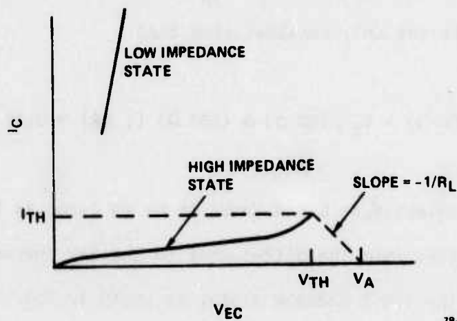
FIG. 8 I-V characteristics of high impedance state illustrating relation between threshold voltage V_{TH} and applied voltage V_A at switching for device with I-V characteristics as in Fig. 7b.
