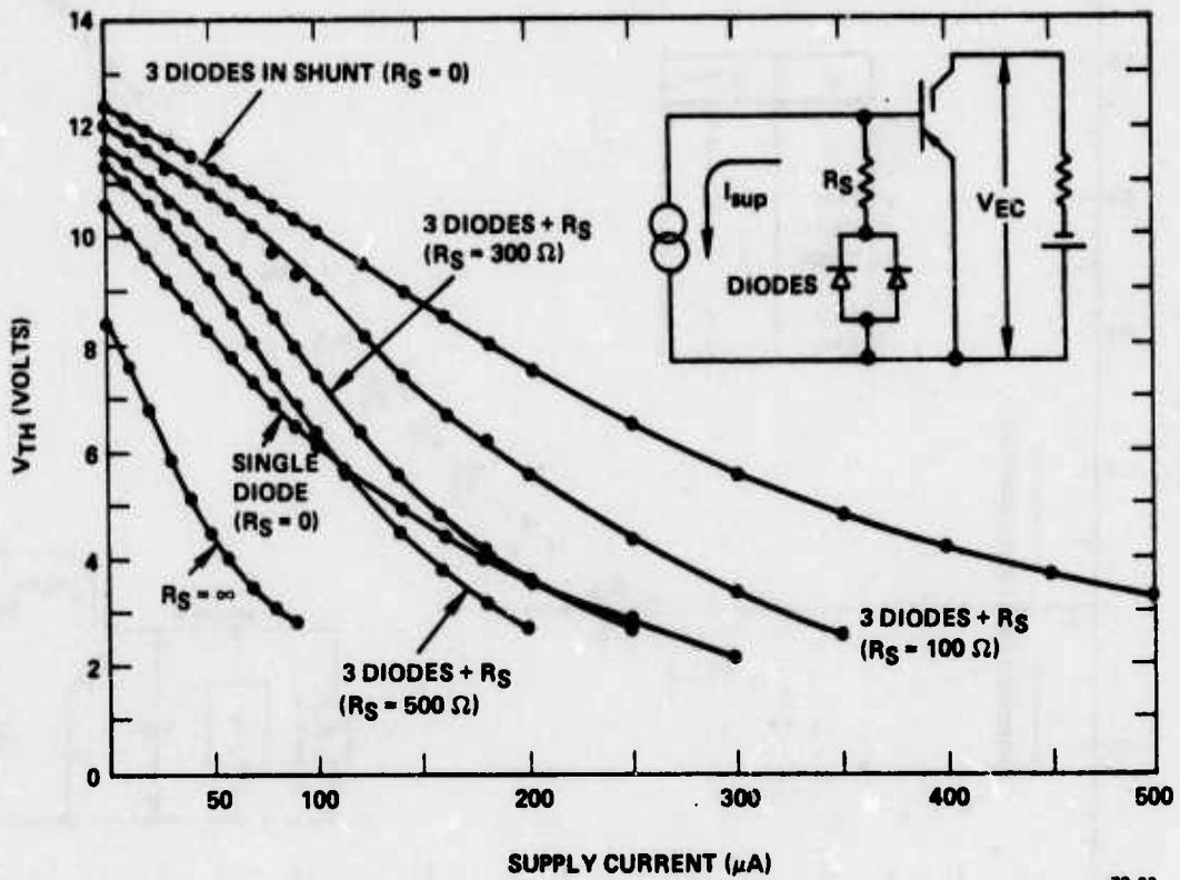
FIG. 15 Threshold voltage V_{TH} as a function of current drawn from base terminal when emitter-base terminals are shunted by various external impedances.
