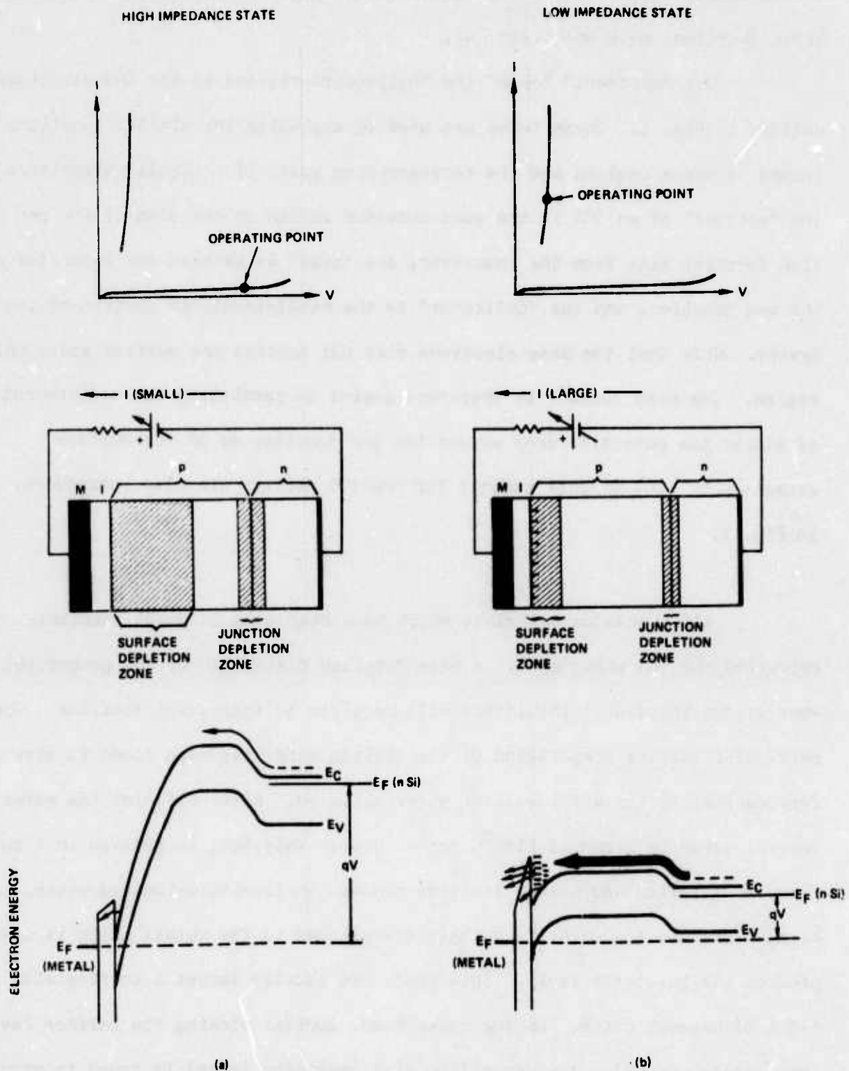
FIG 2 Bistable current-voltage characteristics, relative widths of surface and junction depletion zones and energy band diagram of M-I-p-n device. E_F , E_C and E_V denote Fermi level, conduction band edge and valence band edge, respectively. (a) High impedance state. (b) Low impedance state.
