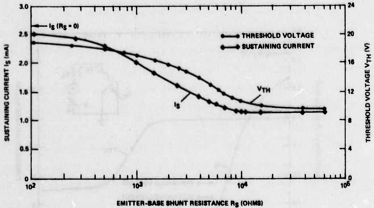
FIG. 4 Variation of sustaining current I_S and threshold voltage V_{TH} of a metal-SiO 2 -N x -y-p-n + device as a function of emitter-base shunt resistance R_S .
