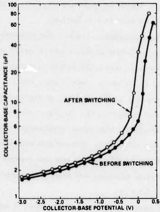
FIG. 5 Collector-base capacitance of a metal-SiO 2 -n-p + device as a function of applied potential.
