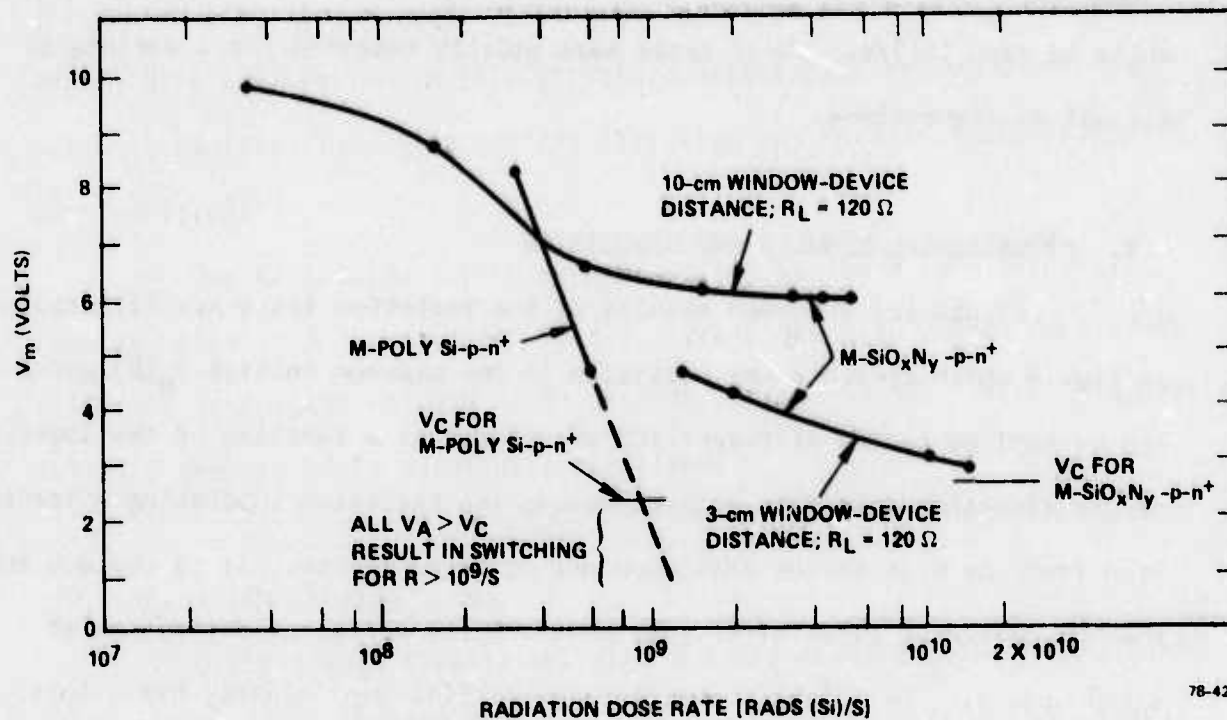
FIG. 4 Maximum voltage V_M which can be applied to devices and load resistor which permits device to remain in high impedance state as a function of applied radiation dose rate for M-polysilicon-p-n + device and type "A" M-SiO x N y -p-n + device.
