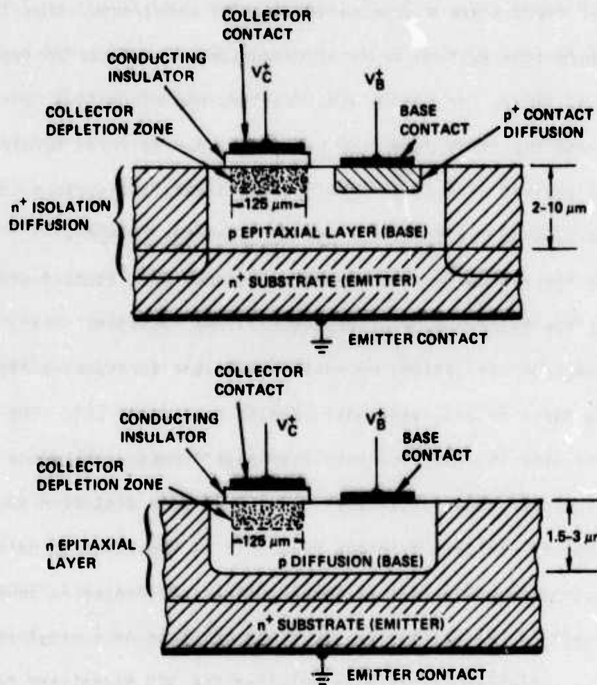
FIG. 1 Cross sectional views of two typical three terminal ICS structures illustrated for M/I/p/n device.
