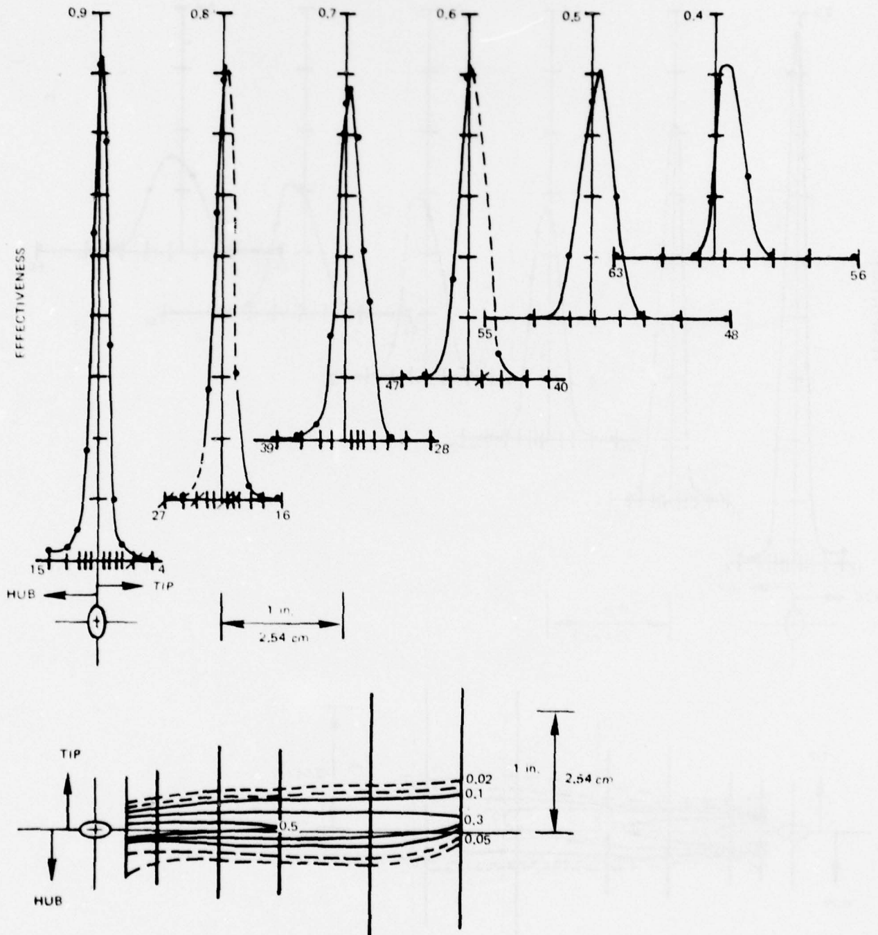
Figure 16. Suction Surface Film Cooling, M = 0.5, R = 1.0
