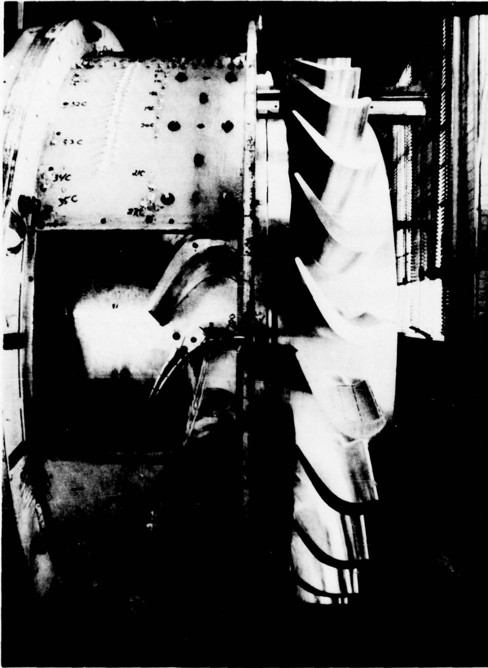
Figure 1. Large Scale Rotating Rig 1-1/2 Stage Turbine Configuration
