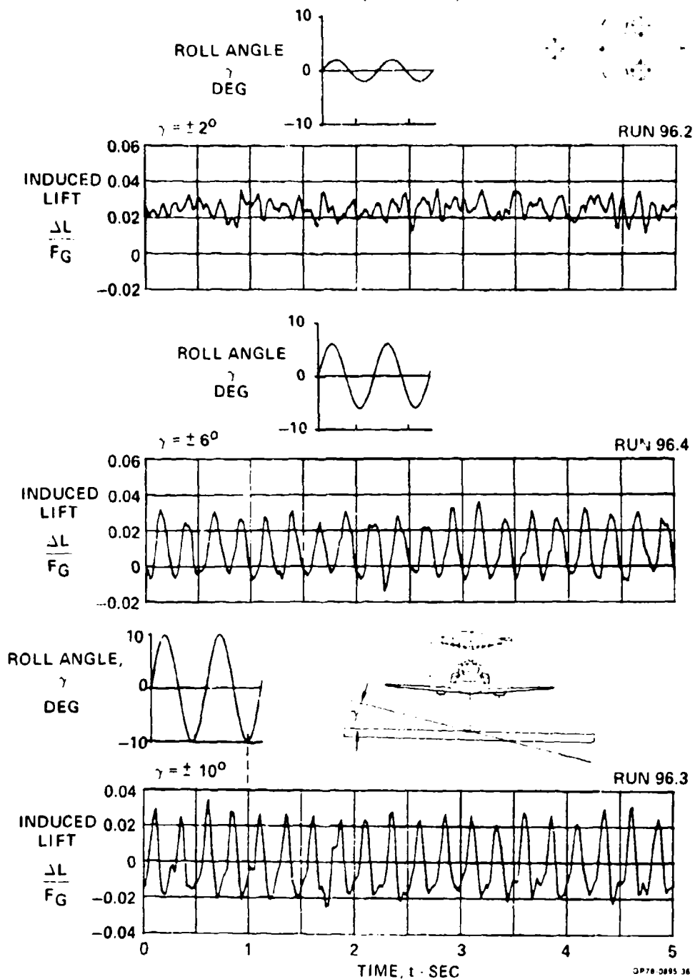
FIGURE 5-36 SUBSONIC V/STOL INDUCED LIFT FOR ROLLING DECK
