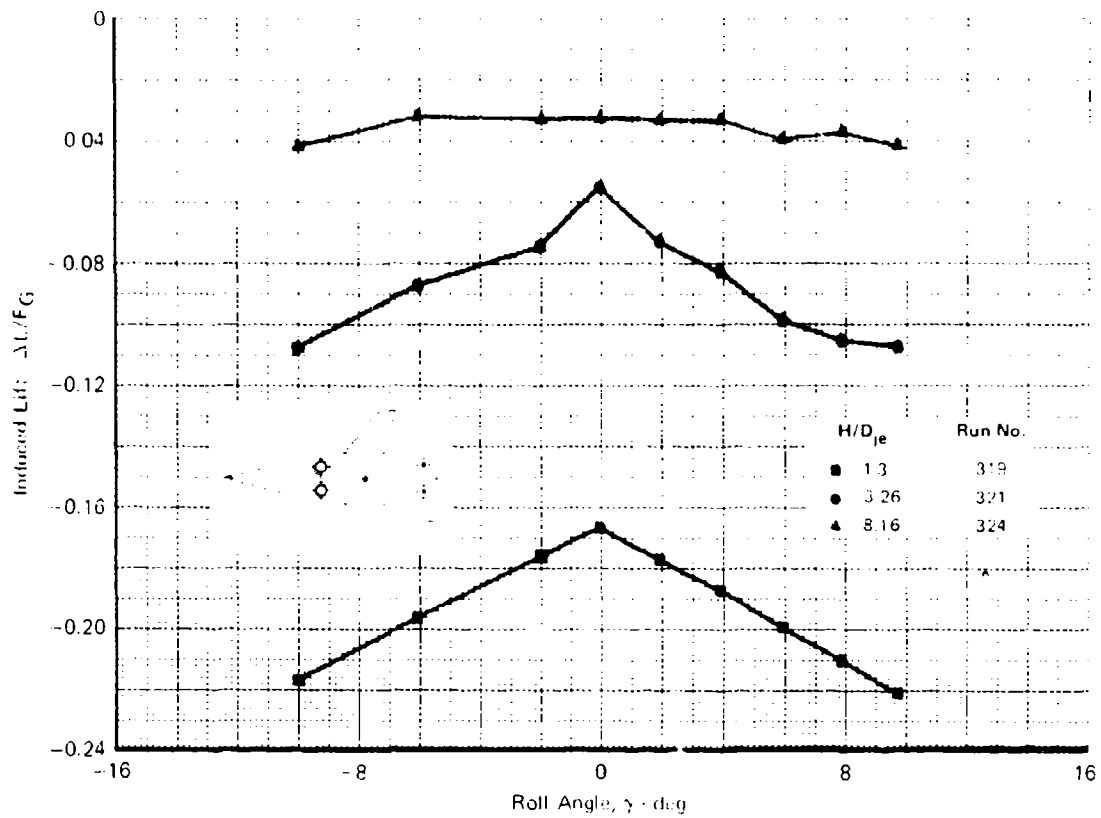
FIGURE 5-27 4 JET SUPERSONIC V/STOL STATIC ROLL EFFECTS
