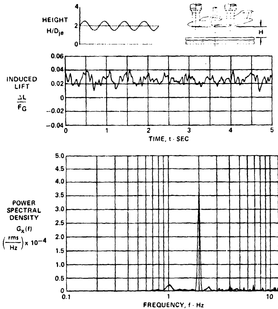
FIGURE 6-52 SUBSONIC V/STOL INDUCED LIFT PSD RESPONSE WITH AMPLITUDE VARIATIONS
