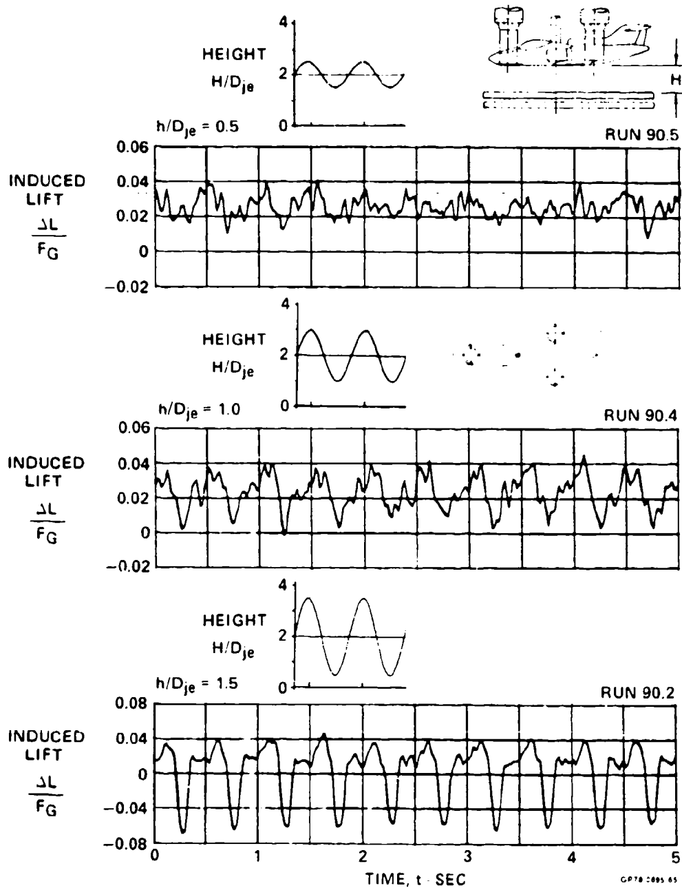
FIGURE 5-35 SUBSONIC V-STOL HEAVE AMPLITUDE EFFECTS
