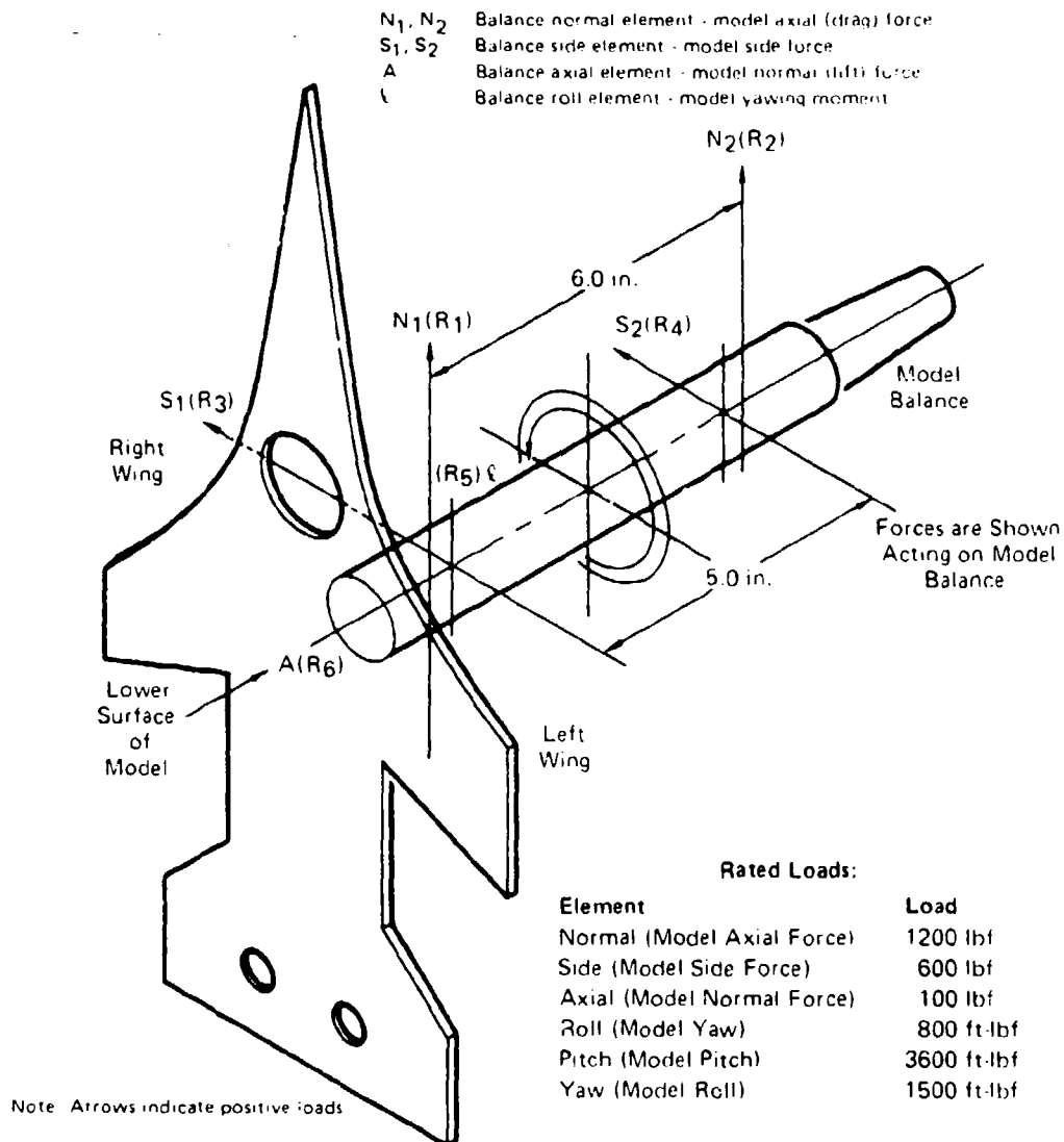
b) Model Balance Installation
