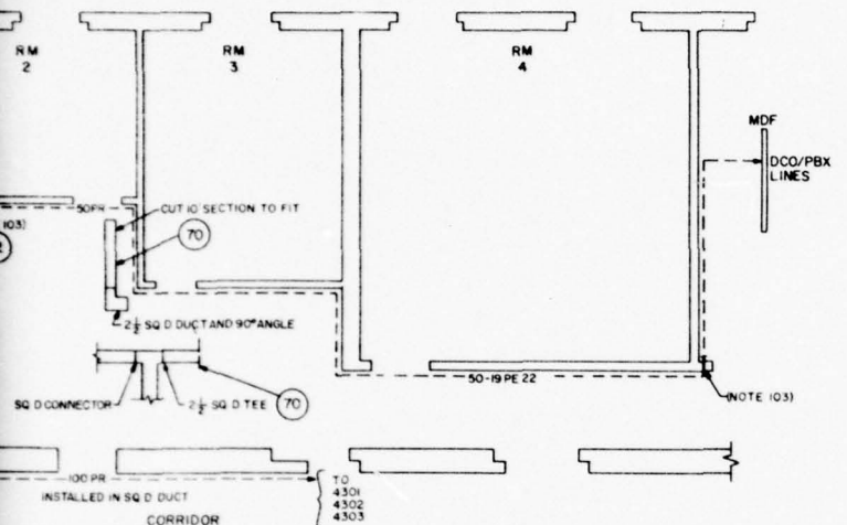
DETAIL A SUPPORT REQUIREMENTS
