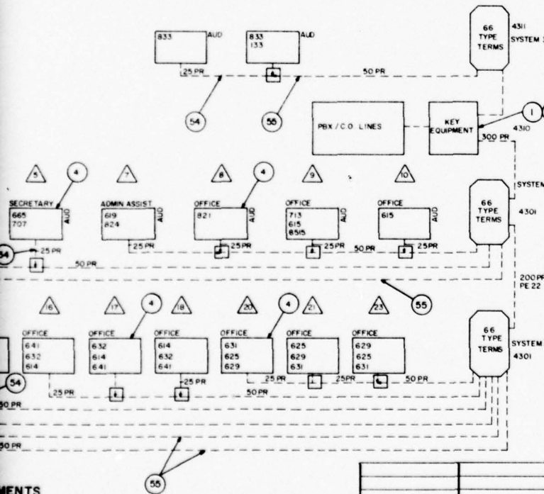
DETAIL A SUPPORT REQUIREMENTS
