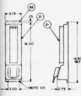
CONNECTORIZED ONE-EIGHTH BLUE FIELD BACK PANEL
