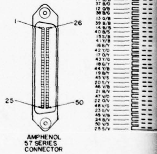
TYPICAL BLOCK AND CONNECTOR
