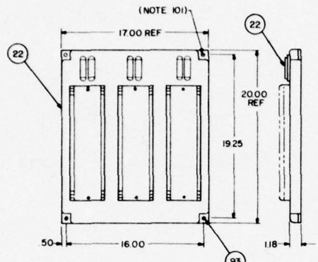
CONNECTORIZED FULL RED FIELD BACK PANEL
