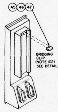
TYPICAL BLOCK AND CONNECTOR WIRING DIAGRAMS
