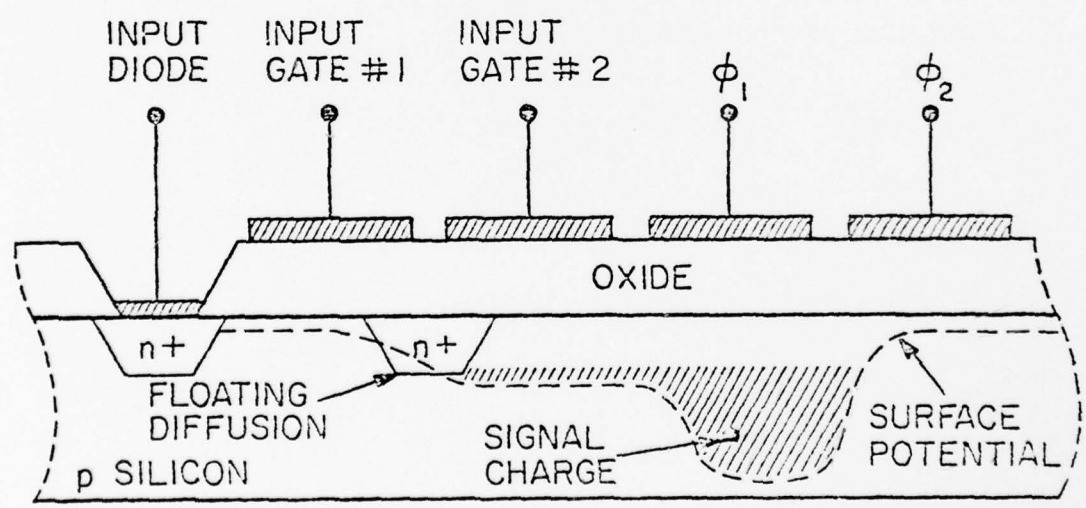
Figure 3 Floating Diffusion Input
