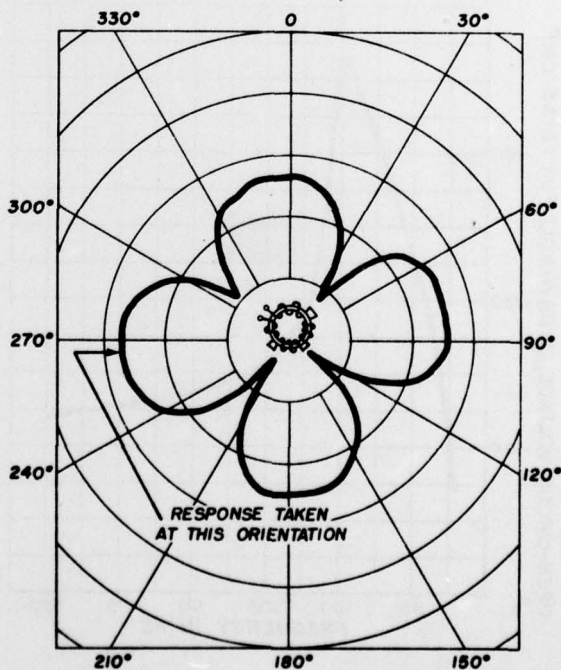
Fig. 6B - Receiving Directivity Pattern Taken at 53.8 kc and Schematic Drawing of Winding
