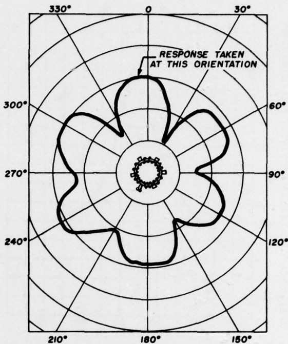
Fig. 7B - Receiving Directivity Pattern Taken at 76 KC and Schematic Drawing of Winding
