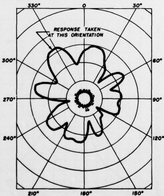
Fig. 8B - Receiving Directivity Pattern Taken at 99.8 KC and Schematic Drawing of Winding
