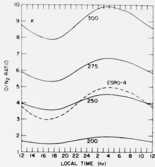
Figure 6. The O/N_2 Ratio at Thermospheric Altitudes and Compared to the Measurements of Kohnlein et al 9
