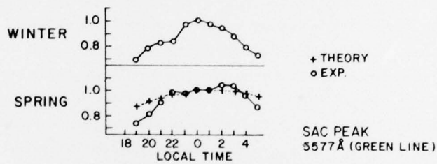
Figure 7. The Nighttime Variation of the Integral of the Atomic Oxygen Concentration (dashed line) Where the Limits of Integration Are From 85 to 120 km. The ground based green line ( 5577 \text{ \AA} ) measurements (solid line) at Sac peak (Brenton and Silverman) 10 are compared to O column density ( \int O^3 dz ) with good agreement
