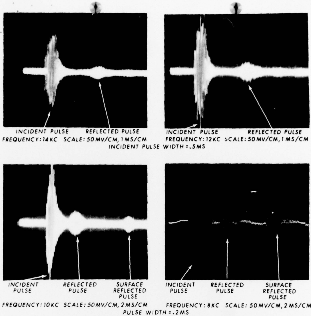
Fig. 30 - Reflection Measurements (090° Bearing)
