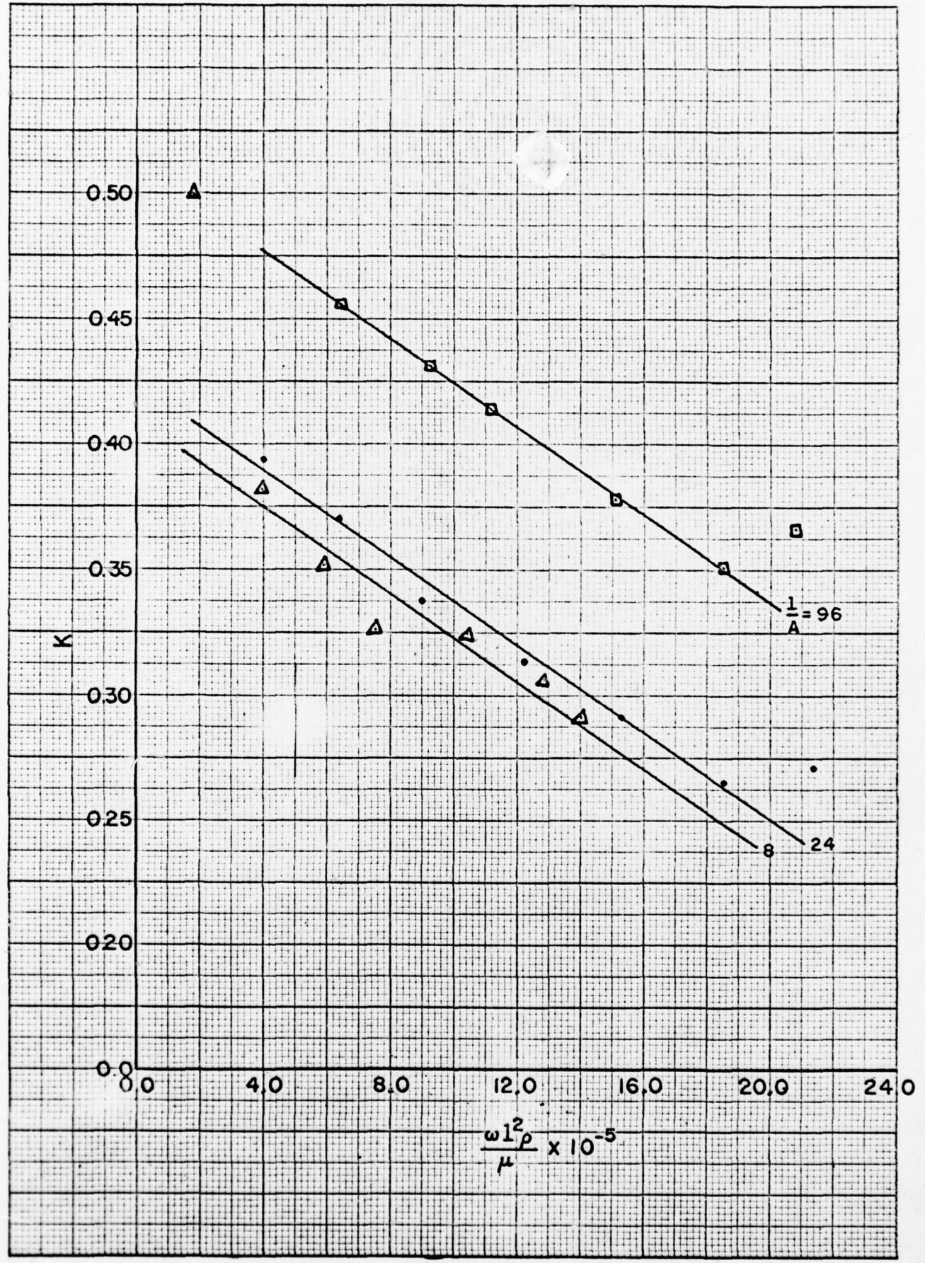
FIGURE 15 Hydrodynamic Mass Factor for the Winged Body
