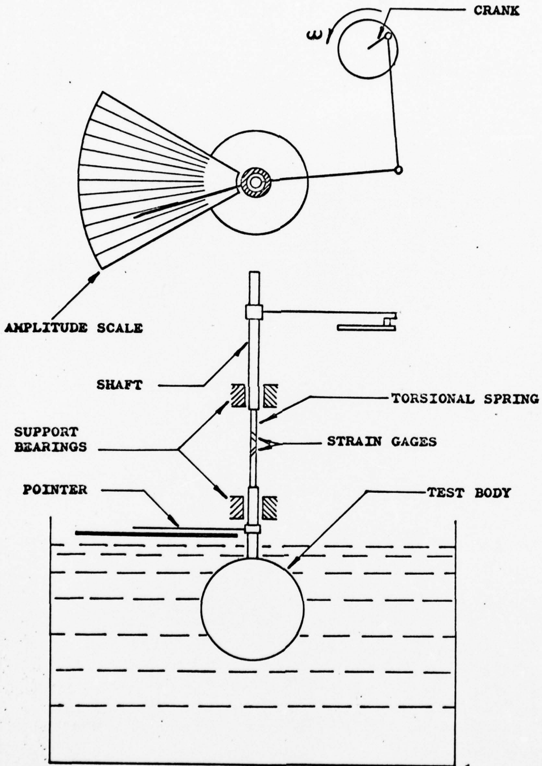
FIGURE 6 SCHEMATIC OF HYDRODYNAMIC MASS MOMENT OF INERTIA APPARATUS
