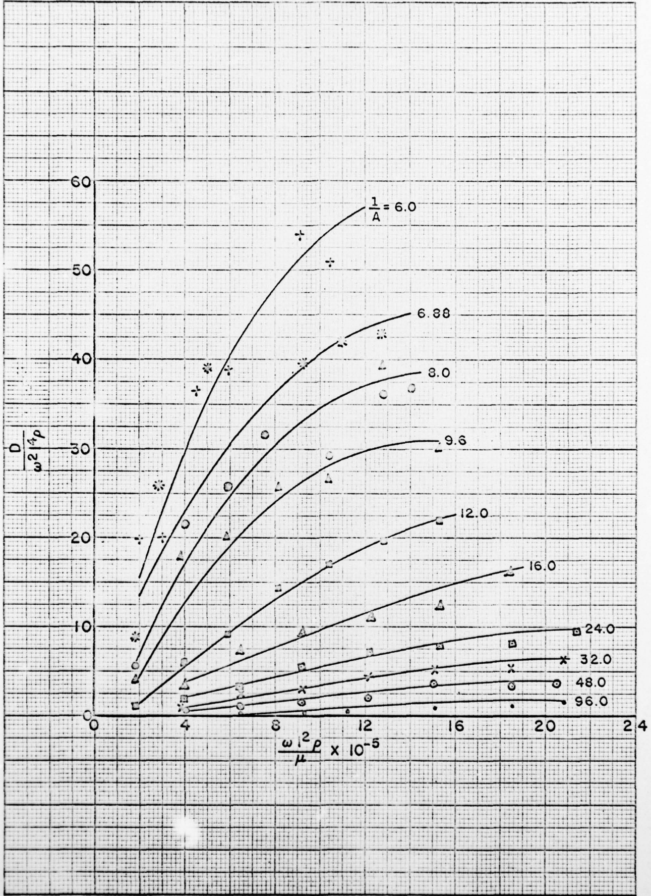
FIGURE 22 Damping for Winged Body Perpendicular to Direction of Towing
