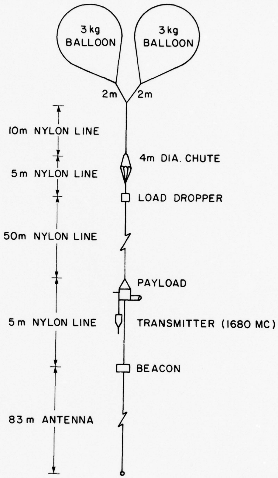
Figure 5. The load train configuration.
