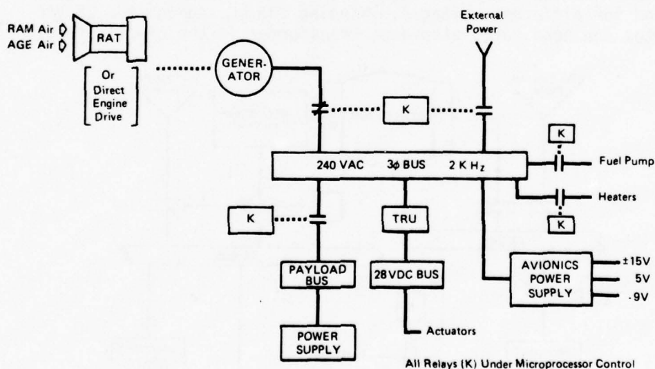
Figure 26. VSVF System
