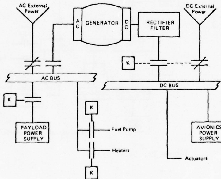
Figure 27. AC/DC System
