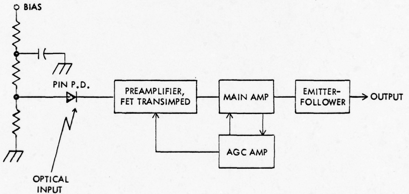
Figure 7.2.1.6-2. Equalized Impedance-Matched Optoelectronic Receiver
