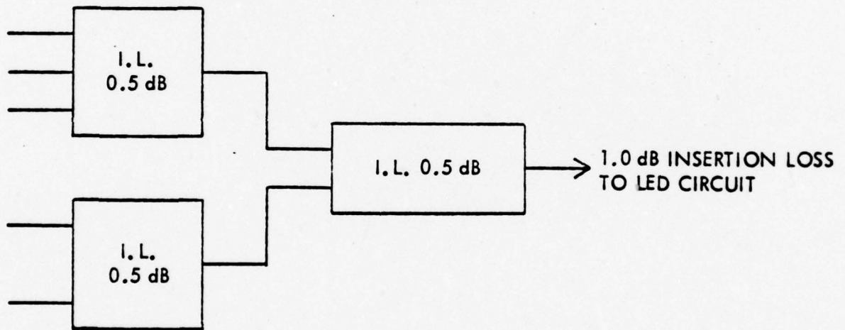
(B) 5 CHANNEL COMBINER (ONE PER SYSTEM)
