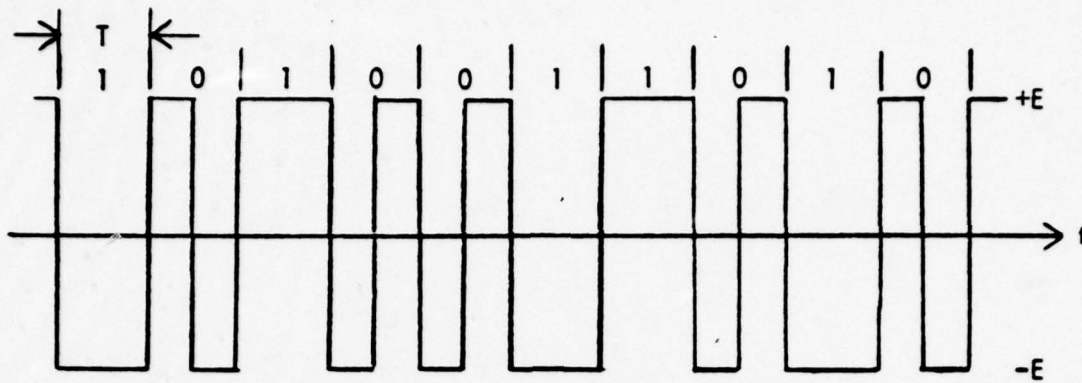
Figure 3.1-1. An Idealized Conditioned Diphase Waveform
