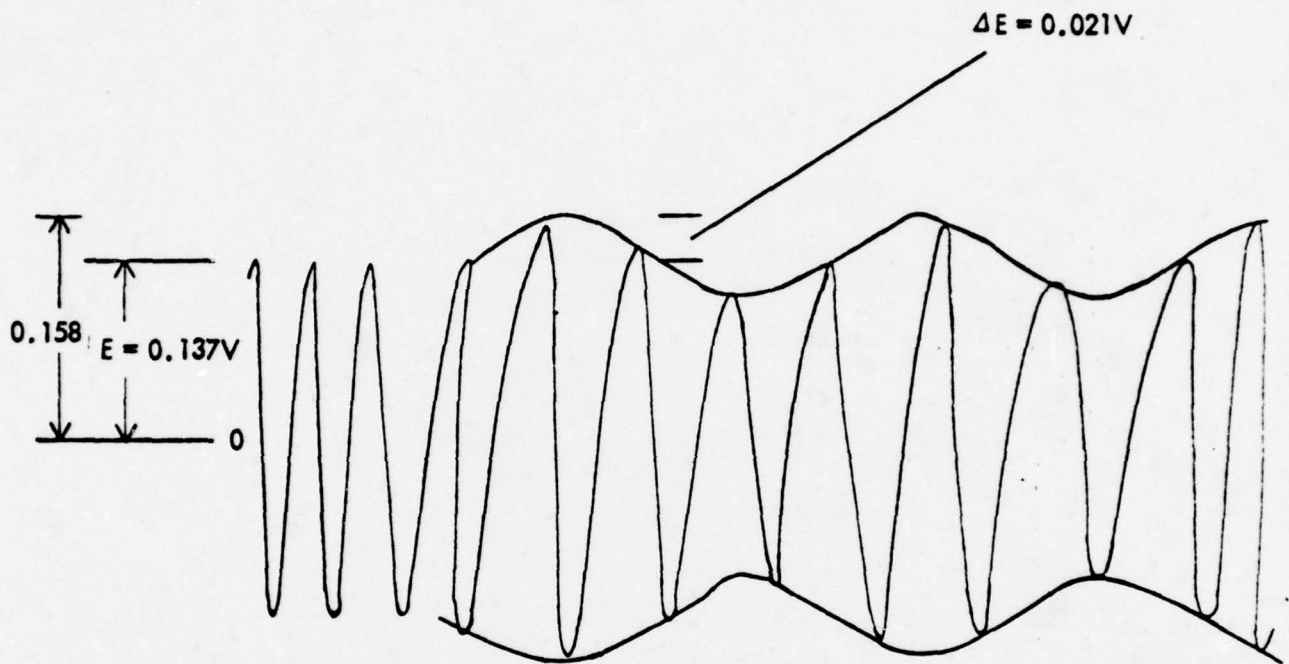
Figure 7.2.1.2.1. Single Tone Amplitude Modulated Waveform
