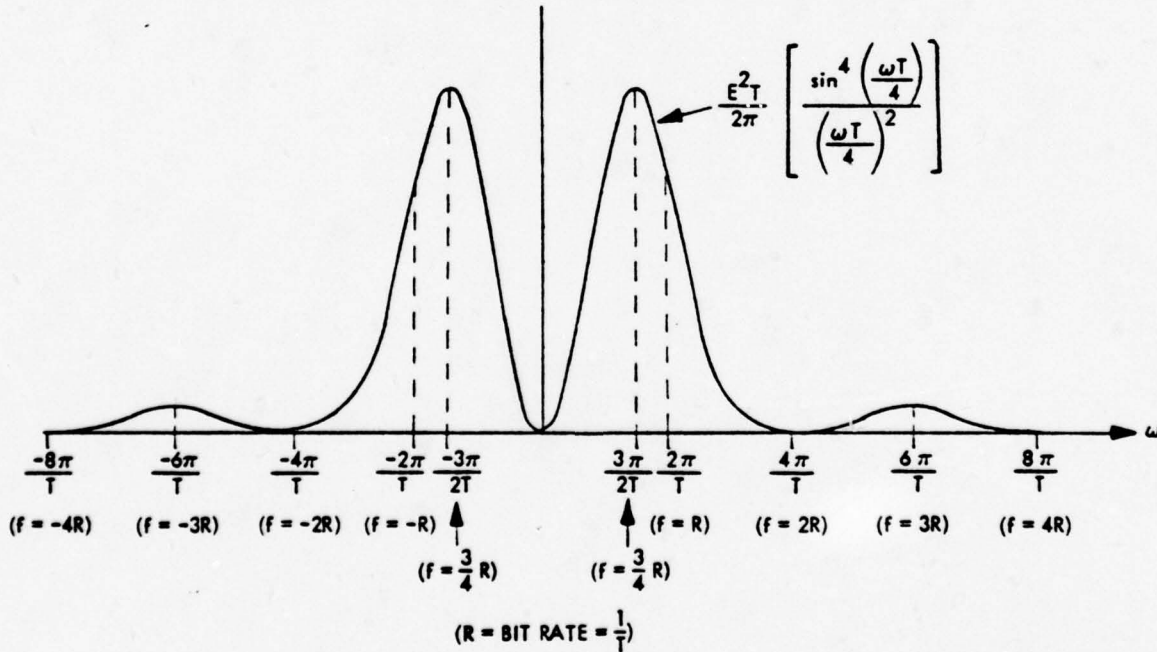
Figure 3.1-2. Power Spectrum for Conditioned Diphase PCM [1]
