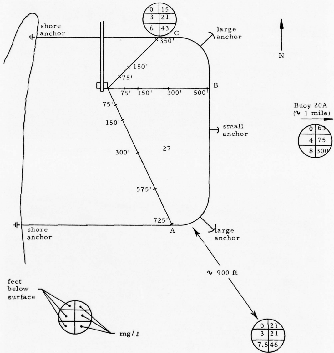
Figure 43. Anchor configuration and background suspended solids levels at site 3
