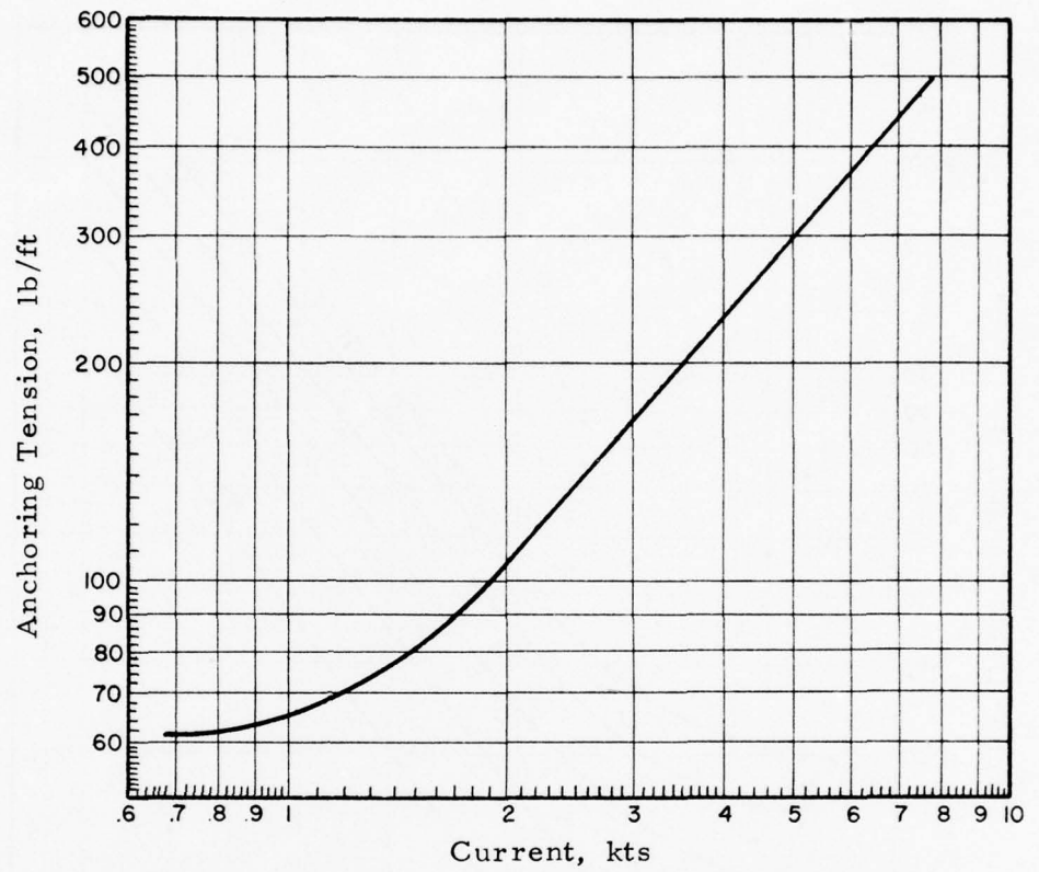
Figure 30. Anchoring loads for a totally submerged 5-ft silt curtain with bottom tension member 60 lb/ft net buoyancy
