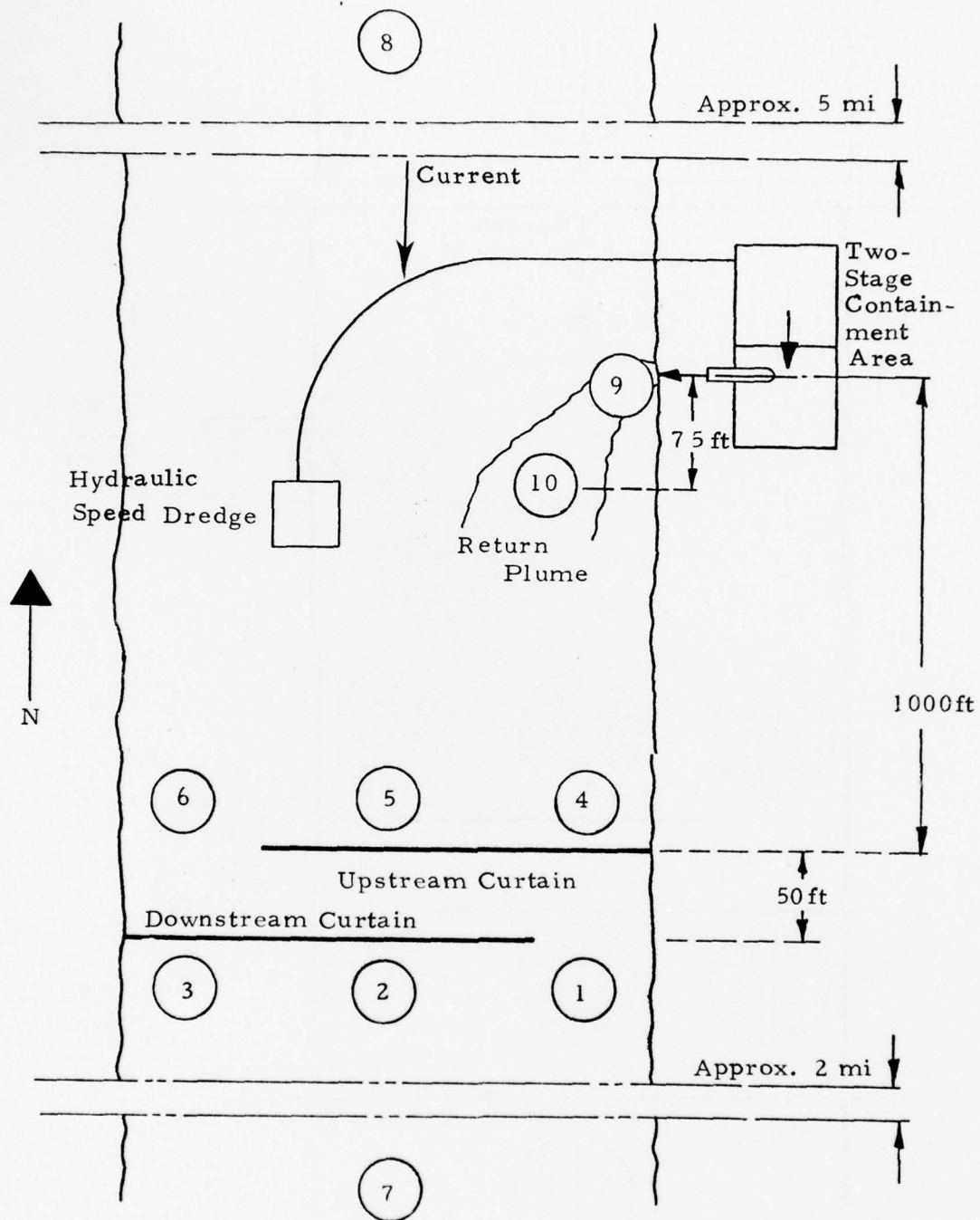
Figure 35. Schematic showing sampling stations at site 1
