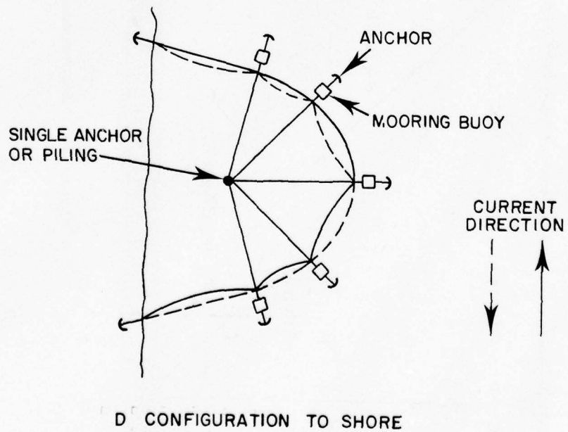
Figure 75. Recommended anchoring configurations 170
