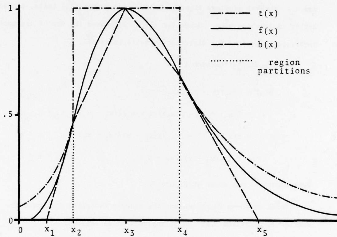
Figure A. Algorithm G2PE for \alpha = 5 .
