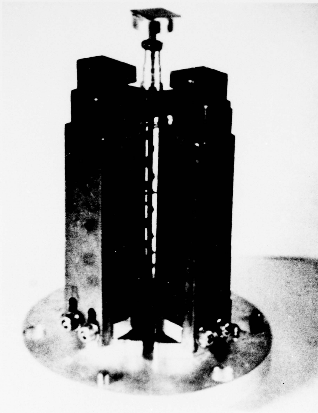
Figure 3 - The cryogenic mechanical scanner
