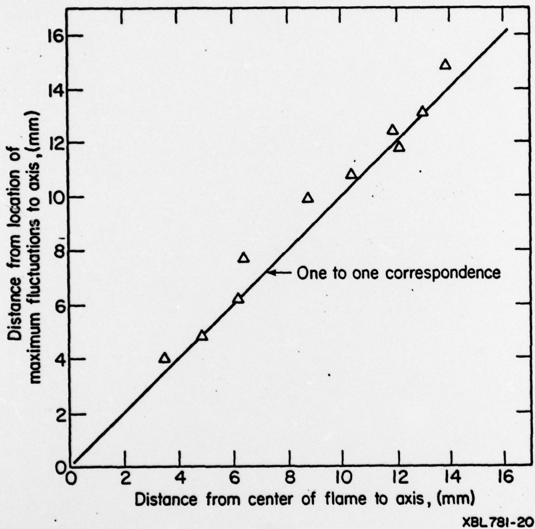
FIGURE 14. Correlation of Flame Location with Location of Maximum RMS Fluctuation
