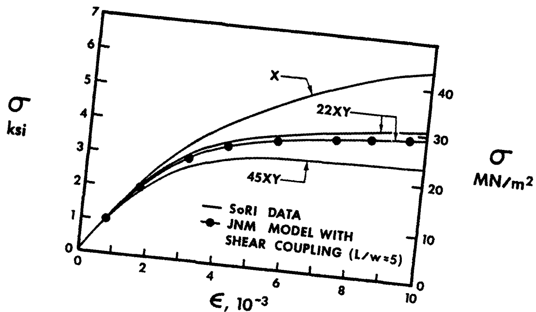
FIGURE 3.40 TENSION STRESS-STRAIN BEHAVIOR IN xy-PLANE
