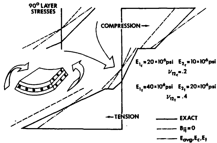
FIGURE 2.21 STRESS DISTRIBUTION IN A 3-LAYER "SYMMETRIC" LAMINATE WITH MODERATE ORTHOTROPY AND HIGH E_t/E_c
