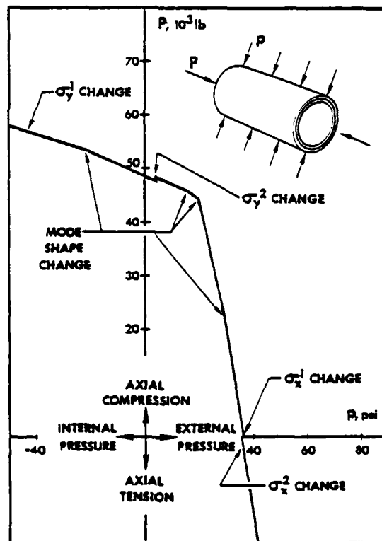
FIGURE 2.22 BUCKLING OF A TWO-LAYERED BORON-EPOXY SHELL
