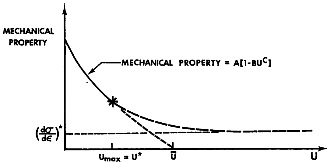
FIGURE 3.13 MECHANICAL PROPERTY VERSUS STRAIN ENERGY CURVE EXTRAPOLATION
