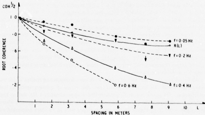
Fig. 9. Spatial correlation R(L) derived from maximum cross correlations between pairs of sensors, and the contribution from each frequency band (coherence). In-line array 300 m, 1969 July 30 at 1116, with humidity sensors.
