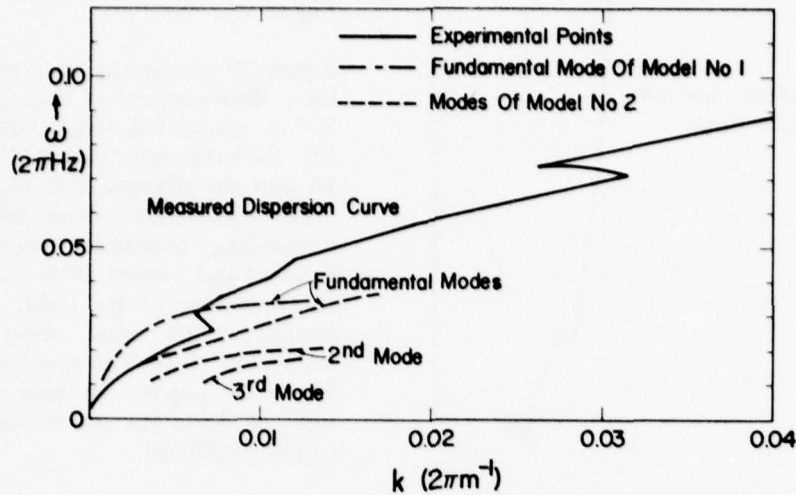
Figure 8 Intrinsic frequency as a function of the wavenumber Only the fundamental mode is shown for model no.1.
