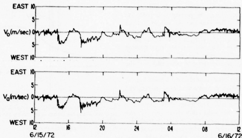
FIG. 4. A comparison of the average wind speed ( V_o ) measured optically, with the average of the readings of six Gill propeller anemometers ( V_a ) uniformly spaced along the optical path. Both the anemometers and the optical system measure the component of wind that is horizontal and at right angles to the path. The path is 300 m long, oriented north-south, and 3 m above the ground.
