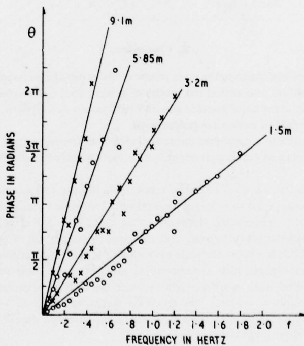
Fig. 11. Phase of cross-spectrum against frequency for various sensor spacings. Data as in Figure 9.
