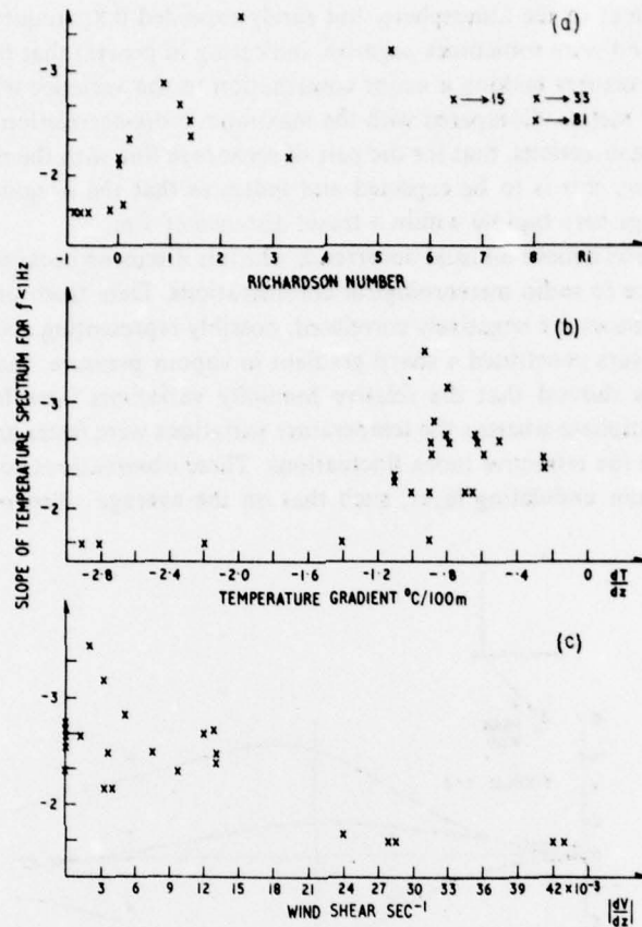
Fig. 5. Variation of slope of temperature spectrum ( f < 1 Hz) with (a) Richardson number, (b) temperature gradient and (c) wind shear.
