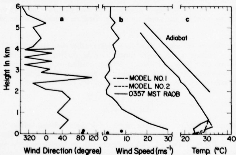
Figure 9 Radiosonde at 0457 MDT The circles shown are the wind and temperature data from the tower at the time of the wave event. The various atmospheric models discussed are shown as dashed curves.
