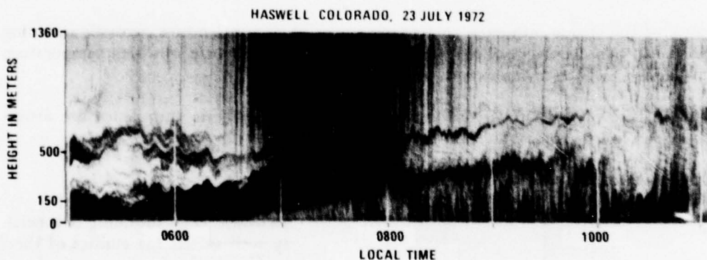
Figure 3.9 Facsimile recording of backscatter acoustic intensity during conditions of nocturnal inversion and breaking up of the same
