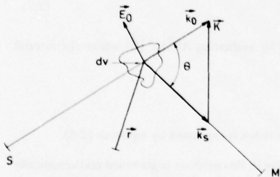
Figure 2.1 Scatter geometry
