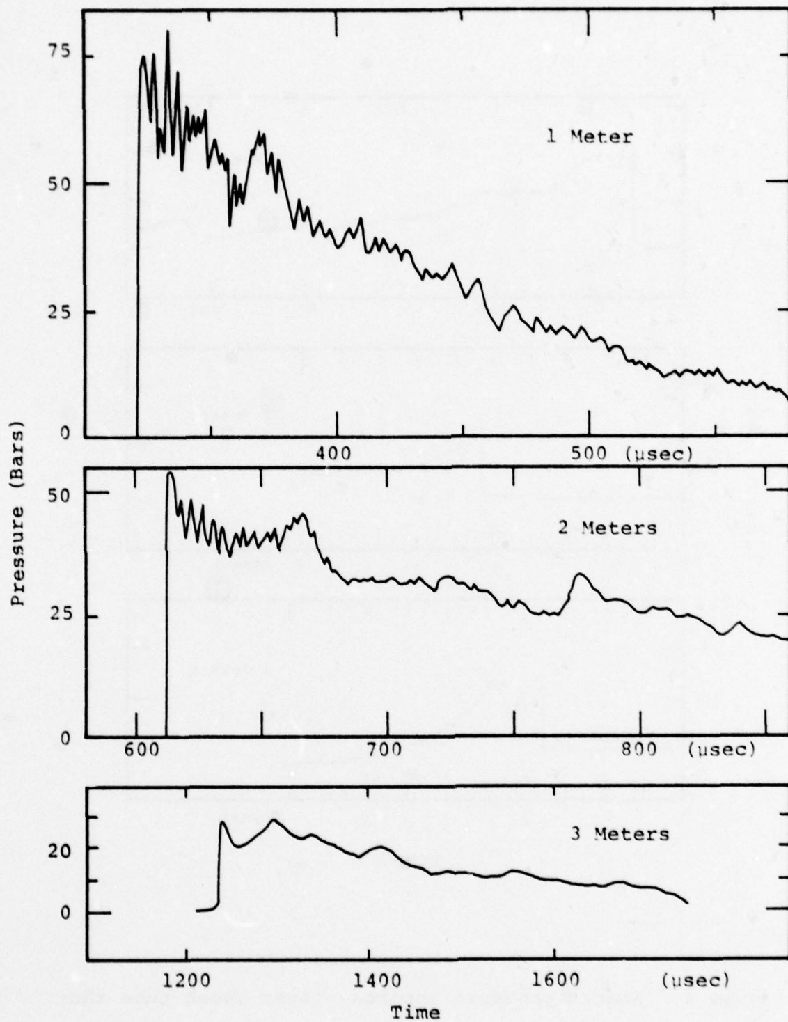
Figure 5. Static pressure records, second shock tube shot.
