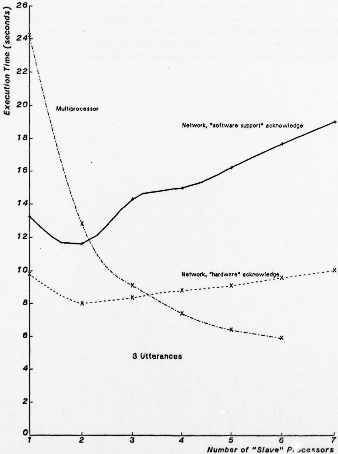
Fig. 4.16: Harpy, Execution Time of Multiprocessor and Network
