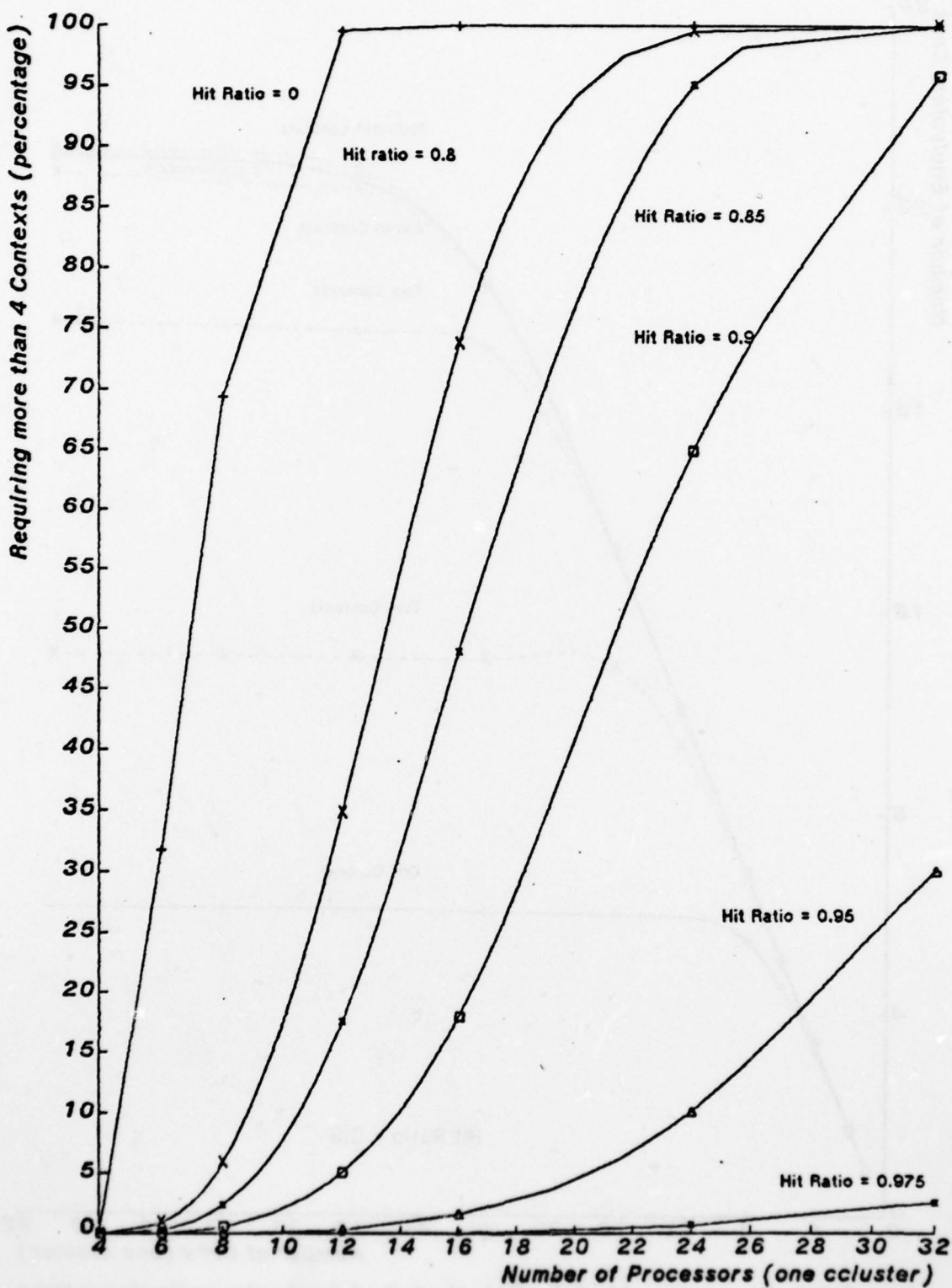
Fig. 3.15: Network Model, Requirement for more than 4 Contexts
