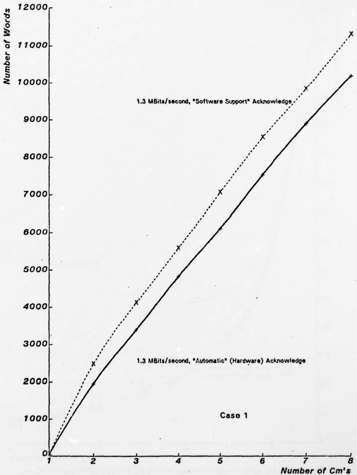
Fig.4.9: Integer Programming, Network, Number of Words Transferred
