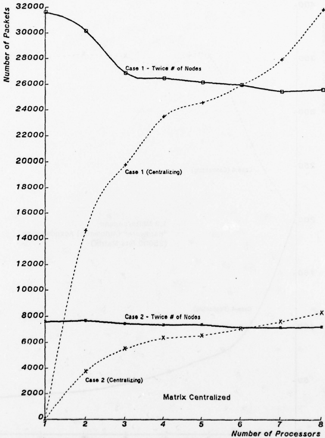
Fig.4.14: Integer Programming, Number of Packets Sent
