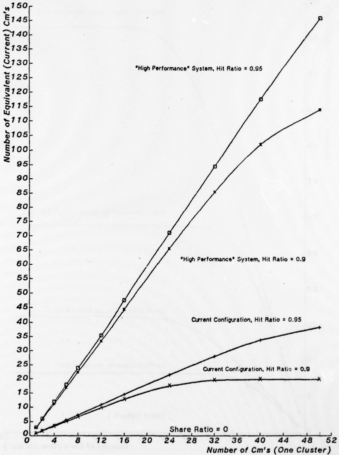
Fig. 3.29: High Performance, No Kbus-Pmap, Fast Pc.-Mem. and Arbit.
