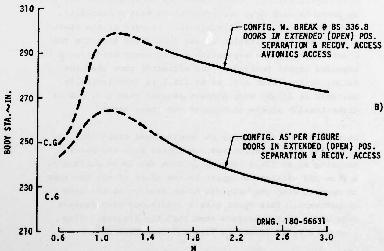
FIGURE 37 STATIC CENTER OF PRESSURE ESTIMATES FOR SEPARABLE FOREBODY OF MODEL 987-230B A) LONGITUDINAL B) DIRECTIONAL
