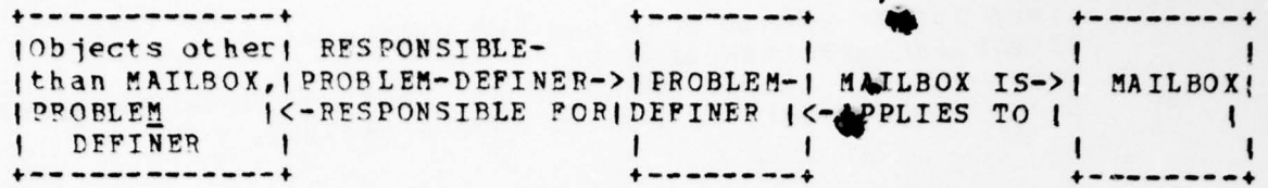
Figure 2.9.1 URL Statements for Describing Project Management
