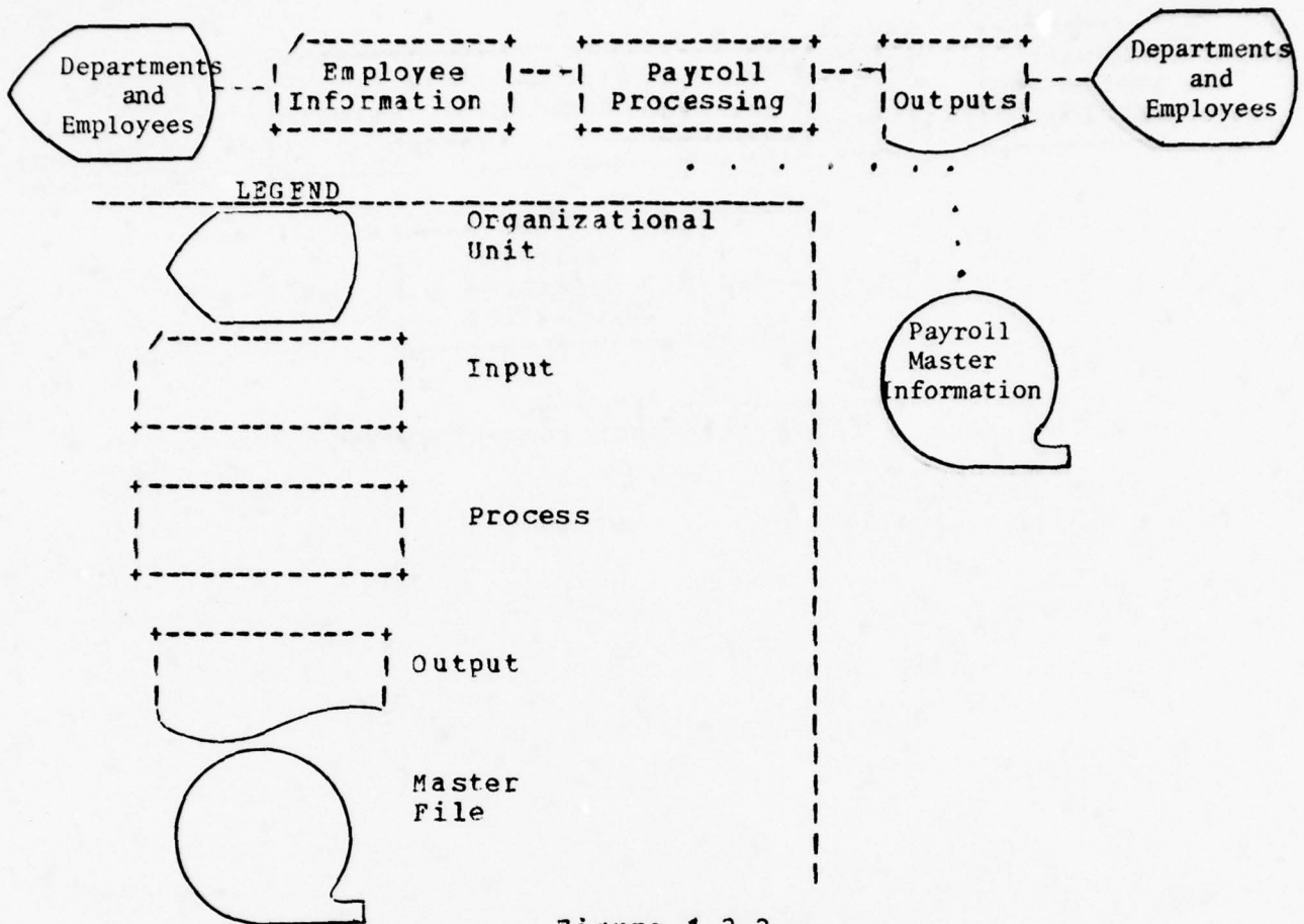
Figure 1.2.2 System Flowchart for PAYSYSTEM Using Standard Flowchart Symbols
