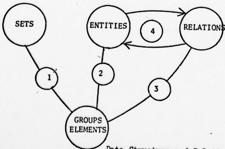
Data Structure and Relationships Figure 2.3.1
