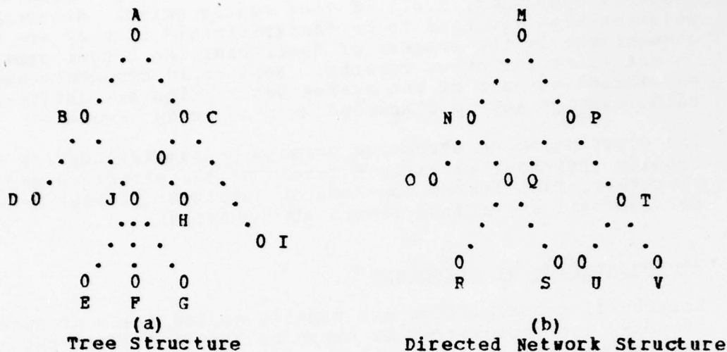
Figure 2.2.1 Tree and Network Structures
