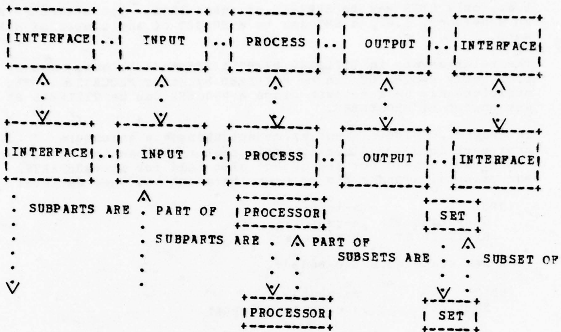
Figure 2.2.2 SOME STRUCTURAL RELATIONSHIPS EXPRESSIBLE IN URL
