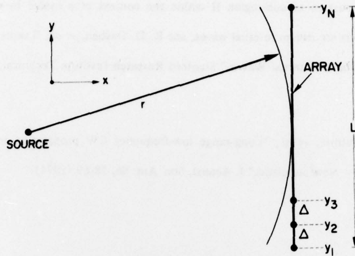
Fig. (1) — Array geometry. The array is of length L and consists of N elements spaced \Delta apart. It is parallel to the y -axis so that the n th array element is located at (x, y_n, z) . It is oriented broadside to the source. The source is a distance r away from the array where r \gg L . The slight variation of the range along the array is ignored in the calculation of the array gain.
