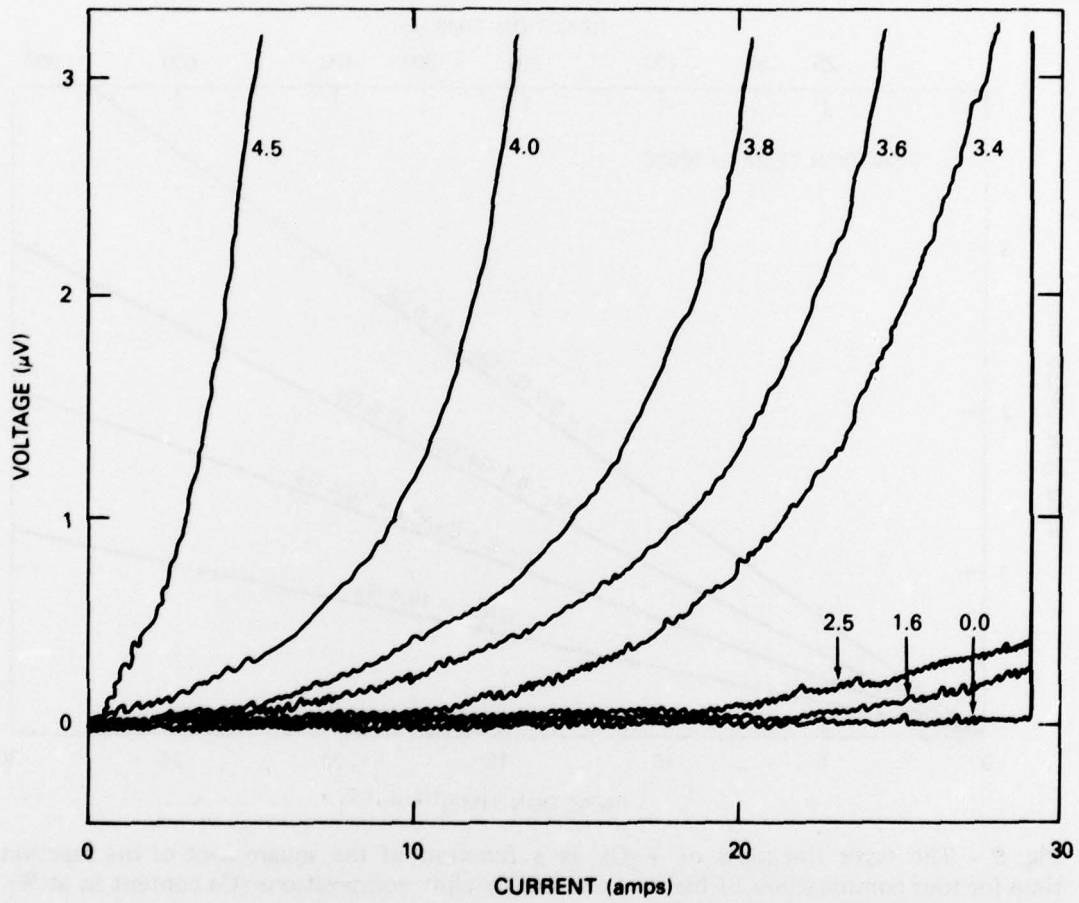
Fig. 8 - Voltage versus current characteristics of a V_3Ga wire at tensile stresses of 0.0 to 4.5 \times 10^8 Pa (0 to 65,250 psi). The magnetic field and temperature were constant: 9T and 4.2K respectively.
