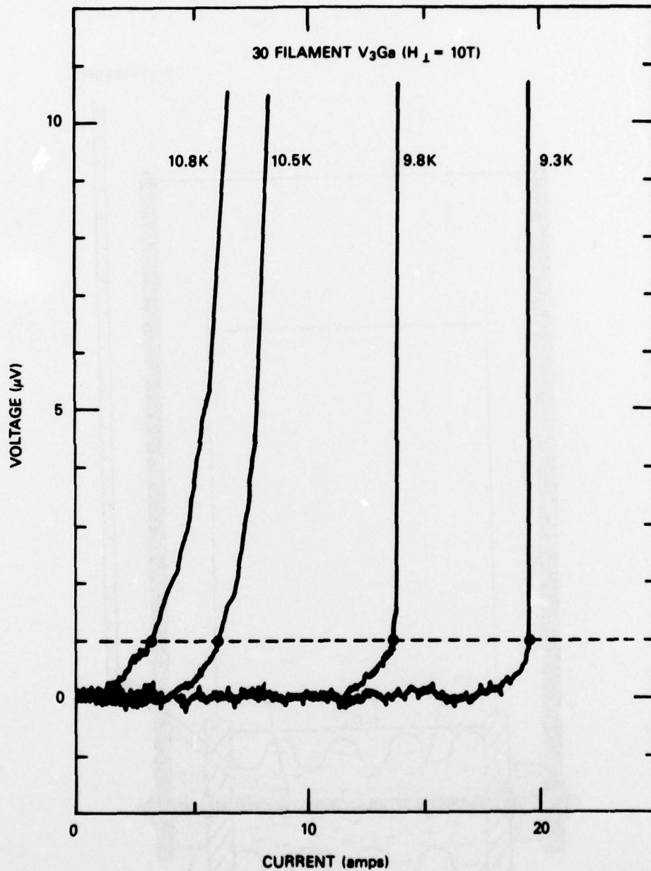
Fig. 6 - Voltage versus current characteristics of a V_3Ga wire at four temperatures in a transverse magnetic field of 10T. The intersections of these traces with the dashed-line at 1 \mu V ( 2 \mu V/cm ) are the I_c 's of the wire at the respective temperatures.
