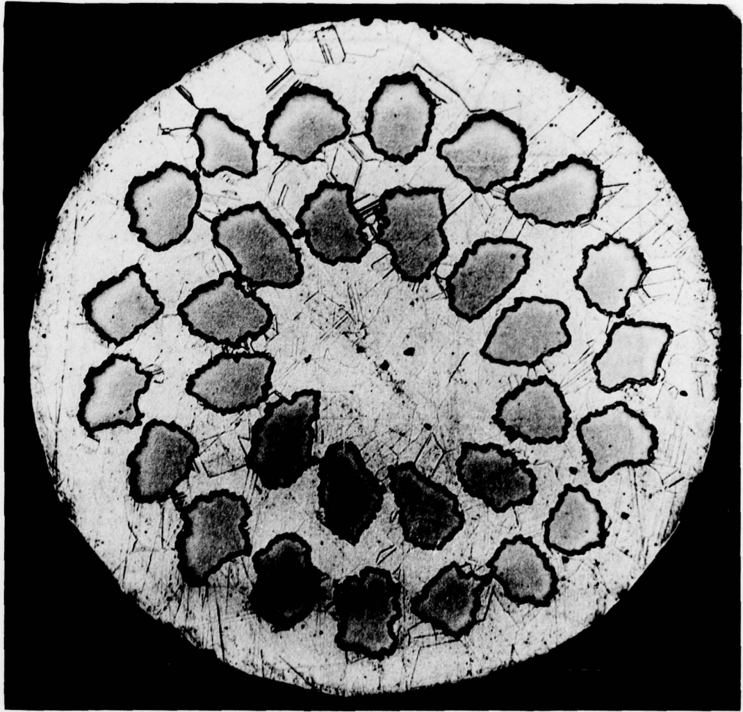
Fig. 4 - Micrograph of the cross-section of a 0.8 mm diameter wire containing 30-filaments of V-8 at % Ga in a Cu-17.5 at % Ga matrix. A 144 hour heat-treatment at 650^\circ has produced the 4\ \mu\text{m} thick layer of V_3Ga on each of the filaments. Marker = 50\ \mu\text{m} .
