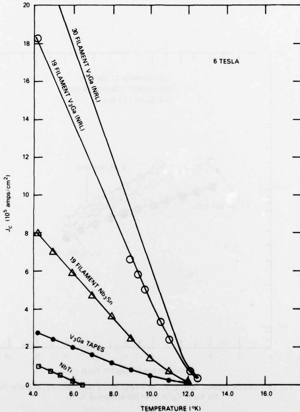
Fig. 11 - Comparisons of the J_c values for two NRL multifilament V_3Ga wires, a BNL experimental Nb_3Sn wire (Ref. 6), commercial tapes from Vacuum Metallurgical Co., Ltd. (Ref. 20), and commercial Nb-Ti wire from Imperial Metal Ind., Ltd. (Ref. 20).
