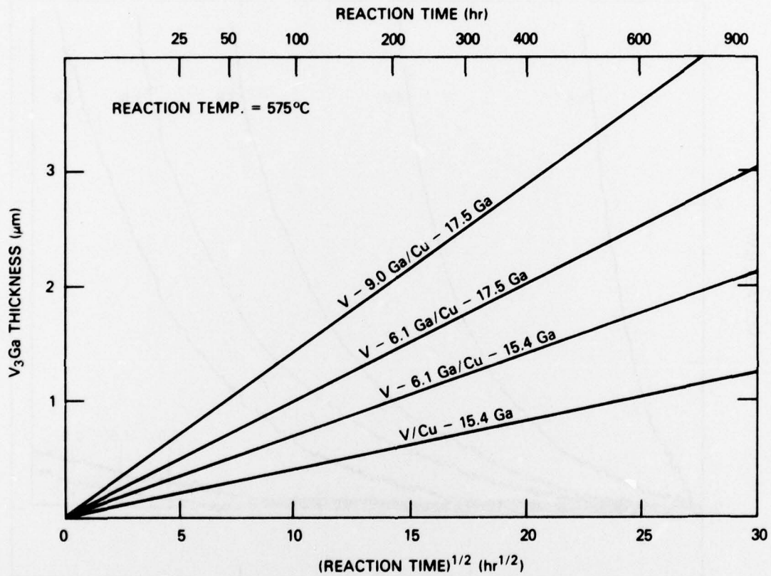
Fig. 9 - The layer thickness of V_3Ga as a function of the square root of the reaction time for four combinations of filament and matrix alloy compositions (Ga content in at %). The reaction temperature is 575°C.
