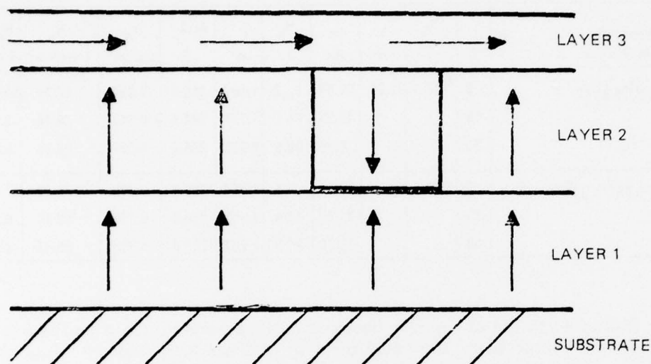
Figure 2. Triple Layer Self-Biased Bubble Domain Structure
