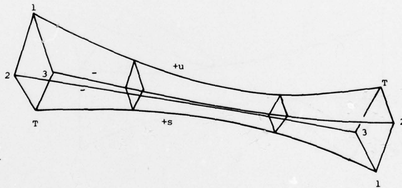
Figure 2.4d 2 : III_1 , \epsilon > 0 , region 1, k odd or even
