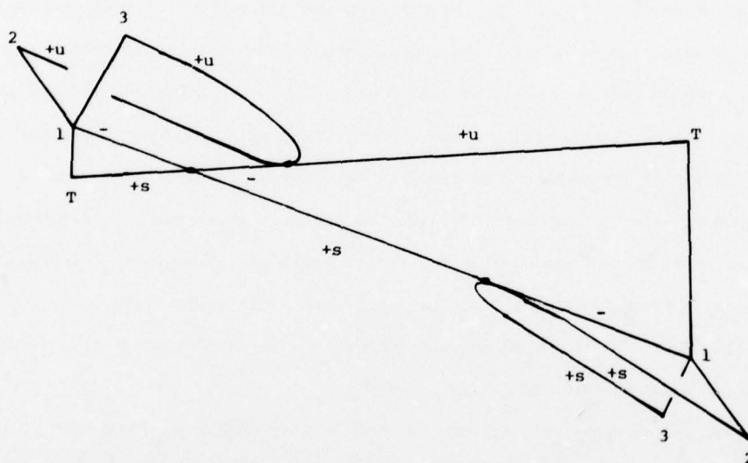
Figure 2.3e 2 : III_2, (-1)^k \delta < 0
