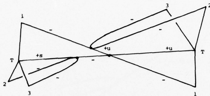
Figure 2.3c 1 : III_0, (-1)^k \delta > 0
