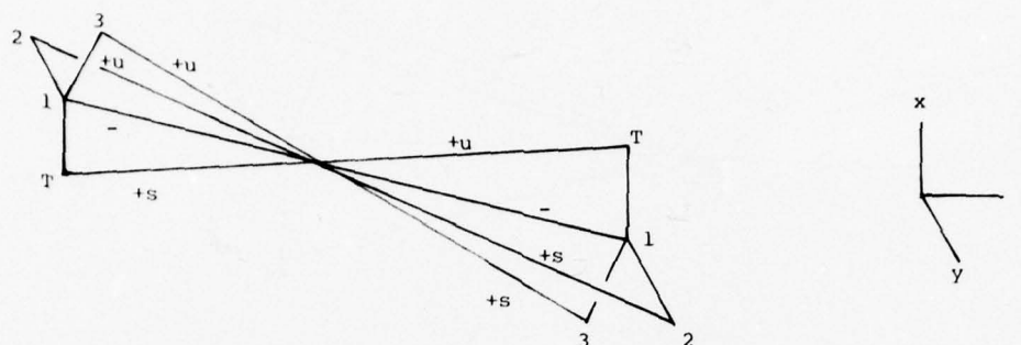
Figure 2.2e: Unperturbed III_2
