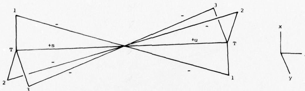
Figure 2.2c: Unperturbed III_0
