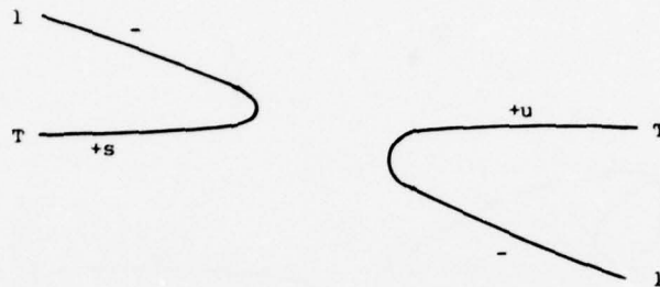
Figure 2.4a 1 : I_0, \epsilon > 0
