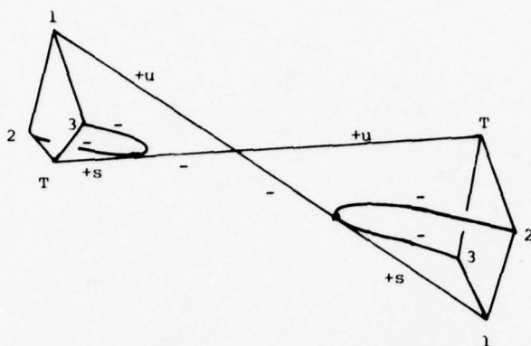
Figure 2.3d 1 : III_1, (-1)^{k_\delta} > 0
