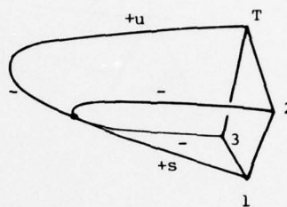
Figure 2.4d 1 : III_1 , \epsilon > 0 , region 5, k odd or even
