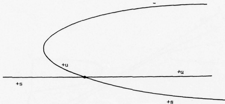
Figure 2.5: Behavior in the large
