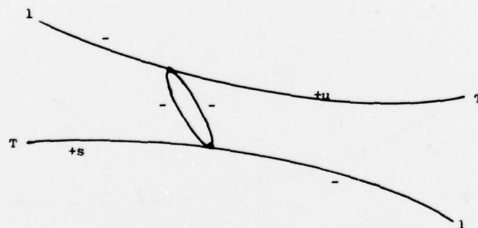
Figure 2.4a 2 : I_0 , unphysical
