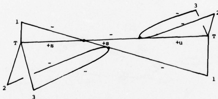
Figure 2.3c 2 : III_0, (-1)^k \delta < 0
