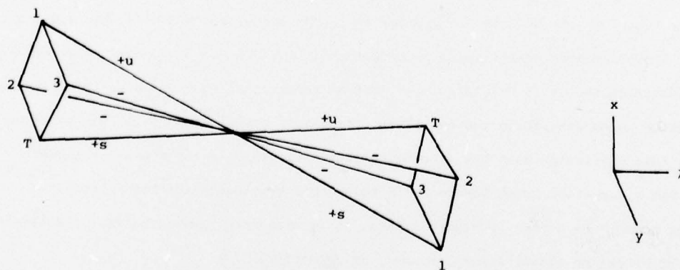
Figure 2.2d: Unperturbed III_1
