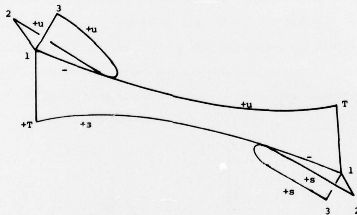
Figure 2.4e 2 : III 2 , \epsilon > 0 , k even
