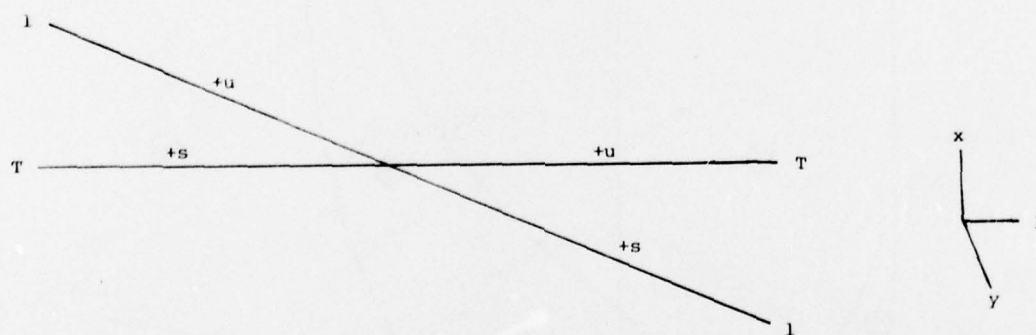
Figure 2.2b: Unperturbed I_1
