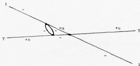
Figure 2.3a 1 : I_0, (-1)^{k_\delta} > 0
