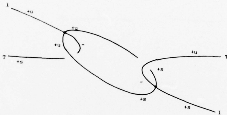
Figure 2.4b 1 : I_1 , unphysical
