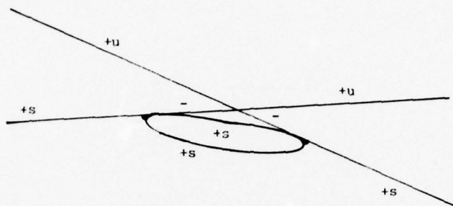
Figure 2.3b 1 : I_1, (-1)^k \delta > 0
