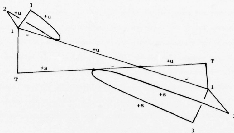
Figure 2.3e 1 : III_2, (-1)^k \delta > 0
