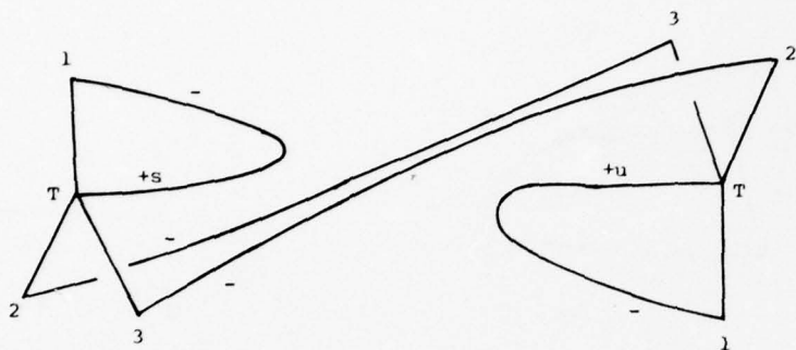
Figure 2.4c 1 : III_0 , \epsilon > 0 , k even
