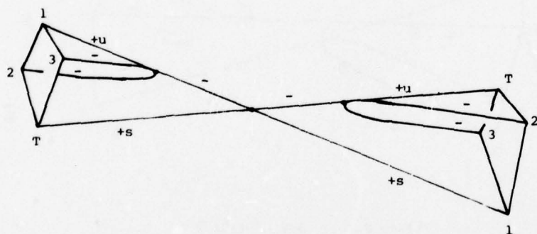
Figure 2.3d 2 : III_1, (-1)^{k_\delta} < 0
