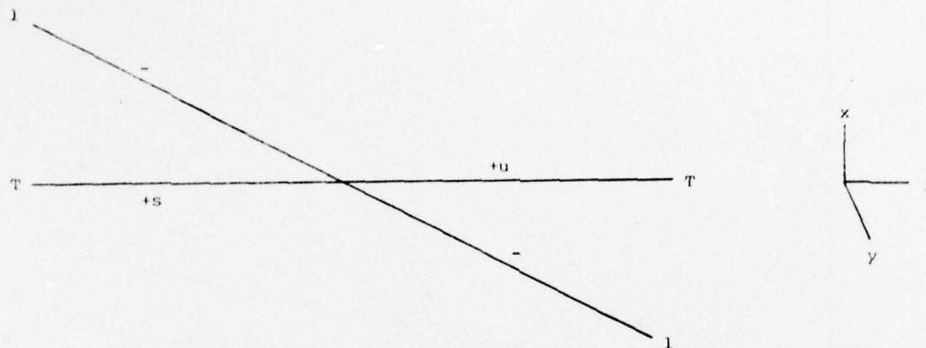
Figure 2.2a: Unperturbed I_0
