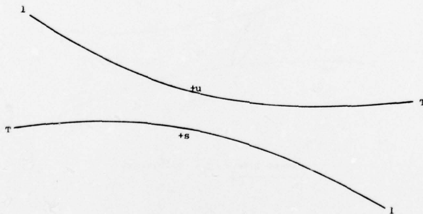
Figure 2.4b 2 : I_1 , \epsilon > 0
