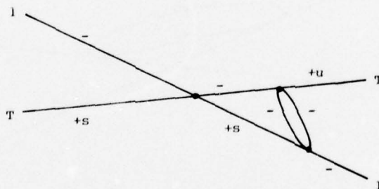
Figure 2.3a 2 : I_0, (-1)^{k_\delta} < 0
