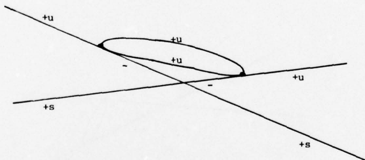
Figure 2.3b 2 : I_1, (-1)^k \delta < 0
