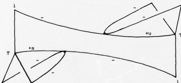
Figure 2.4c 2 : III_0 , \epsilon > 0 , k odd
