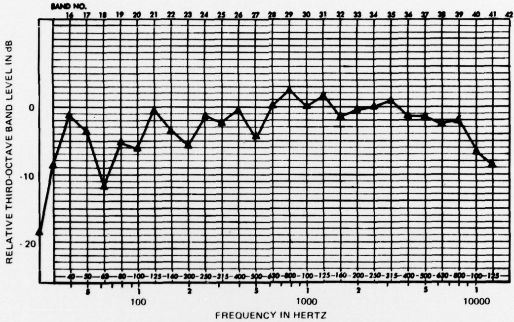
One-third octave acoustic response of playback system in studio with pink noise input.
