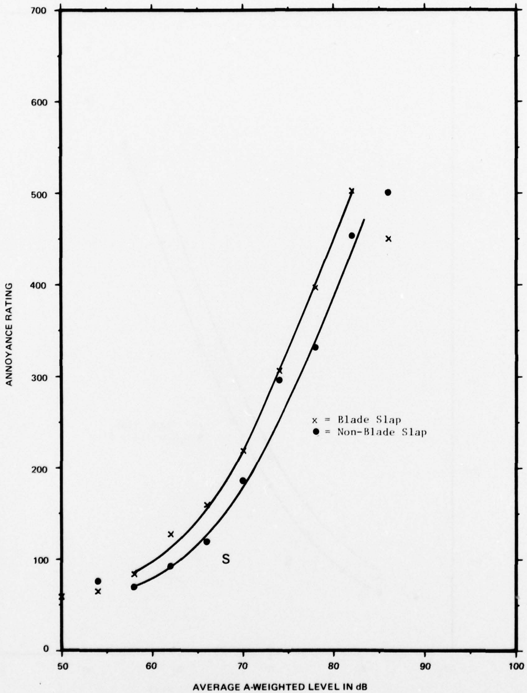
Figure 10. Mean annoyance ratings of laboratory group of 9 bladeslap sounds with 9 non-bladeslap sounds occurring during the same flight.
