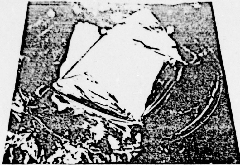
Figure 2. (a) Photograph of ruptured aluminum diaphragm showing quadrant petaling pattern.
