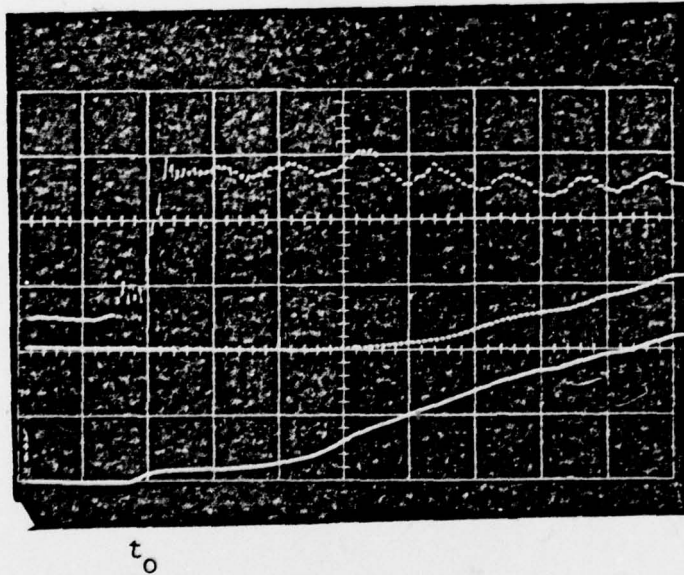
Figure 7. Nebulized RJ-5 combustion experiment at 1500°K. Lower trace: infrared emission from CO 2 (0.5 v/cm), middle trace, visible emission; upper trace, pressure profile. Sweep speed 100 \mu sec/cm, t_0 marks reflected shock arrival at observation station.
