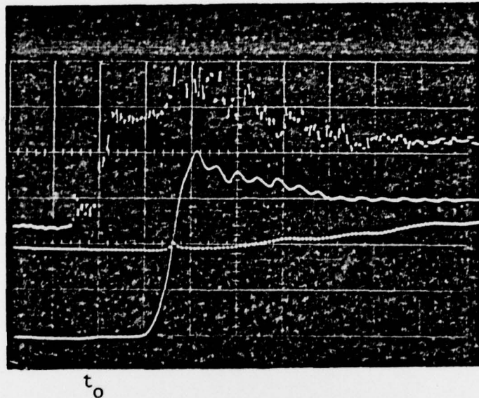
Figure 9. Nebulized RJ-5 combustion at 1700°K. Lower trace: infrared emission from \text{CO}_2 (1 v/cm); middle trace, visible emission, upper trace, pressure profile. Sweep speed 100 \mu\text{sec}/\text{cm} , t_0 marks reflected shock arrival at observation station.
