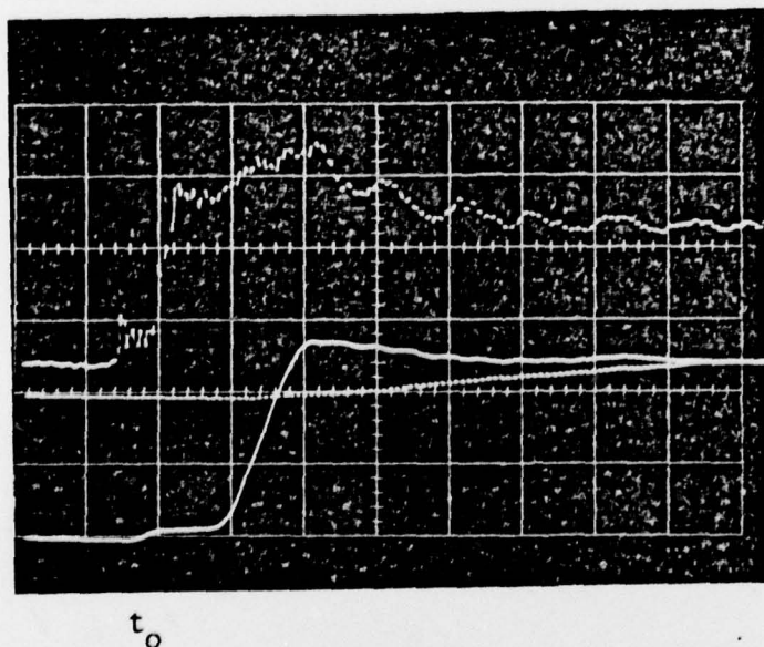
Figure 8. Nebulized RJ-5 combustion at 1700°K. Lower trace: infrared emission from \text{CO}_2 (1 v/cm); middle trace, visible emission; upper trace, pressure profile. Sweep speed 100 \mu sec/cm, t_0 marks reflected shock arrival at observation station.
