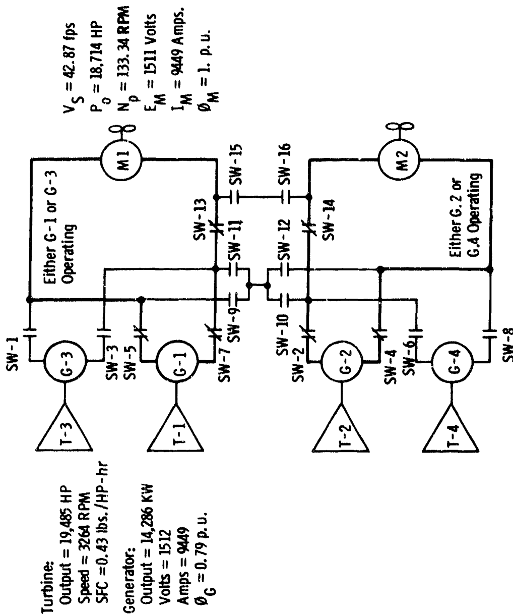
Figure 2.2. One Half Power Configuration
