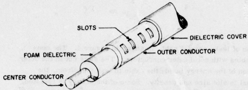
Figure 4. Construction Details of Ported Coaxial Cable
