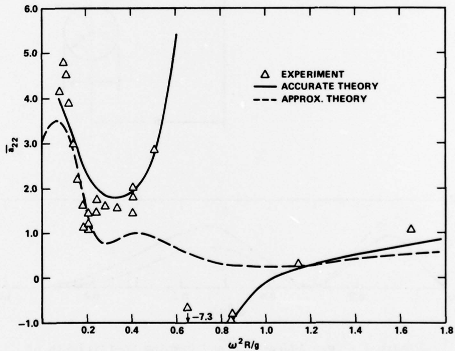
Figure 6 - Sway Added-Mass Coefficient of a SWATH Section
