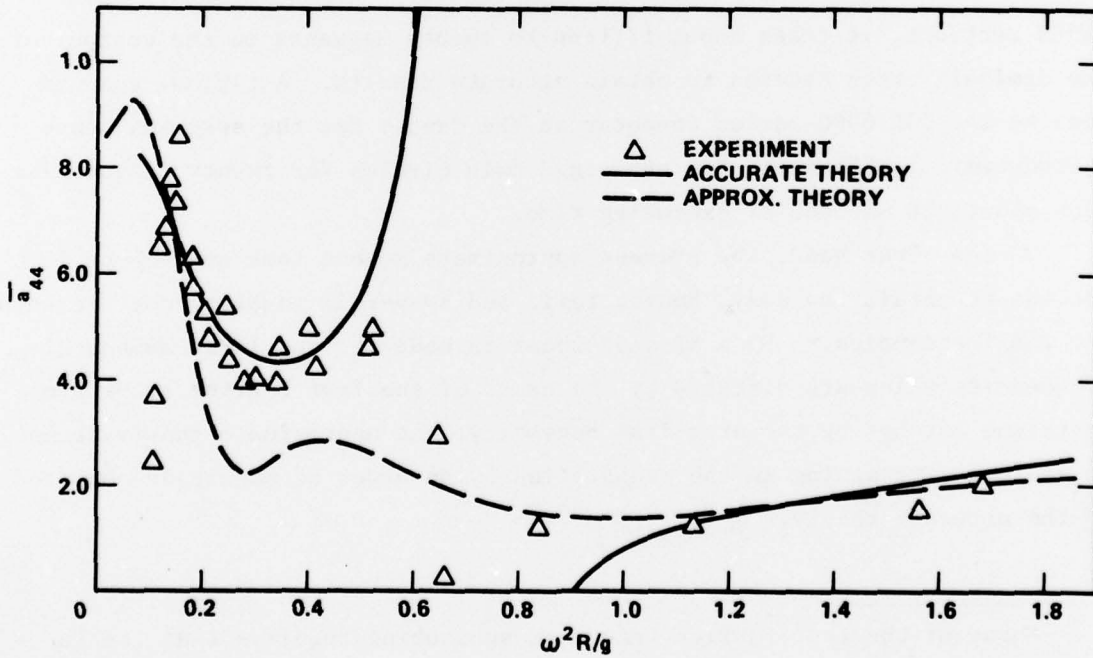
Figure 9 - Roll Added-Inertia Coefficient of a SWATH Section
