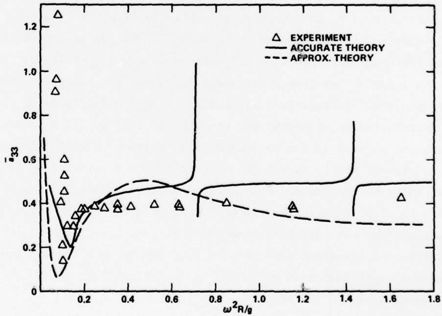
Figure 3 - Heave Added-Mass Coefficient of a SWATH Section
