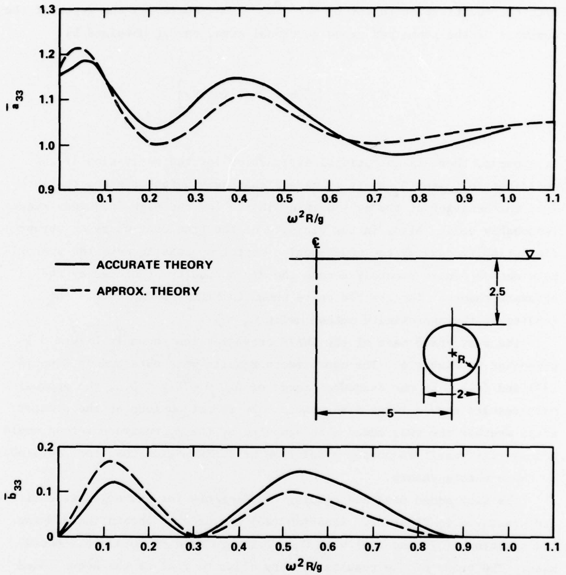
Figure 4 - Heave Added-Mass and Damping Coefficients of Submerged Twin Circles
