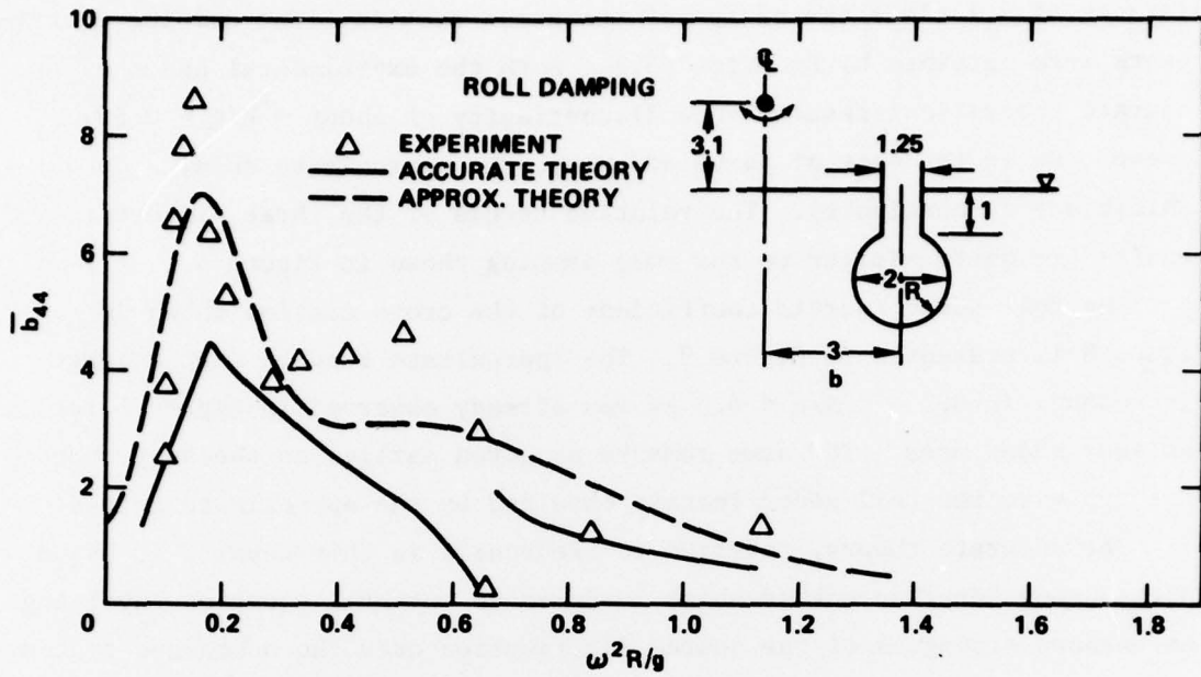
Figure 8 - Roll Damping Coefficient of a SWATH Section
