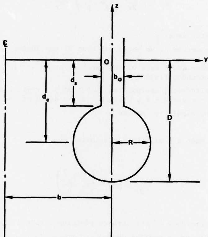
Figure 1 - Demihull Cross Section of a SWATH Ship
