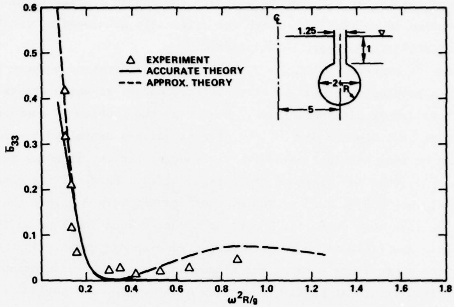
Figure 2 - Heave Damping Coefficient of a SWATH Section
