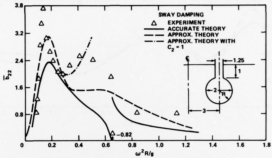
Figure 5 - Sway Damping Coefficient of a SWATH Section
