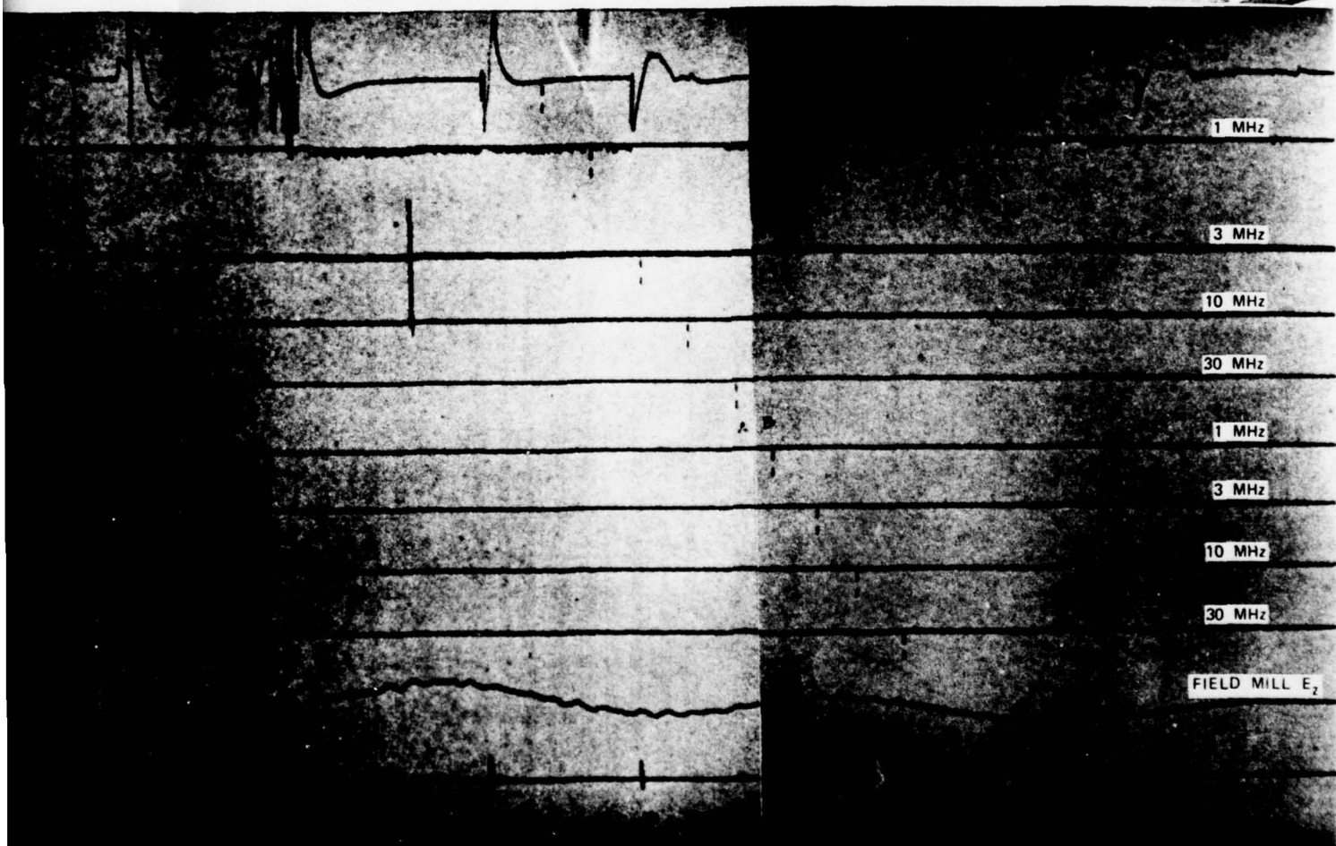
FIGURE 4-3 RECORD OF LIGHTNING STRIKE TO LEAR JET
