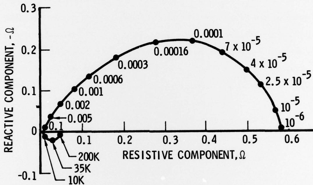
Fig. 4. The Impedance of Nickel Cadmium Cell L1-137 at 25.05°C and a State of Charge of About 60%. The impedance from 10 -6 to 0.1 Hz was obtained from the voltage transient of Figure 3, while from 10 Hz to 200 KHz it was obtained using an alternating current method.
