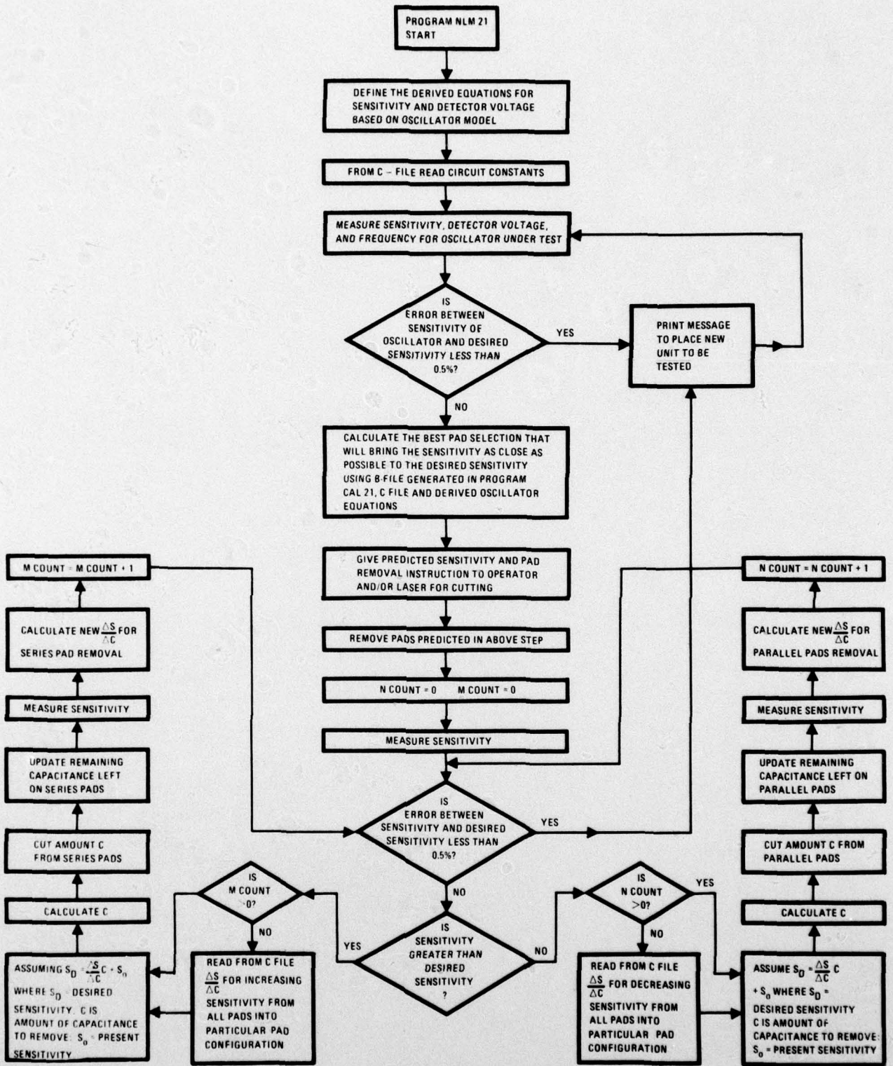
Figure A-3. Flow Chart For Program NLM-21
