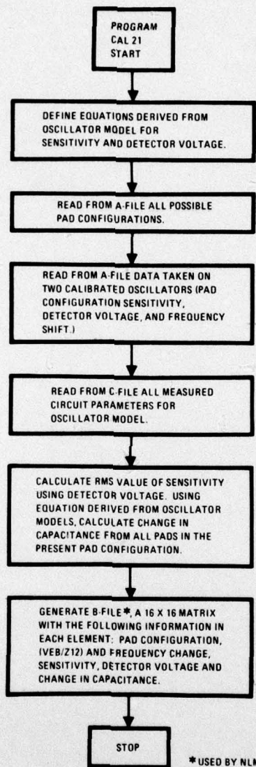
Figure A-2. Flow Chart For Program CAL-21
