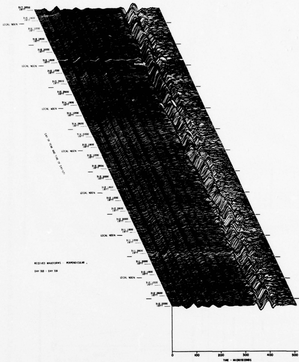
Figure 12. VLF/LF Reflectivity Data for the Polar Ionosphere, DAY 310 (6 Nov) - DAY 316 (12 Nov) 1977 (Cont) Part S. \perp Waveform Display
