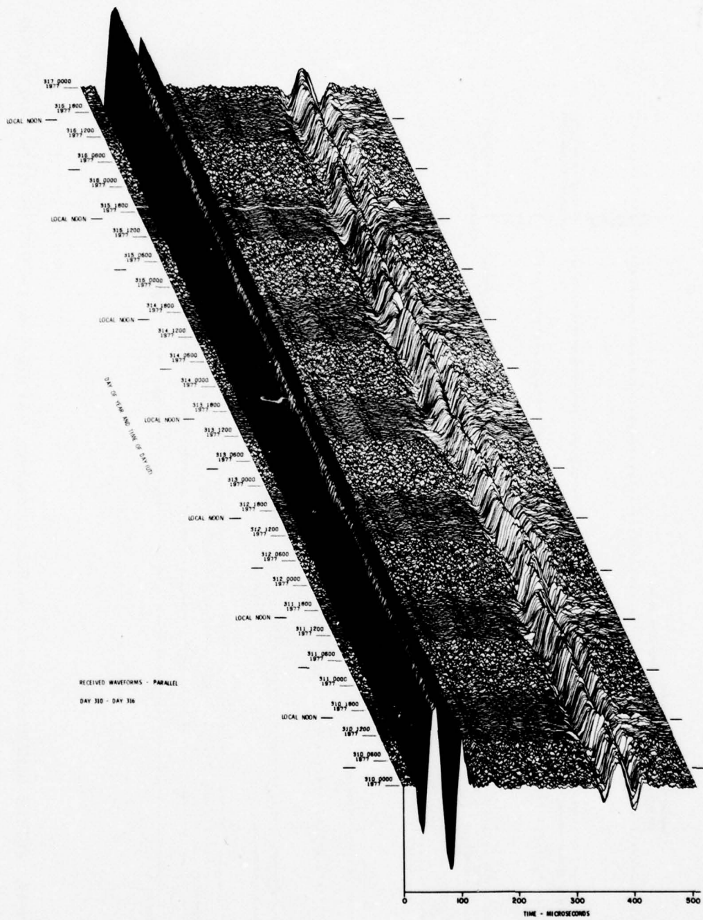
Figure 12. VLF/LF Reflectivity Data for the Polar Ionosphere, DAY 310 (6 Nov) - DAY 316 (12 Nov) 1977 (Cont) Part R. \parallel Waveform Display
