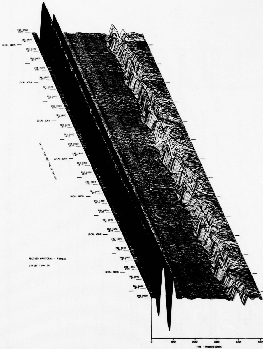
Figure 9. VLF/LF Reflectivity Data for the Polar Ionosphere, DAY 289 (16 Oct) - DAY 295 (22 Oct) 1977 (Cont) Part R. \parallel Waveform Display
