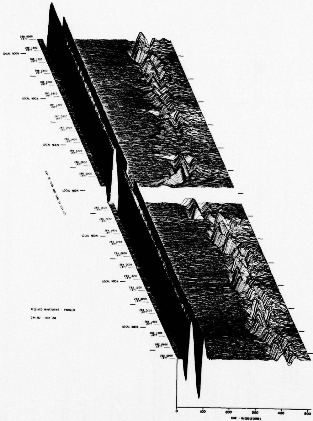
Figure 8. VLF/LF Reflectivity Data for the Polar Ionosphere, DAY 282 (9 Oct) - DAY 288 (15 Oct) 1977 (Cont) Part R. || Waveform Display
