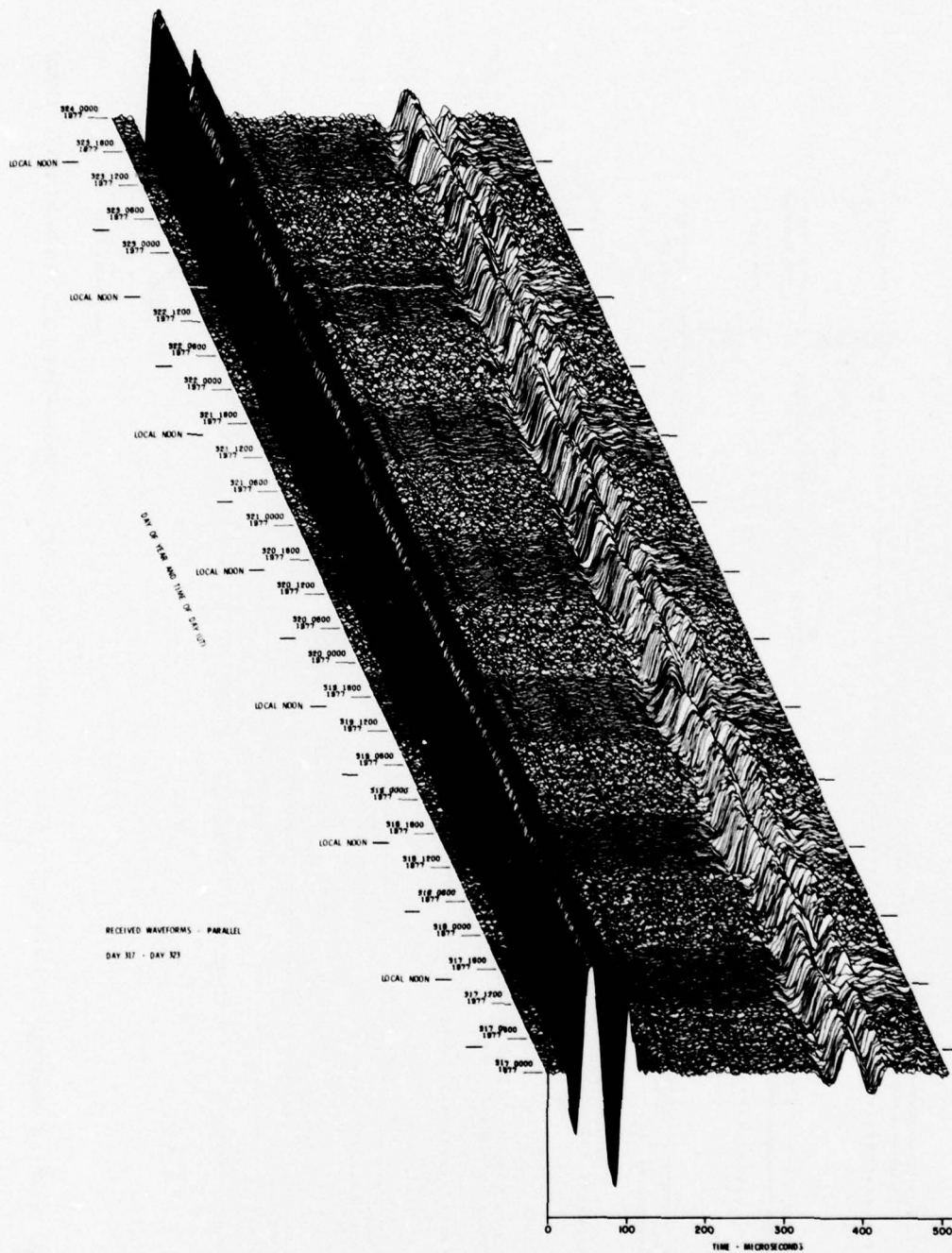
Figure 13. VLF/LF Reflectivity Data for the Polar Ionosphere, DAY 317 (13 Nov) - DAY 323 (19 Nov) 1977 (Cont) Part R. // Waveform Display
