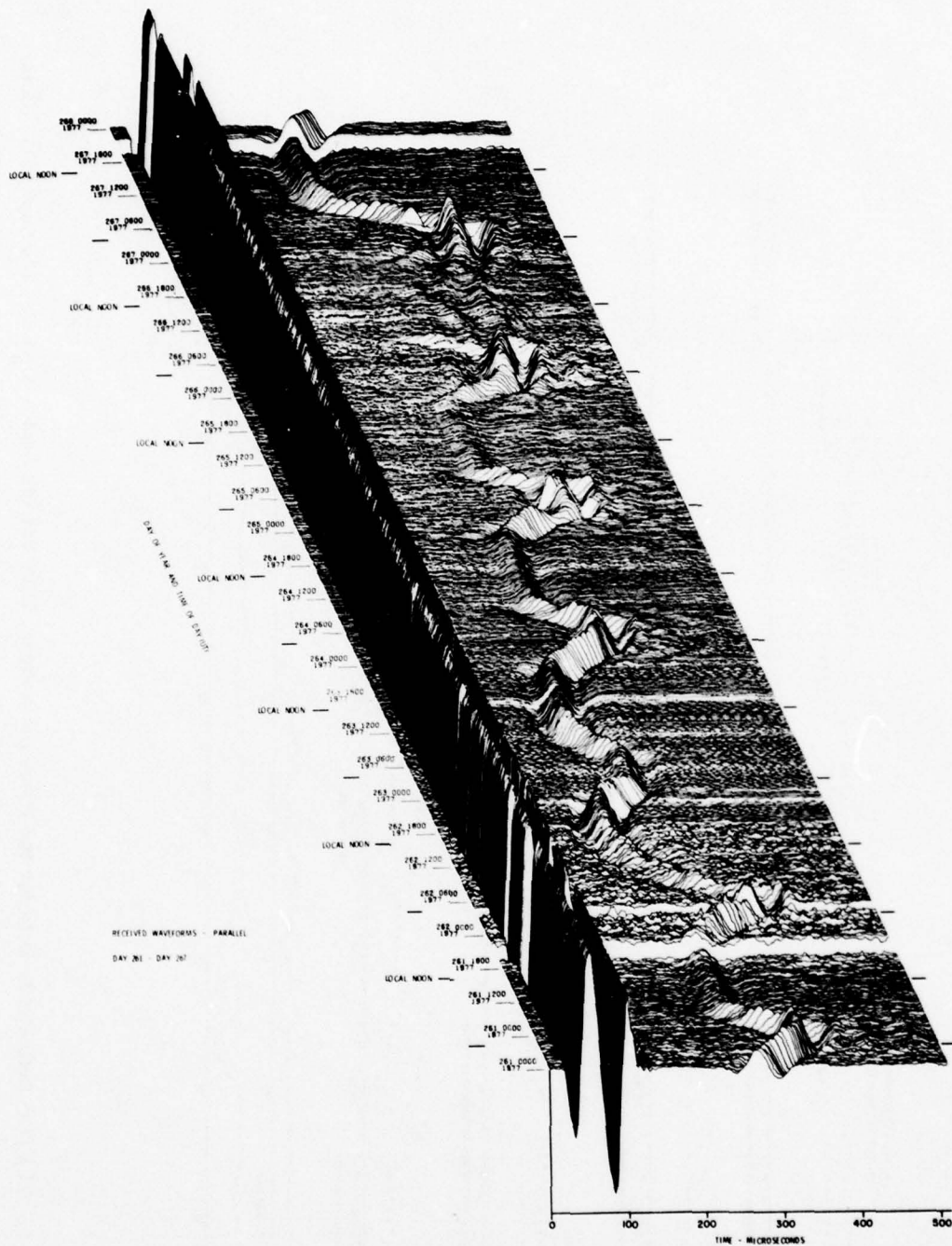
Figure 5. VLF/LF Reflectivity Data for the Polar Ionosphere, DAY 261 (18 Sep) - DAY 267 (24 Sep) 1977 (Cont) Part R. || Waveform Display
