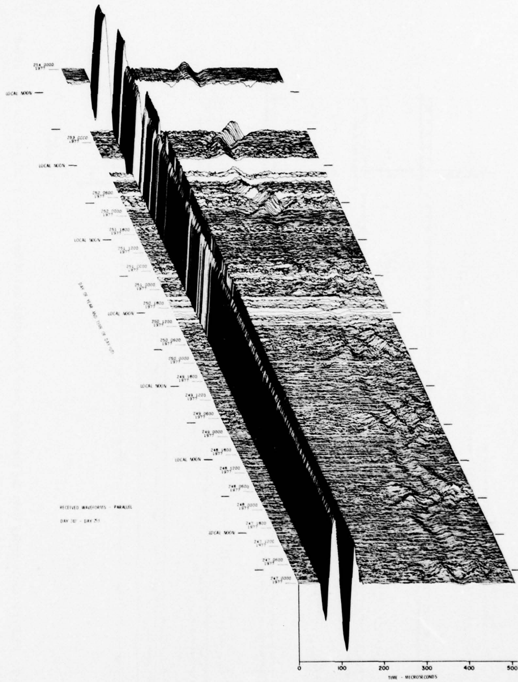
Figure 3. VLF/LF Reflectivity Data for the Polar Ionosphere, DAY 247 (4 Sep) - DAY 253 (10 Sep) 1977 (Cont) Part R. || Waveform Display
