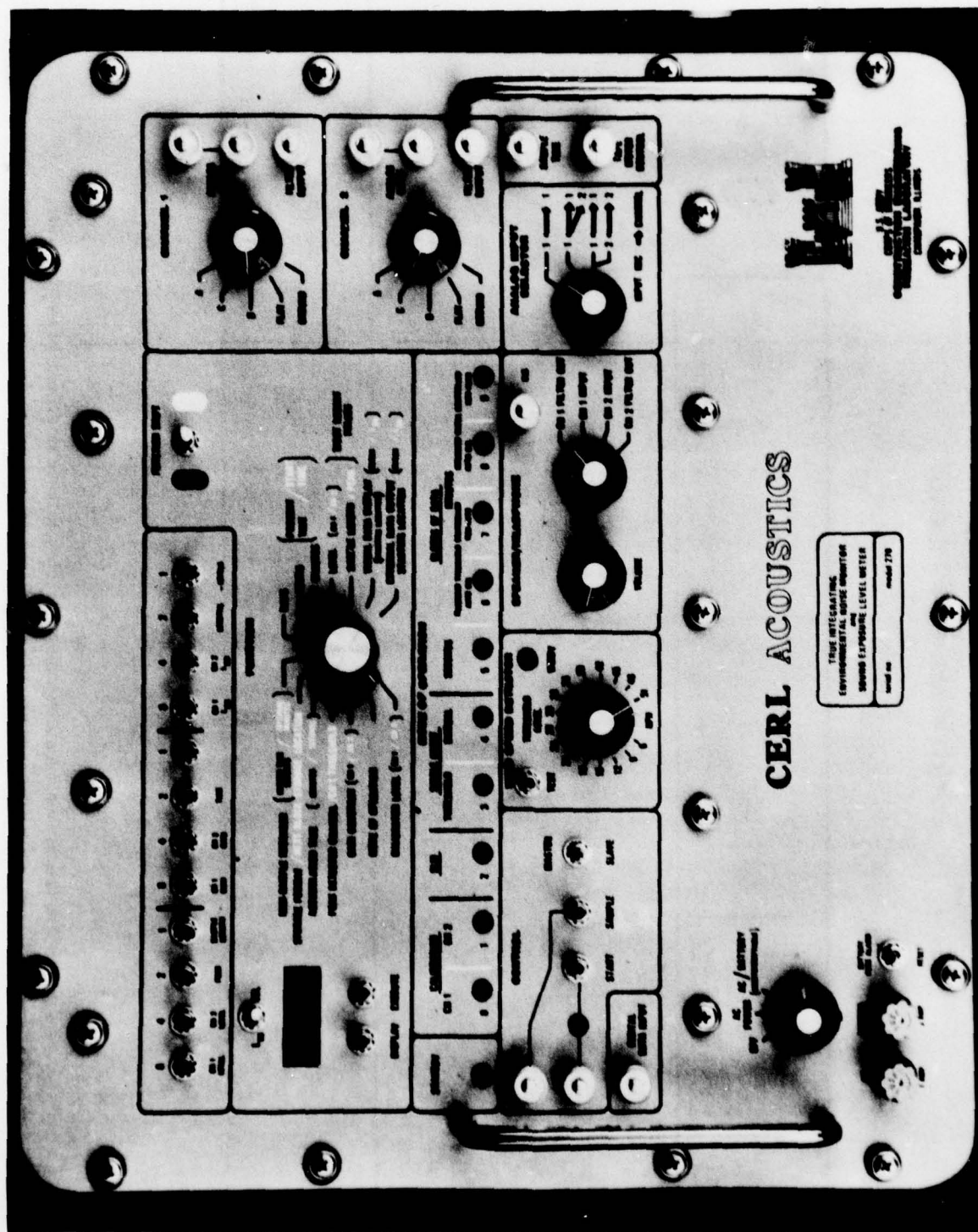
Figure 4. Front panel of the True-Integrating Noise Monitor and Sound-Level Meter.
