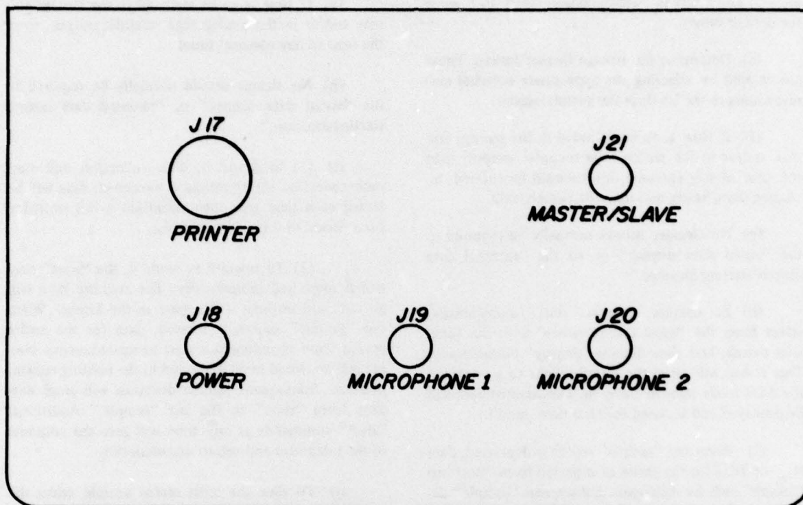
Figure 6. Monitor side connectors layout.
