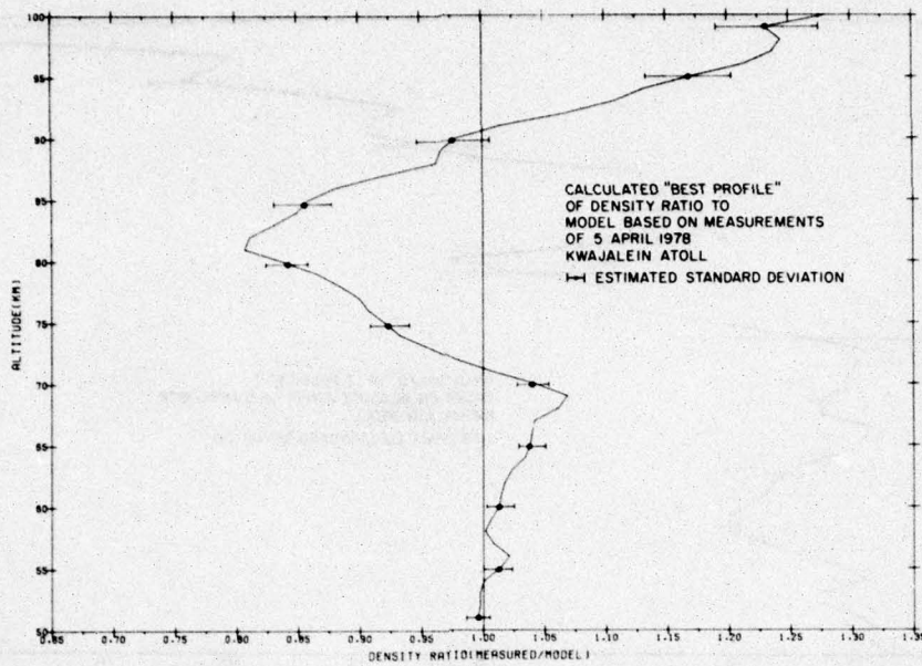
Figure 12a. "Best Profile" Density Ratio to the Model From the Analysis With Weights Dependent on Sensor Accuracy and Atmospheric Variability
