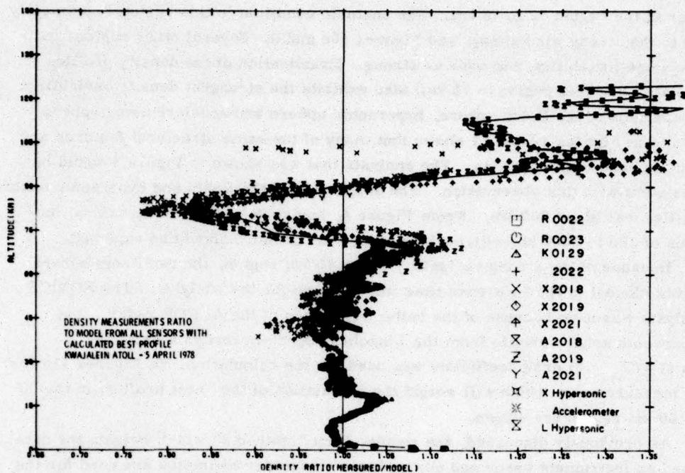
Figure 9a. Summary Plot From 0 to 130 km of all of the Density Measurements of 5 April 1978 Compared to the USSAS 1966 (15 0 Annual) Model With the Calculated Best Profile Shown as a Line. The flight identification numbers are shown (see Table 1) and the X, A and L denote data processed by XONICS, ASL and Lincoln Laboratory, respectively
