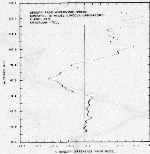
Figure 8a. Hypersonic Sphere Density Results Compared to Model From the Lincoln Laboratory Analysis of the ALCOR Radar Data. Note the scale sizes of the vertical structure compared to the scales expected based on arguments presented in the text
