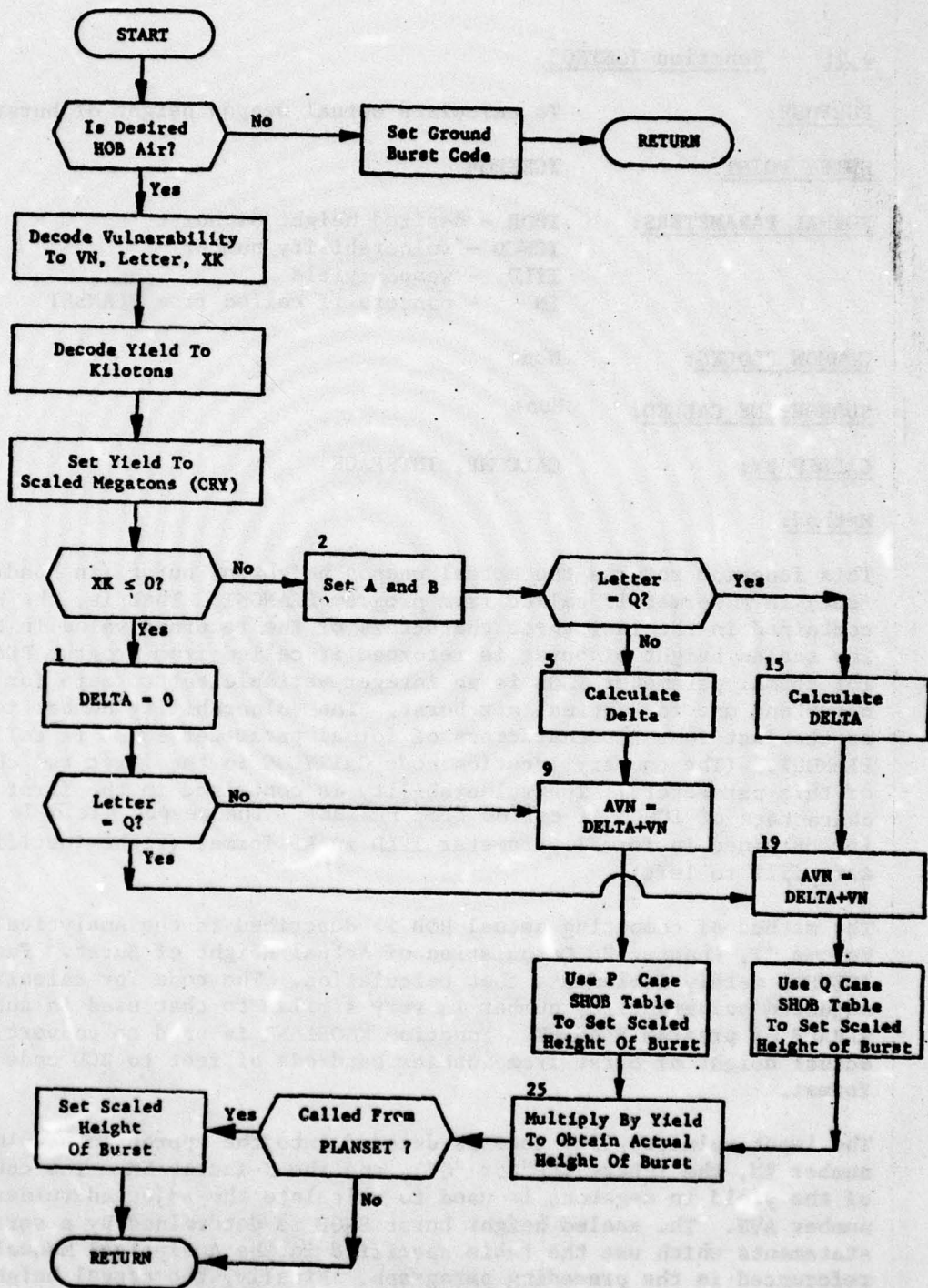
Figure 150. Function IGETHOB
