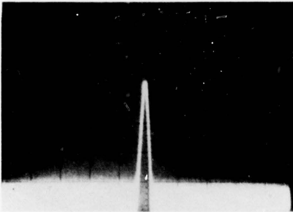
SPECTRUM OF SELF-OSCILLATION MODE V_T = 8.87 \text{ V} I_T = 11.9 \text{ mA} f_o = 3.01 \text{ GHz} (H - 1 MHz/DIV V - 10 dB/DIV)
