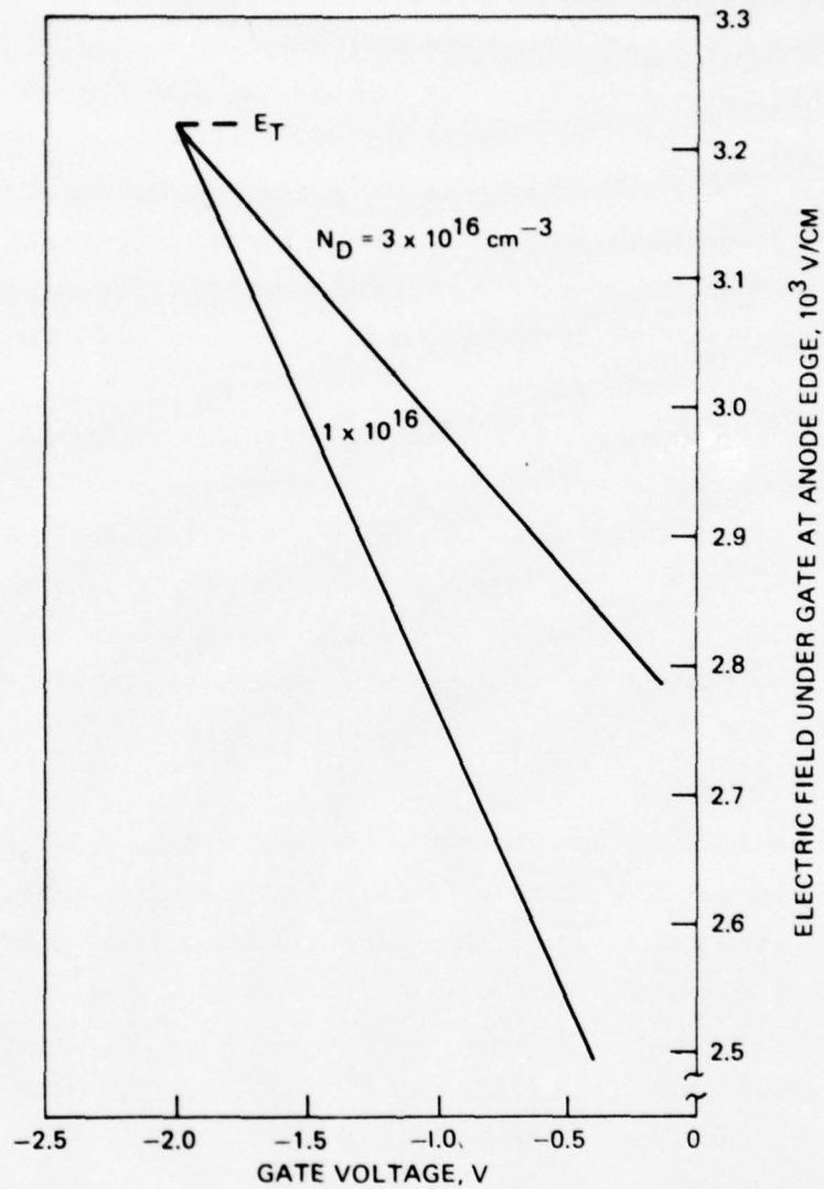
Figure 8. Electric field under the gate versus gate bias ( R_L = 182 \Omega , E_T = 3218 V/cm).
