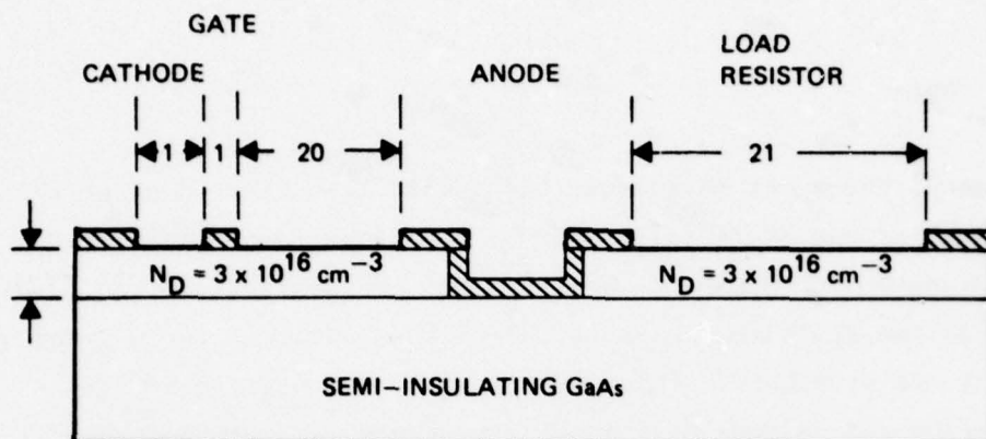
Figure 6. Schematic of TELED and load resistor ( \mu_n = 6000 \text{ cm}^2/\text{V}\cdot\text{sec} , E_T = 3.2 \times 10^3 \text{ V/cm} ). Dimensions in micrometers.
