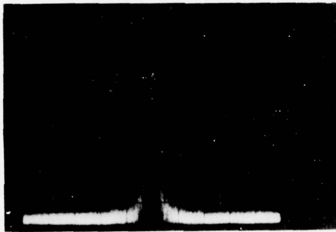
Figure 30. Spectrum of TELD transit time frequency ( f_0 = 2.94 GHz, vertical = 10 dB/div, horizontal = 1 MHz/div, V_{\text{bias}} = 11.1 V, I_D = 14.4 mA).
