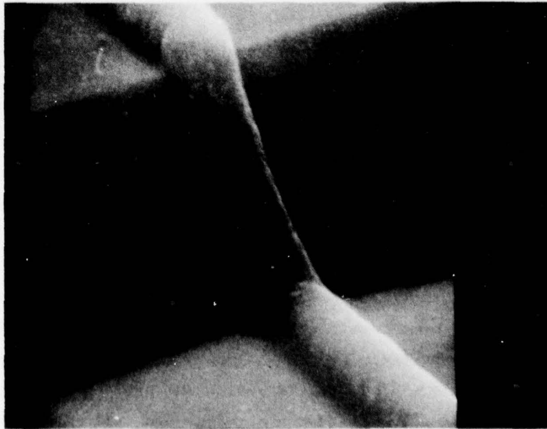
Figure 25. SEM photographs of 2- \mu\text{m} -high mesa with 7500- \text{\AA} -long by 4000- \text{\AA} -high gate deposited by E-beam lithography.
