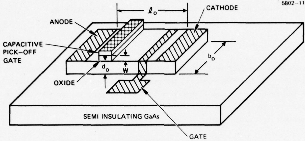
Figure 16. Planar structure of GaAs TELD with capacitively coupled pick-off gate.
