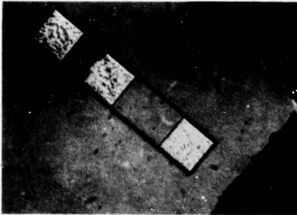
PHOTOMICROGRAPH OF TWO TERMINAL TED WITH RESISTOR LOAD (210 x)
