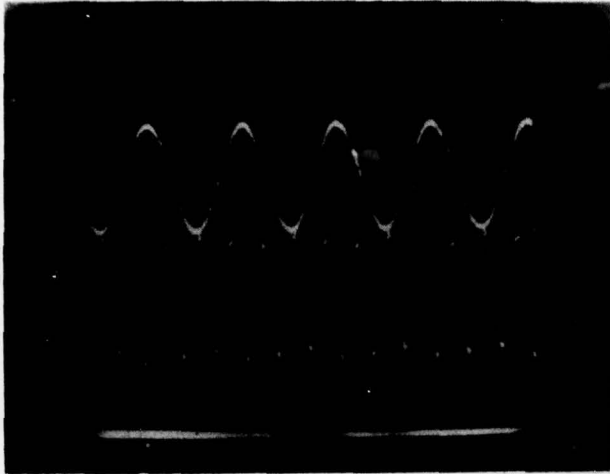
Figure 34. Output waveform of divide- by-three TELED ( f_{in} = 7.095 \text{ GHz} , f_o = 2.365 \text{ GHz} ).
