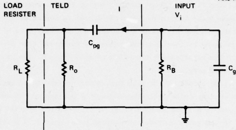
Figure 19. Equivalent circuit of MOS pick-off gate and input to next stage.
