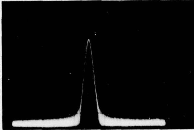
Figure 32. Spectrum of TELD low-frequency oscillation ( f = 1.001 GHz, vertical = 10 dB/div, horizontal = 500 kHz/div, V_{\text{bias}} = 11.1 V, I_{\text{D}} = 14.5 mA).
