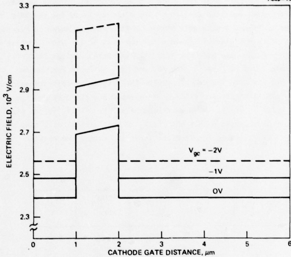
Figure 7. Electric field versus distance for TELD and load resistor in Figure 6 ( V_{\text{bias}} = 11.1 V, I_{\text{DS}} = 29.75 mA).
