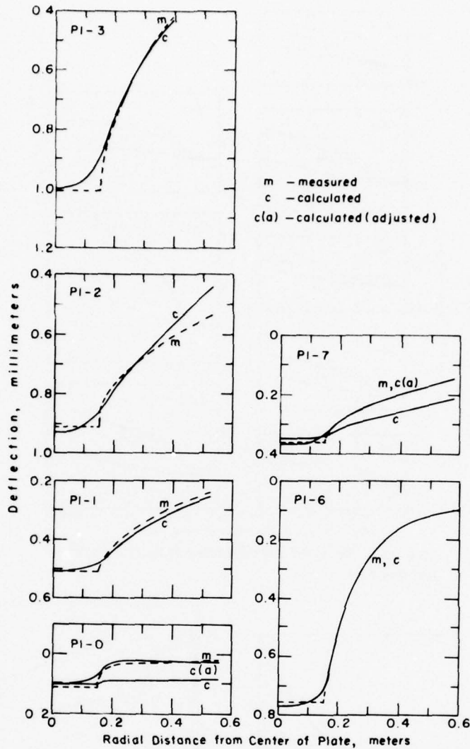
Figure 10. Measured and calculated deflection basins, test point P1.
