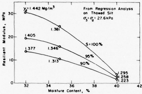
Figure 27. Influence of moisture content and dry density on the resilient modulus of thawed silt.
