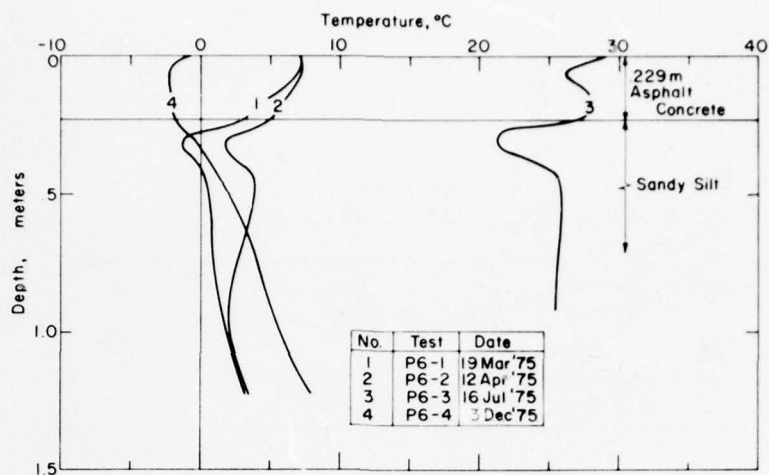
Figure A3. Ground temperatures at test point P6.
