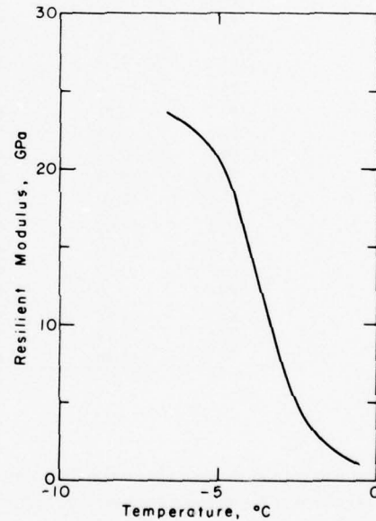
Figure 9. Resilient modulus of frozen silt used in analysis.
