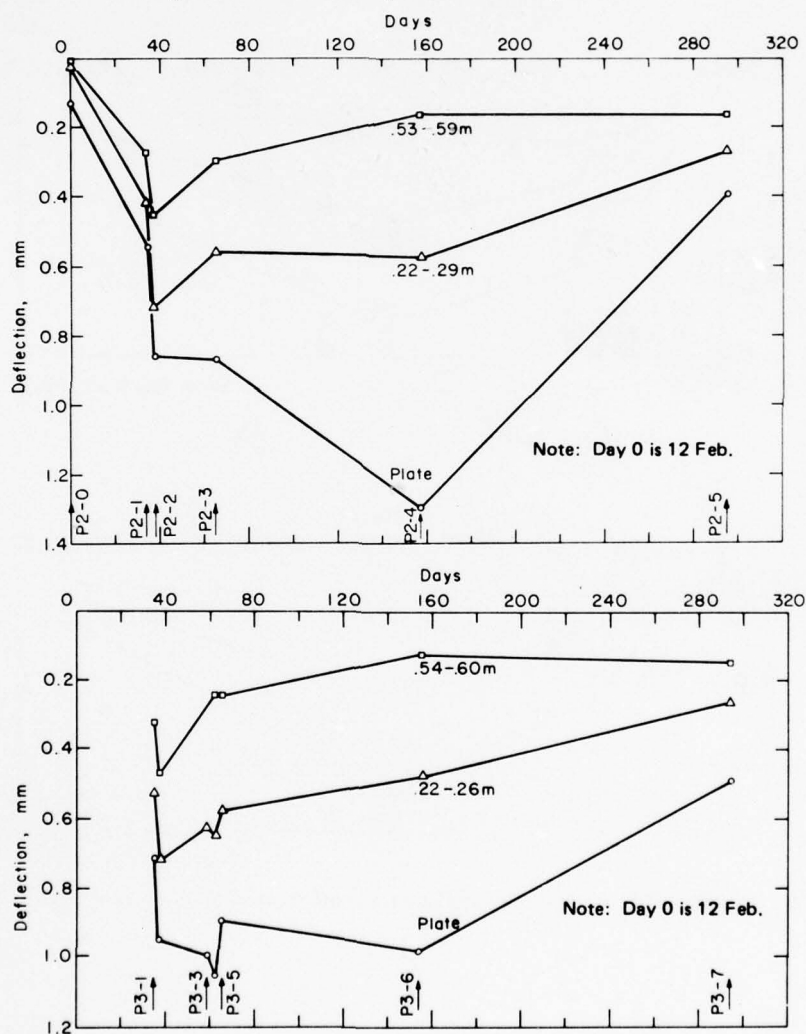
Figure A4. Resilient deflection of plate and two radial points, test points P2 and P3.
