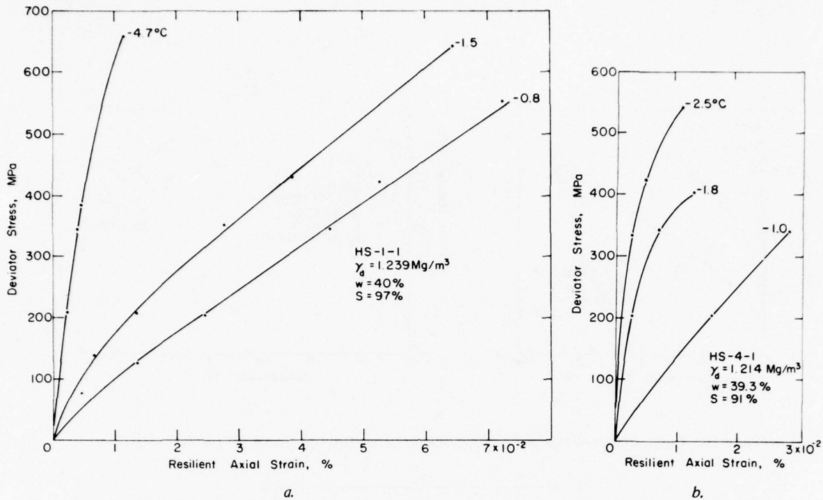
Figure 19. Resilient axial strains and deviator stresses measured on two specimens of frozen silt.
