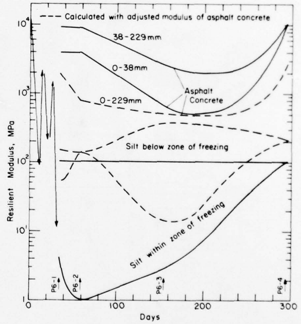
Figure A7. Calculated resilient moduli of subgrade silt, and moduli of asphalt concrete used in analyses, test points P2, P3, P5 and P6.
