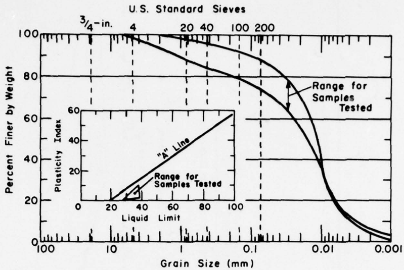
Figure 2. Properties of silt.
