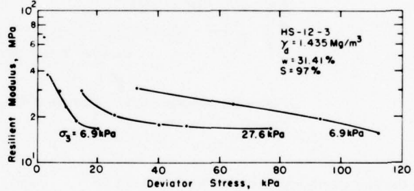
Figure 23. Resilient moduli of two thawed silt specimens.
