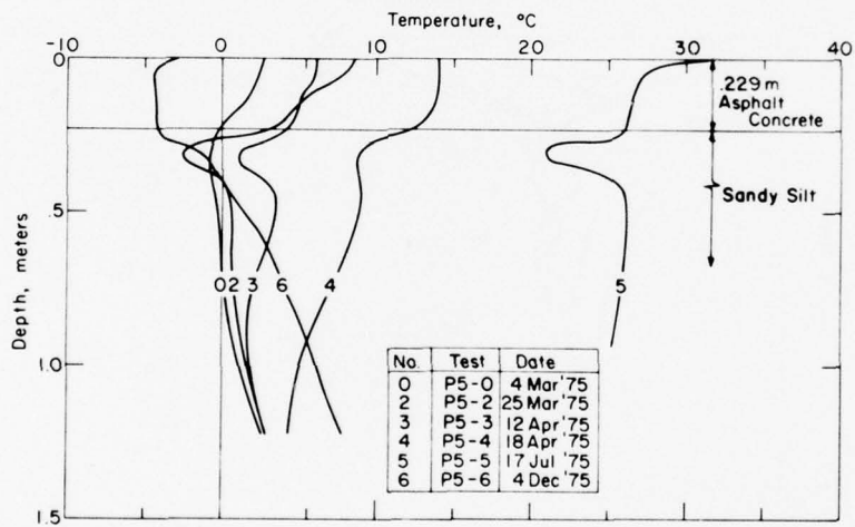
Figure A2. Ground temperatures at test points P4 and P5.
