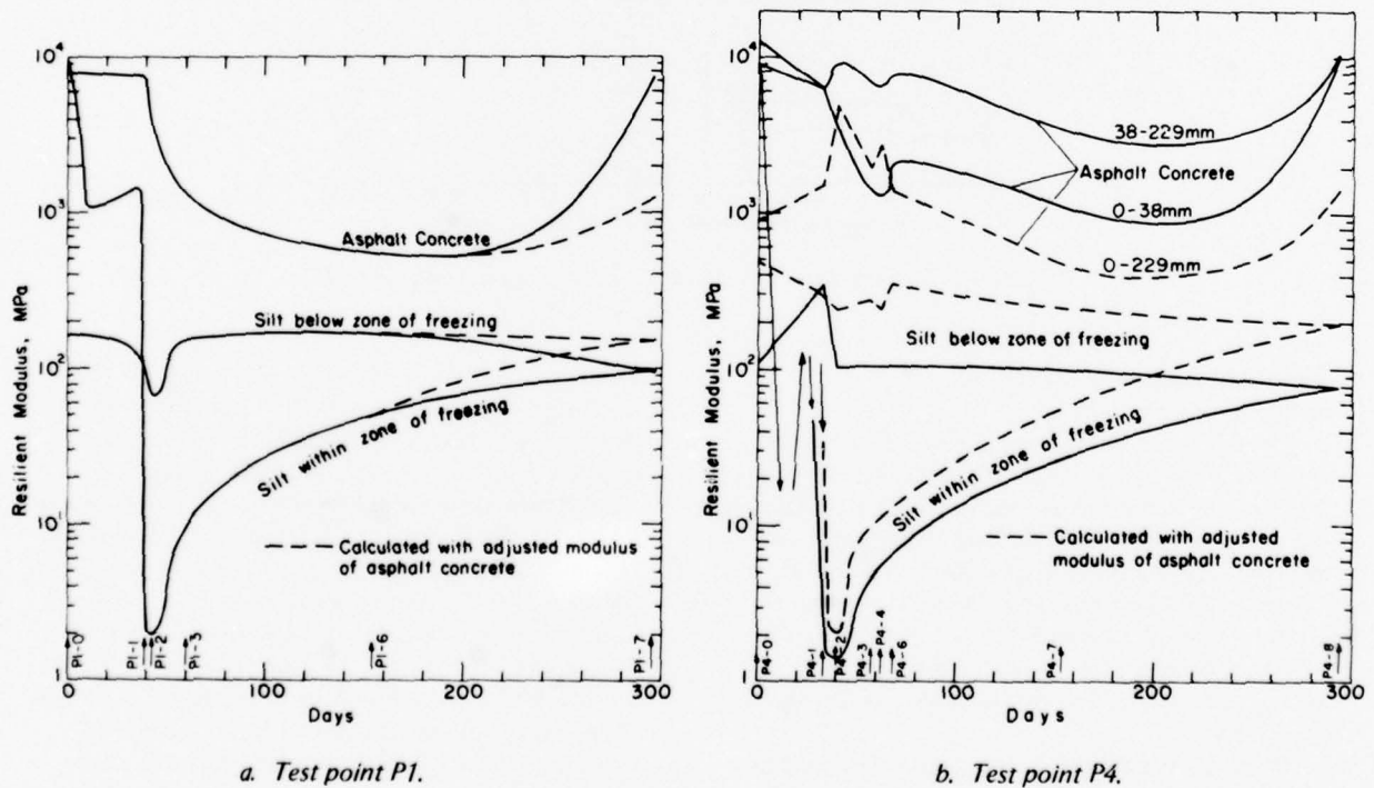
Figure 12. Calculated resilient moduli of subgrade silt, and moduli of asphalt concrete used in analyses, test points P1 and P4.
