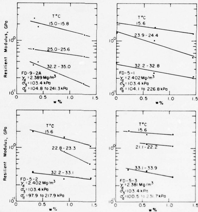
Figure 16. Effect of moisture content on resilient modulus of four asphalt concrete specimens.
