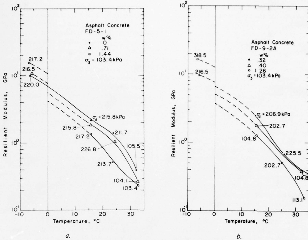
Figure 15. Effect of temperature on resilient modulus of two asphalt concrete specimens.
