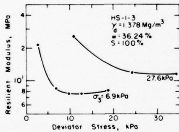
Figure 23. Resilient moduli of two thawed silt specimens.
