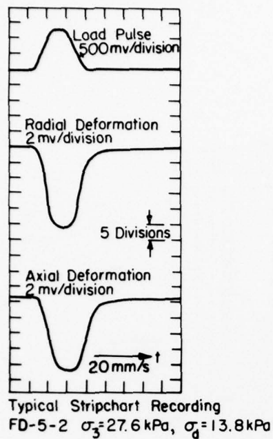
Figure 14. Typical load and deformation strip-chart recordings.
