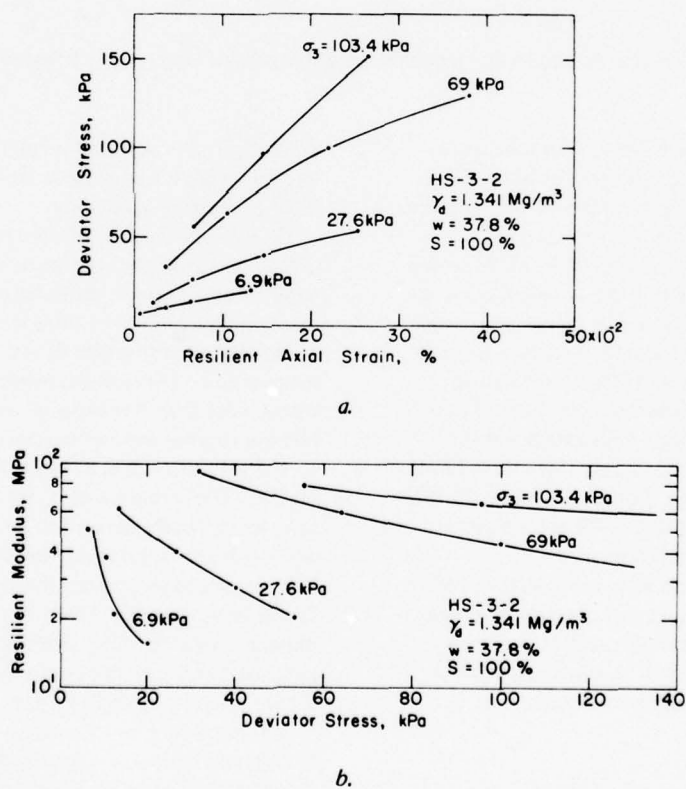
Figure 21. Resilient axial strains and resilient moduli, thawed silt specimen HS-3-2.
