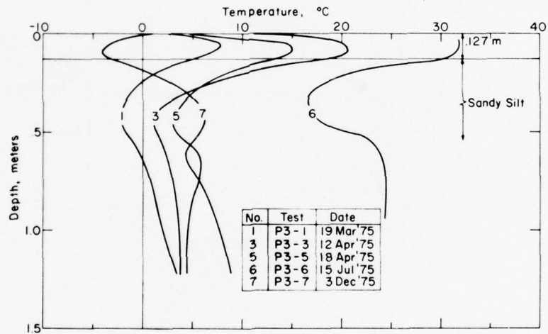
Figure A1. Ground temperatures at test points P2 and P3.
