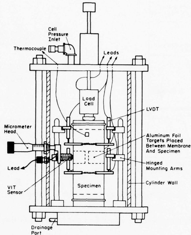
Figure 13. Triaxial cell.
