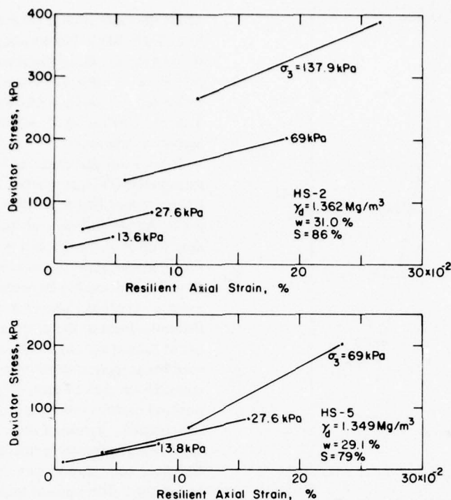
Figure 25. Resilient axial strains in two fully recovered silt specimens.
