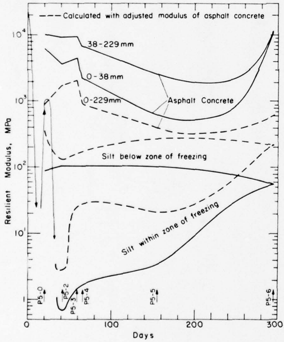
Figure A7. Calculated resilient moduli of subgrade silt, and moduli of asphalt concrete used in analyses, test points P2, P3, P5 and P6.
