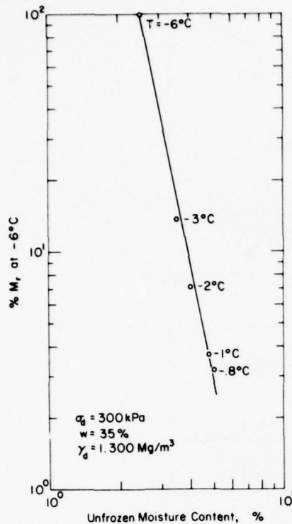
Figure 26. Variation in resilient modulus of frozen silt with unfrozen moisture content.
