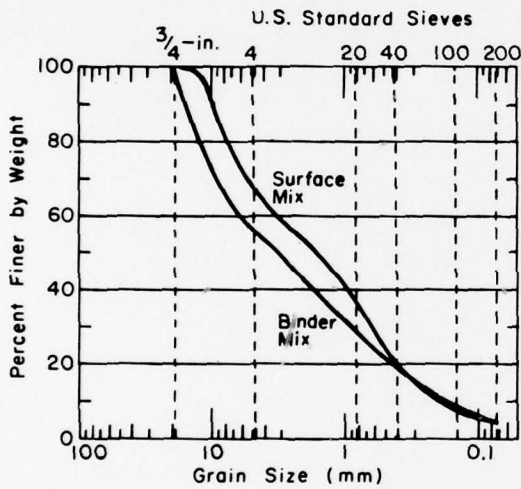
Figure 3. Aggregates for asphalt concrete.
