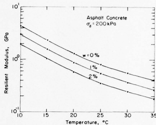
Figure 18. Results of regression analysis, effect of temperature and moisture content on unfrozen asphalt concrete.
