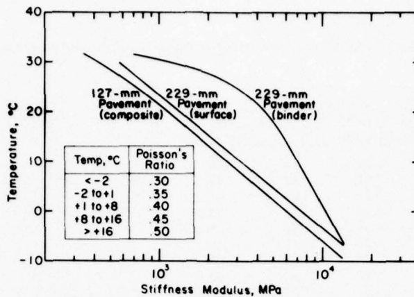
Figure 8. Stiffness modulus of asphalt concrete used in analysis.
