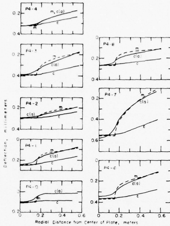
Figure 11. Measured and calculated deflection basins, test point P4.
