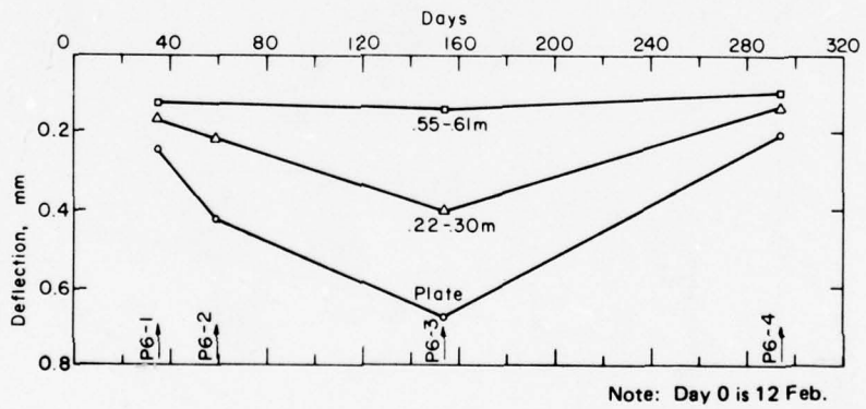
Figure A5. Resilient deflection of plate and two radial points, test points P4, P5 and P6.
