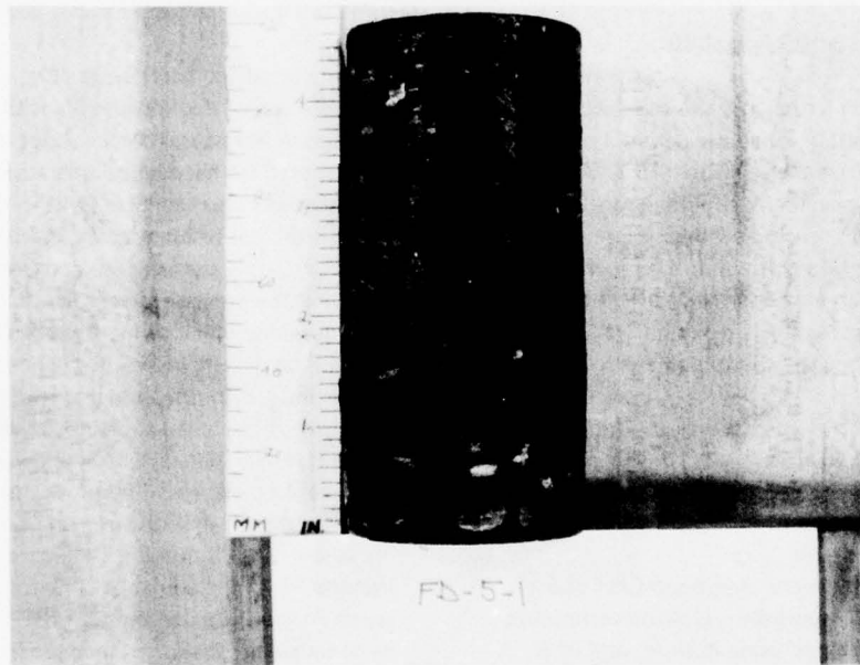
Figure 17. Asphalt concrete specimens after testing for moisture-induced damage.
