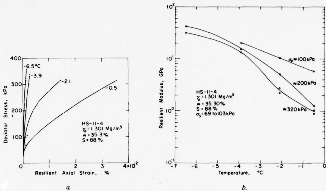
Figure 20. Resilient axial strains and resilient moduli determined on frozen silt specimen HS-11-4.
