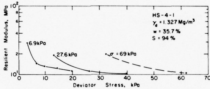
Figure 22. Resilient axial strains and resilient moduli, thawed silt specimen HS-4-1.
