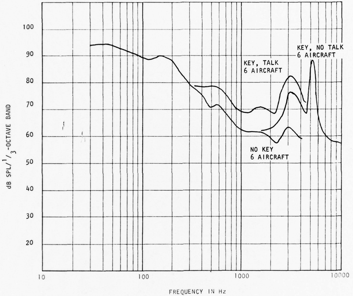
FIGURE 26 CH-54B TARHE: EARCUP NOISE DURING LEVEL FLIGHT. 1/3-OCTAVE WEIGHTED.
