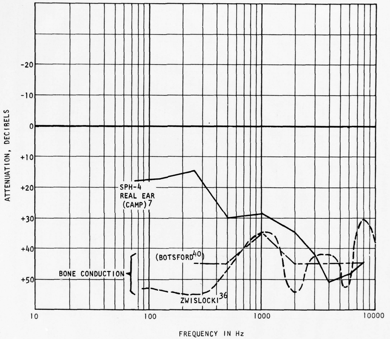
FIGURE 47. LIMITS TO EARCUP ATTENUATION (BONE CONDUCTION)
