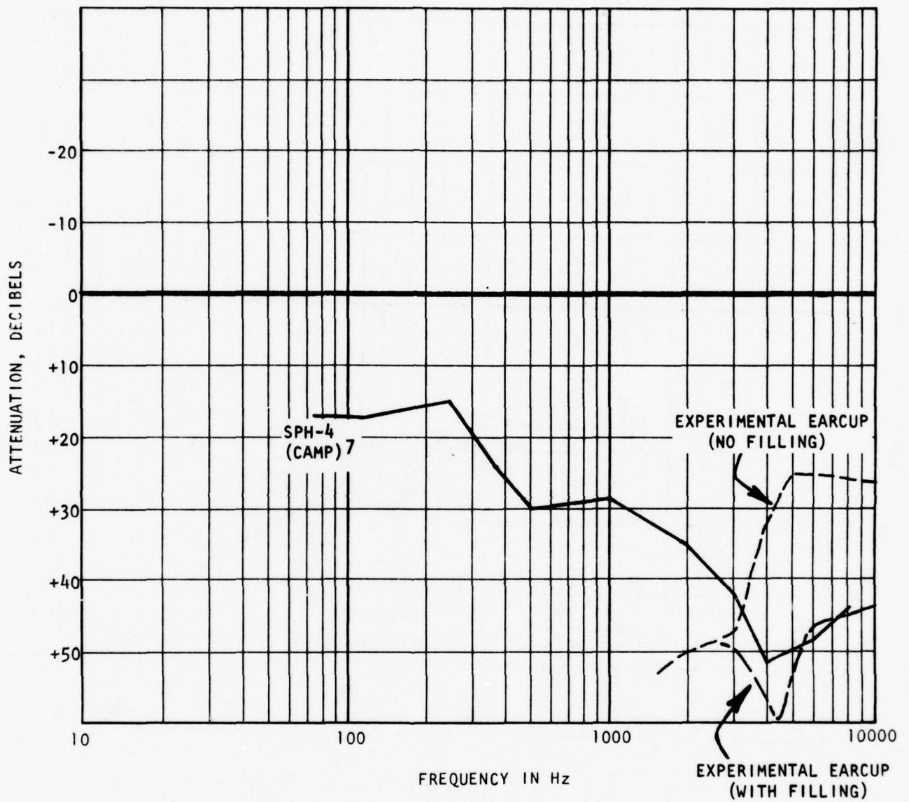
FIGURE 49. ATTENUATION OBTAINED BY FILLING EXPERIMENTAL CUP WITH SOUND-ABSORBING MATERIAL, ISOCYANATE FOAMED PLASTIC (SHAW AND THIESSEN 39 )
