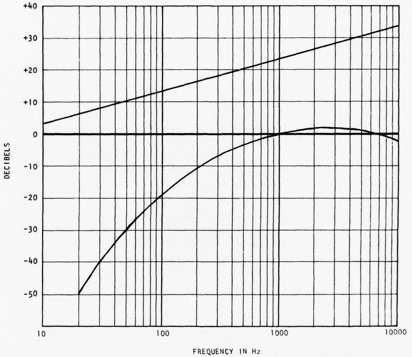
FIGURE 4 WEIGHTING CURVES:
