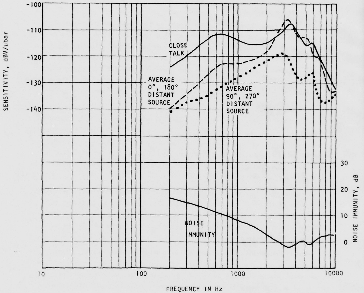
FIGURE 51. RESPONSE OF M-87 MICROPHONE, 5 Ω LOAD RESISTOR
