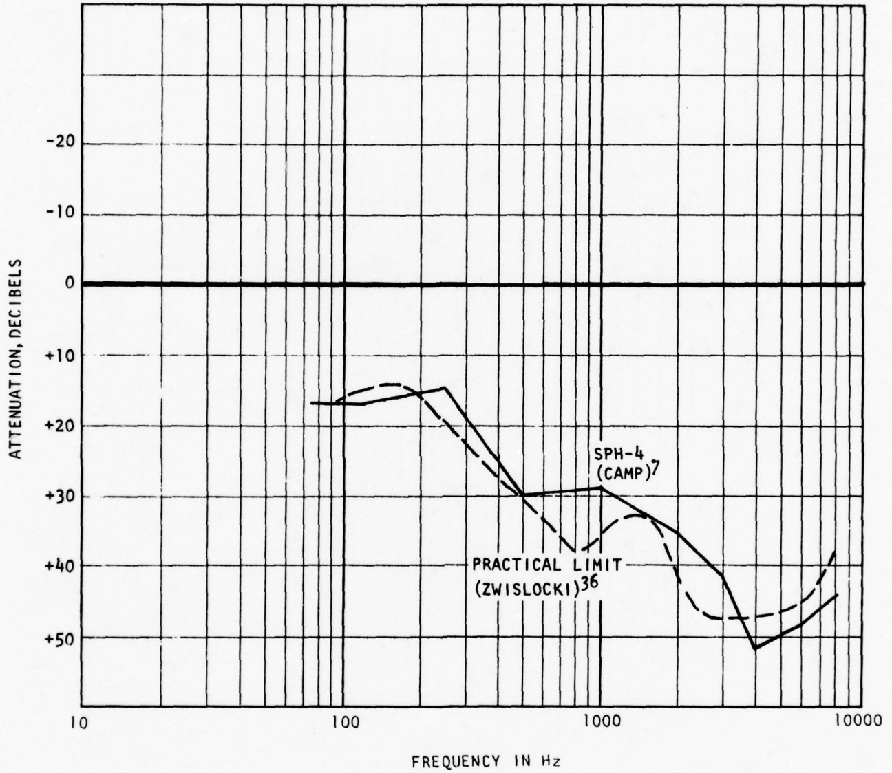
FIGURE 50. RIGID CUP WITH WAX-FILLED CUSHION (ZWISLOCKI 36 )
