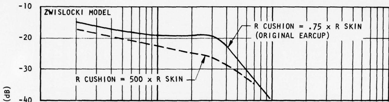
(a) Earcup Shown in Figure 8 of Shaw & Thiessen (Ref. 38) on Flexible Skin
