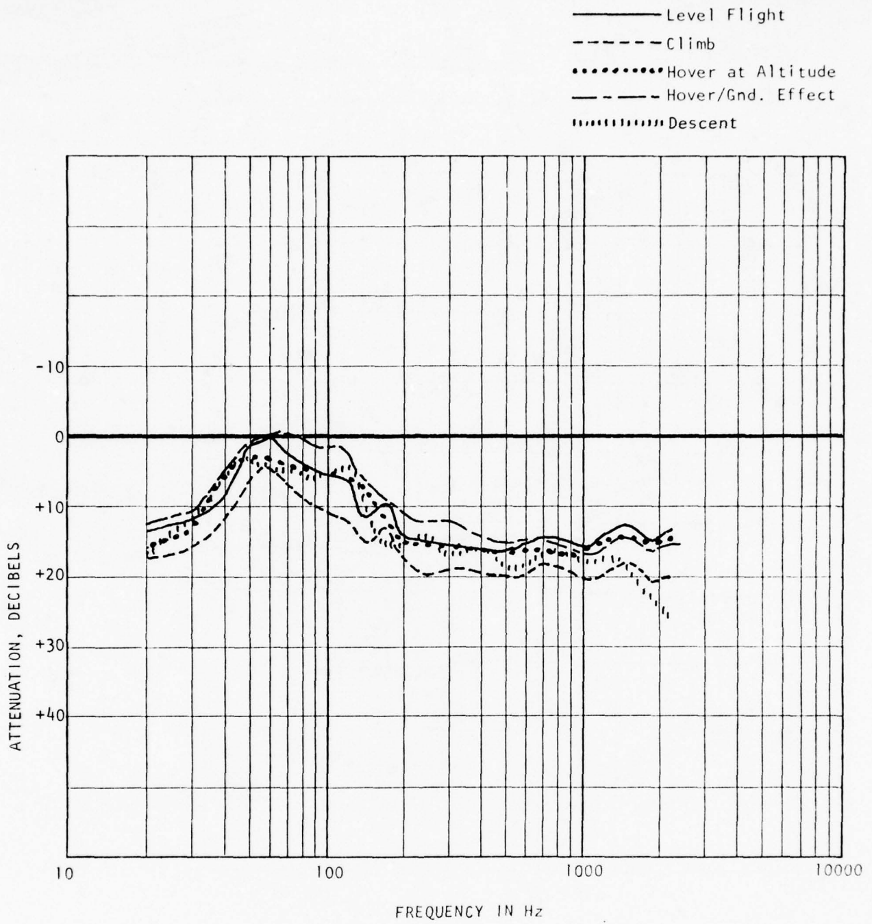
FIGURE 32 EARLUP ATTENUATION IN AN AH-1S HUEYCOBRA HELICOPTER, FOR 5 FLIGHT MODES: SAME DAY, SAME HUMAN SUBJECT
