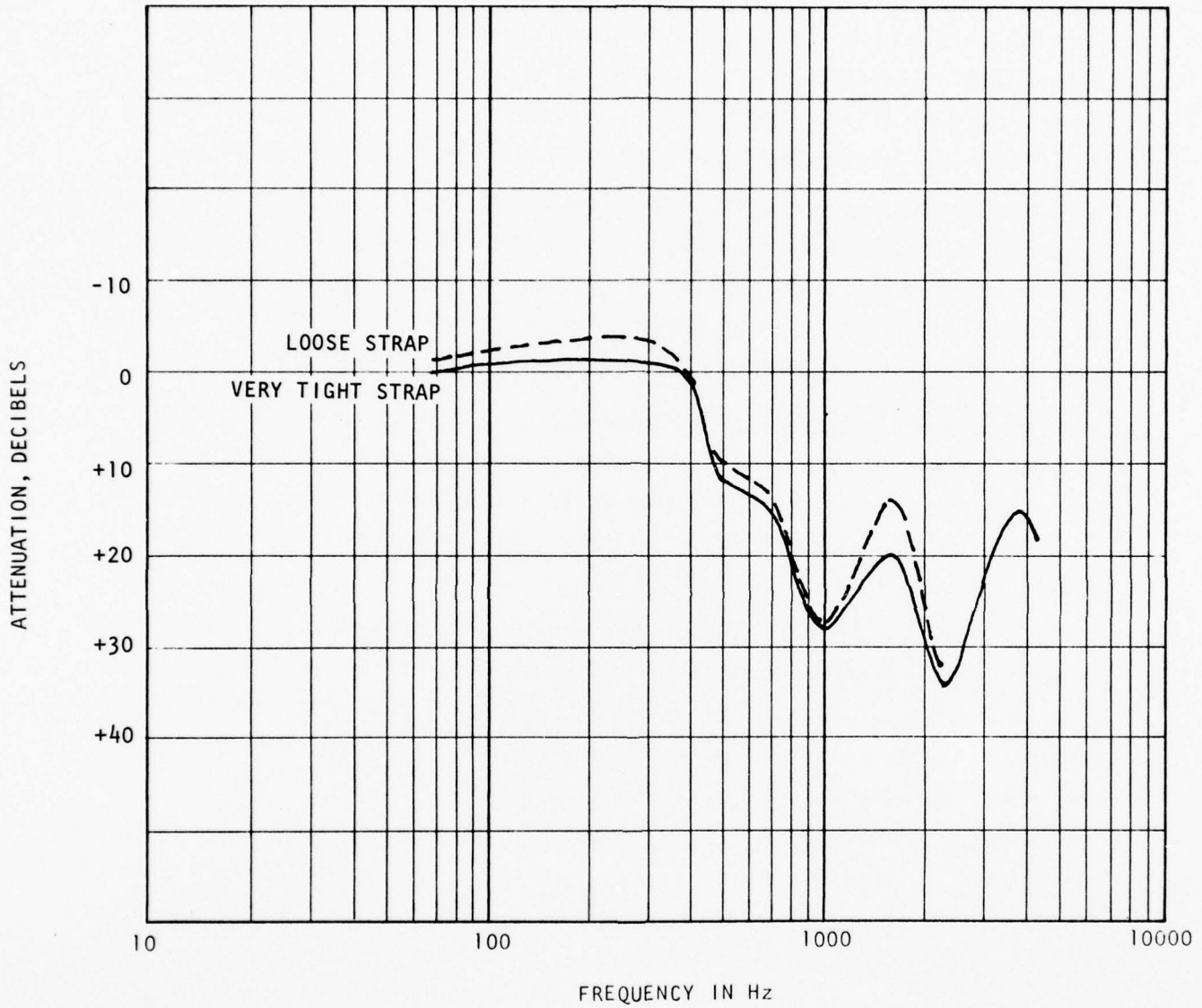
FIGURE 39 EFFECT OF VERY LONG, THICK HAIR ON MALE SUBJECT (JGC)
