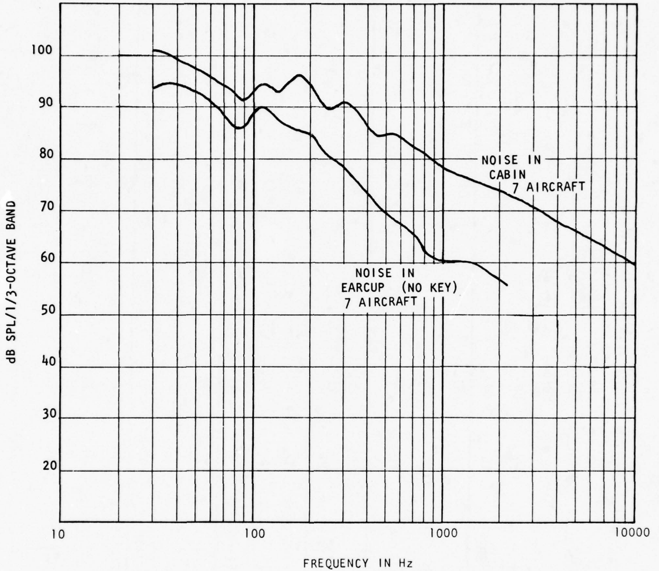
FIGURE 8 UH-1H IROQUOIS: CABIN AND EARCUP (NO KEY) NOISE DURING LEVEL FLIGHT. 1/3-OCTAVE WEIGHTED.
