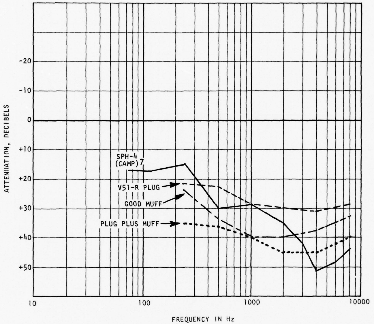
FIGURE 48. ATTENUATION OF EARCUPS AND EARPLUGS (BOTSFORD 40 )
