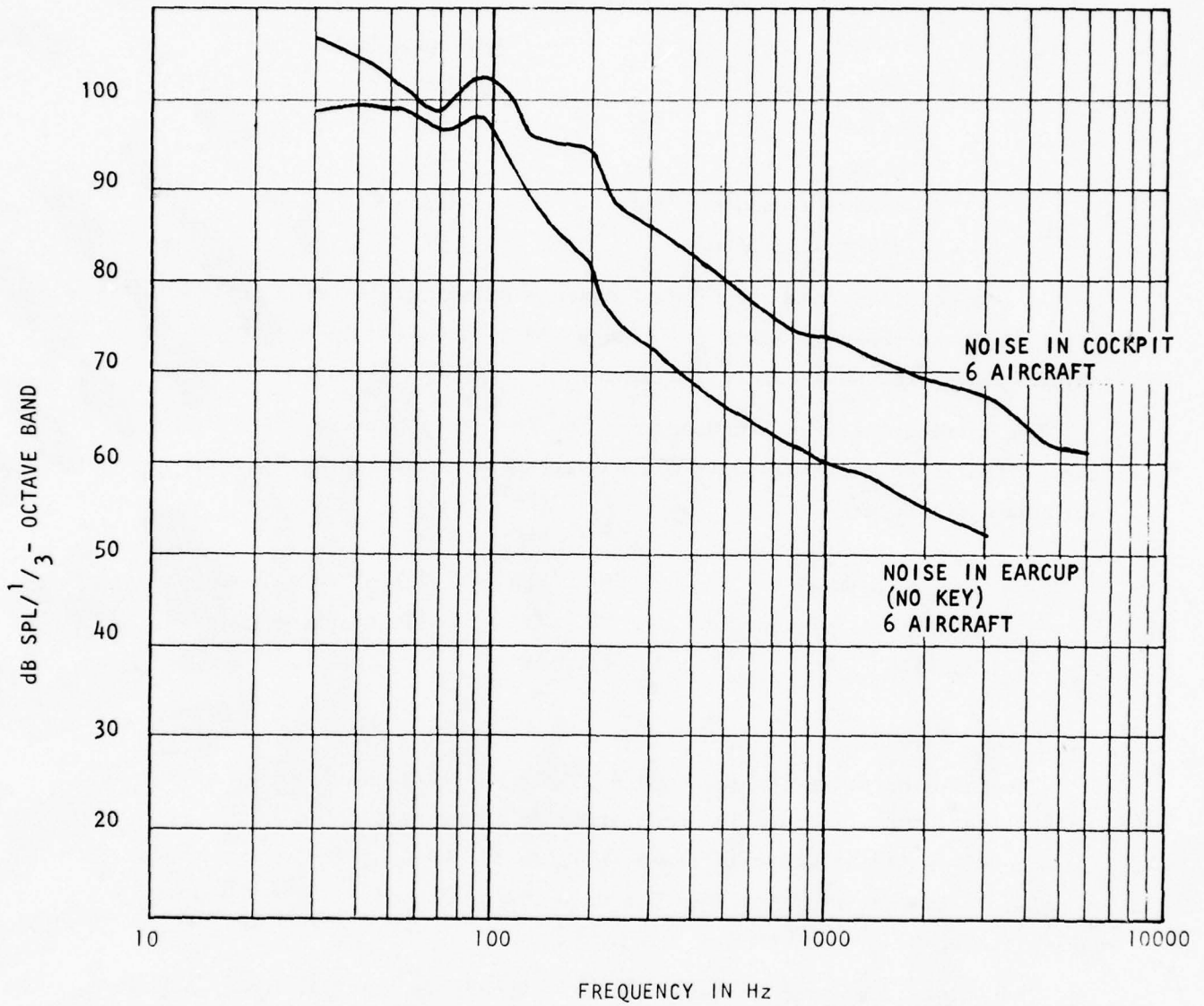
FIGURE 19 AH-1S, AH-1Q HUEYCOBRA: COCKPIT AND EARCUP (NO KEY) NOISE DURING LEVEL FLIGHT. 1/3-OCTAVE WEIGHTED.
