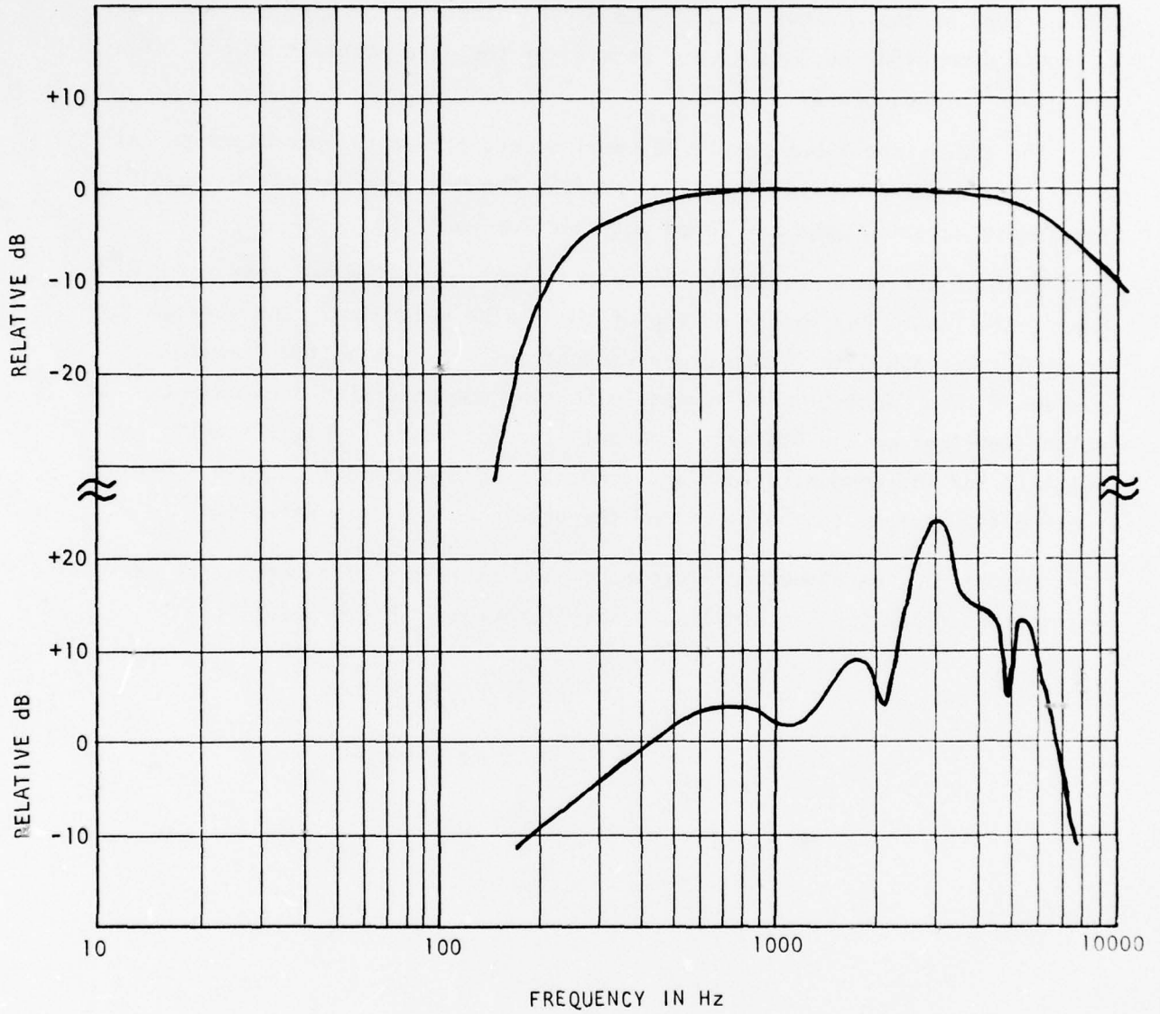
FIGURE 3 (TOP) RESPONSE OF C-1611/AIC (AVRADA MEASUREMENT)
