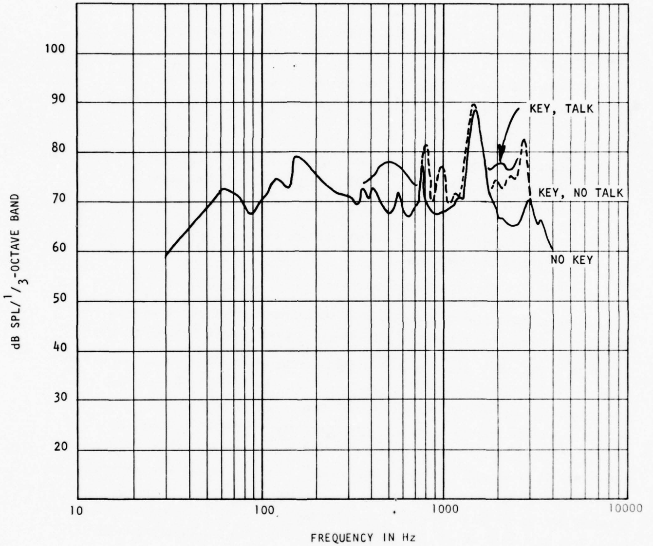
FIGURE 24 CH-47C CHINOOK: EARCUP NOISE DURING CLIMB. 1/3-OCTAVE WEIGHTED. A-WEIGHTED.
