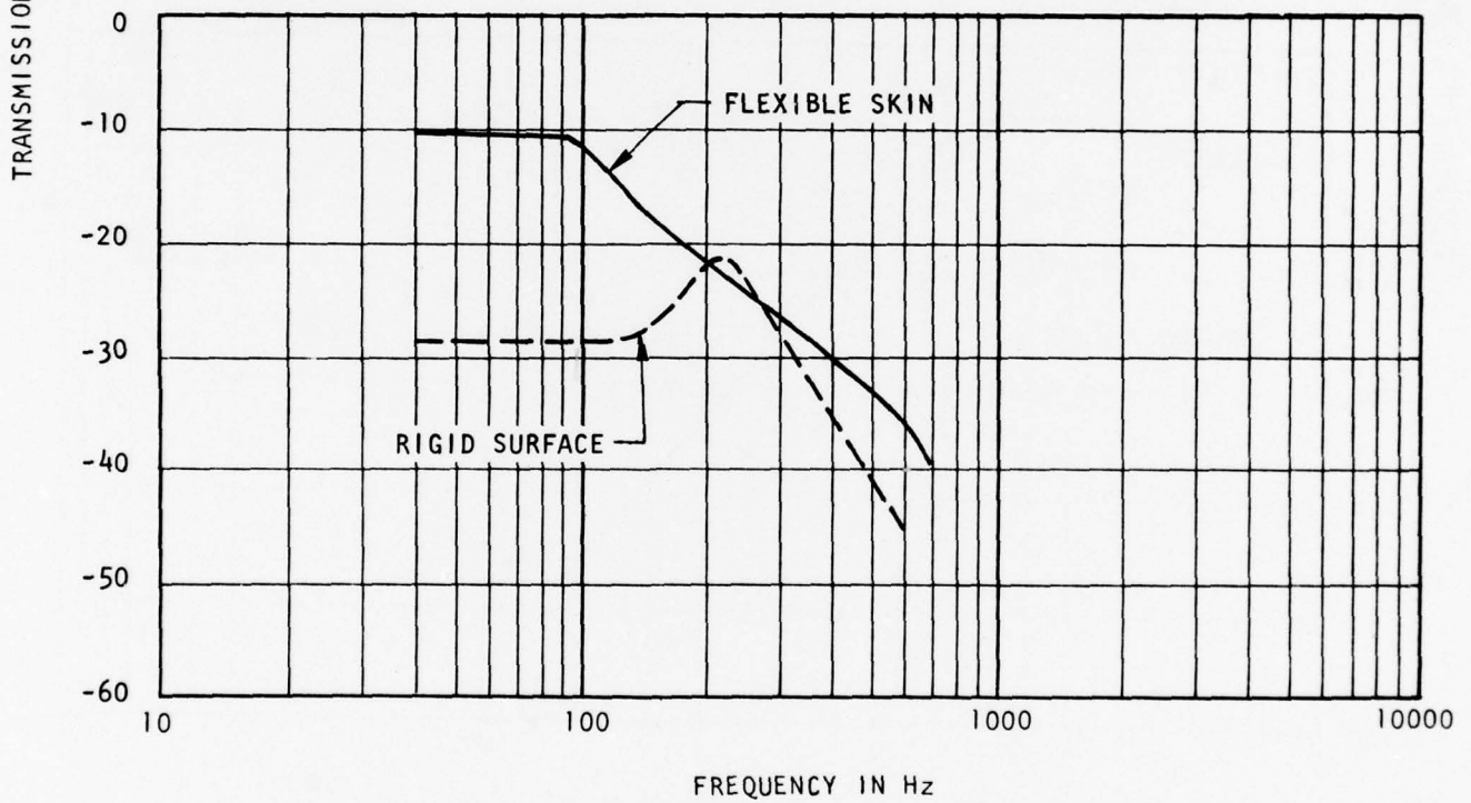
(b) Measured Effect Reported by Shaw & Thiessen 38 for the Earcup Shown in Figure 11 of their Publication
