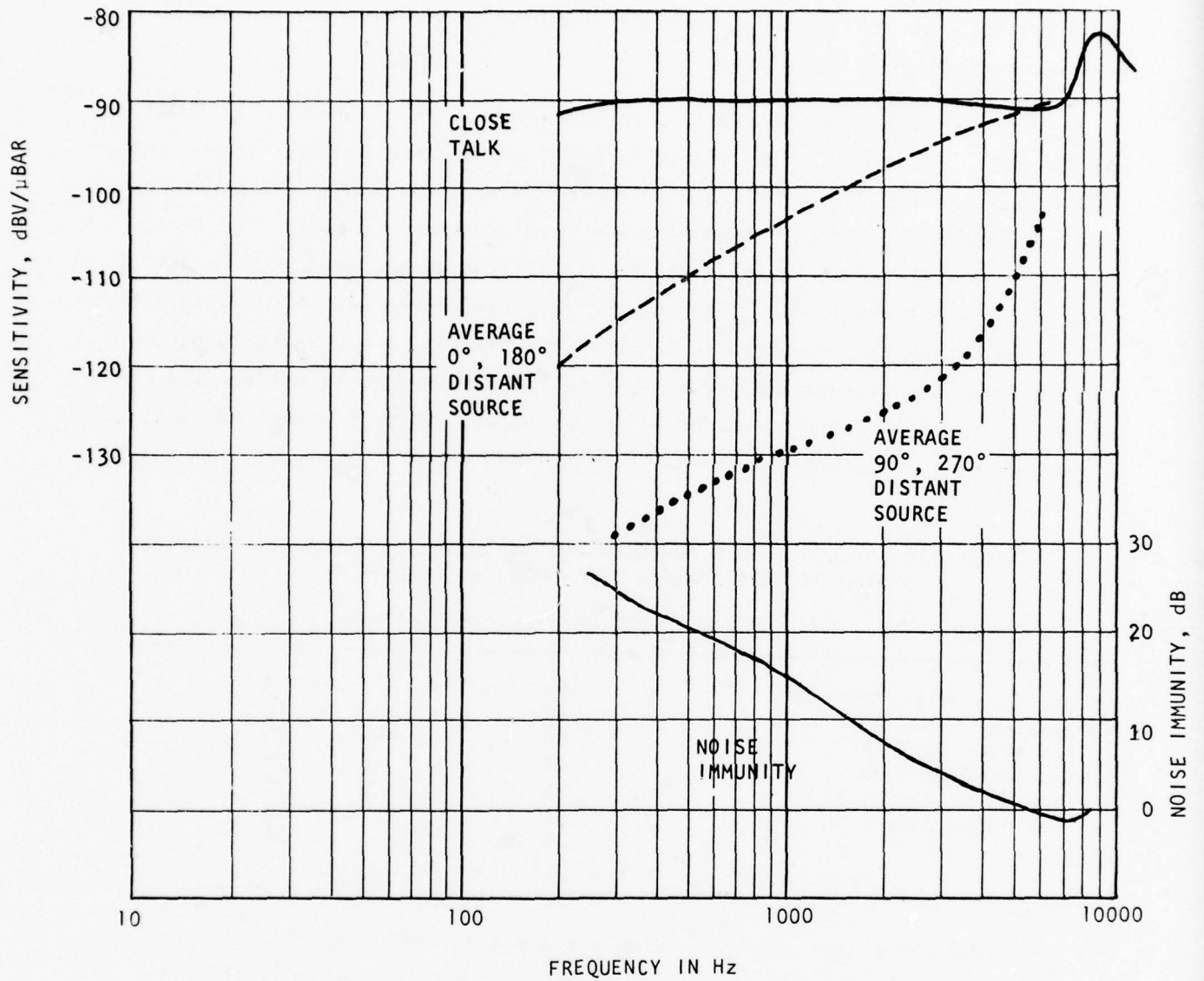
FIGURE 52. RESPONSE OF PIEZOCERAMIC NOISE-CANCELLING MICROPHONE, 150 Ω LOAD RESISTOR
