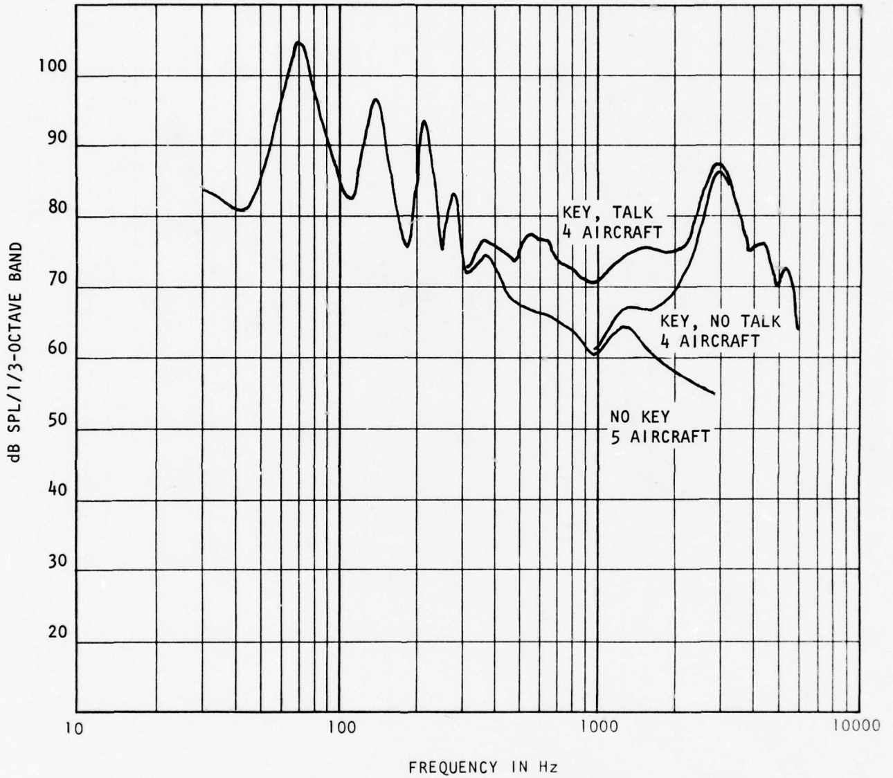
FIGURE 17 OV-10 MOHAWK: EARCUP NOISE DURING LEVEL FLIGHT. 1/3 - OCTAVE WEIGHTED.
