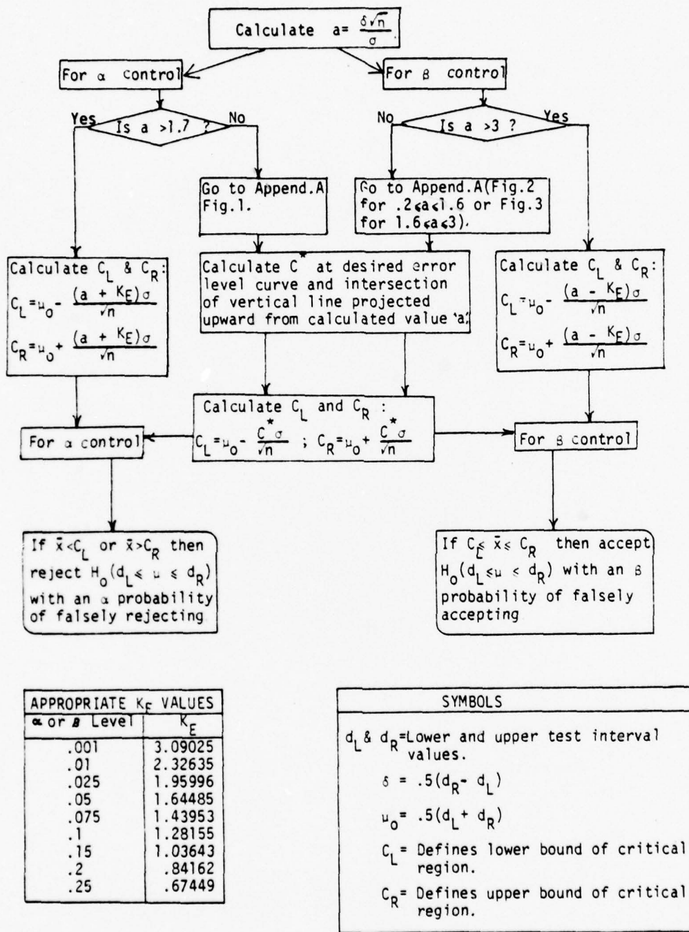
Figure 1: Algorithm For Determining \alpha or \beta Critical Regions for Known \sigma
