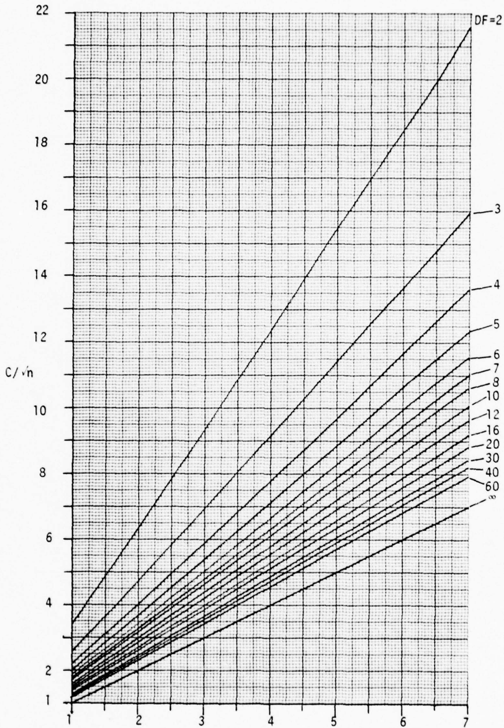
Figure A-13: C/\sqrt{n} Values For \sigma Unknown With \alpha , P_T , or 1-\beta = .1 (r \geq 1)
