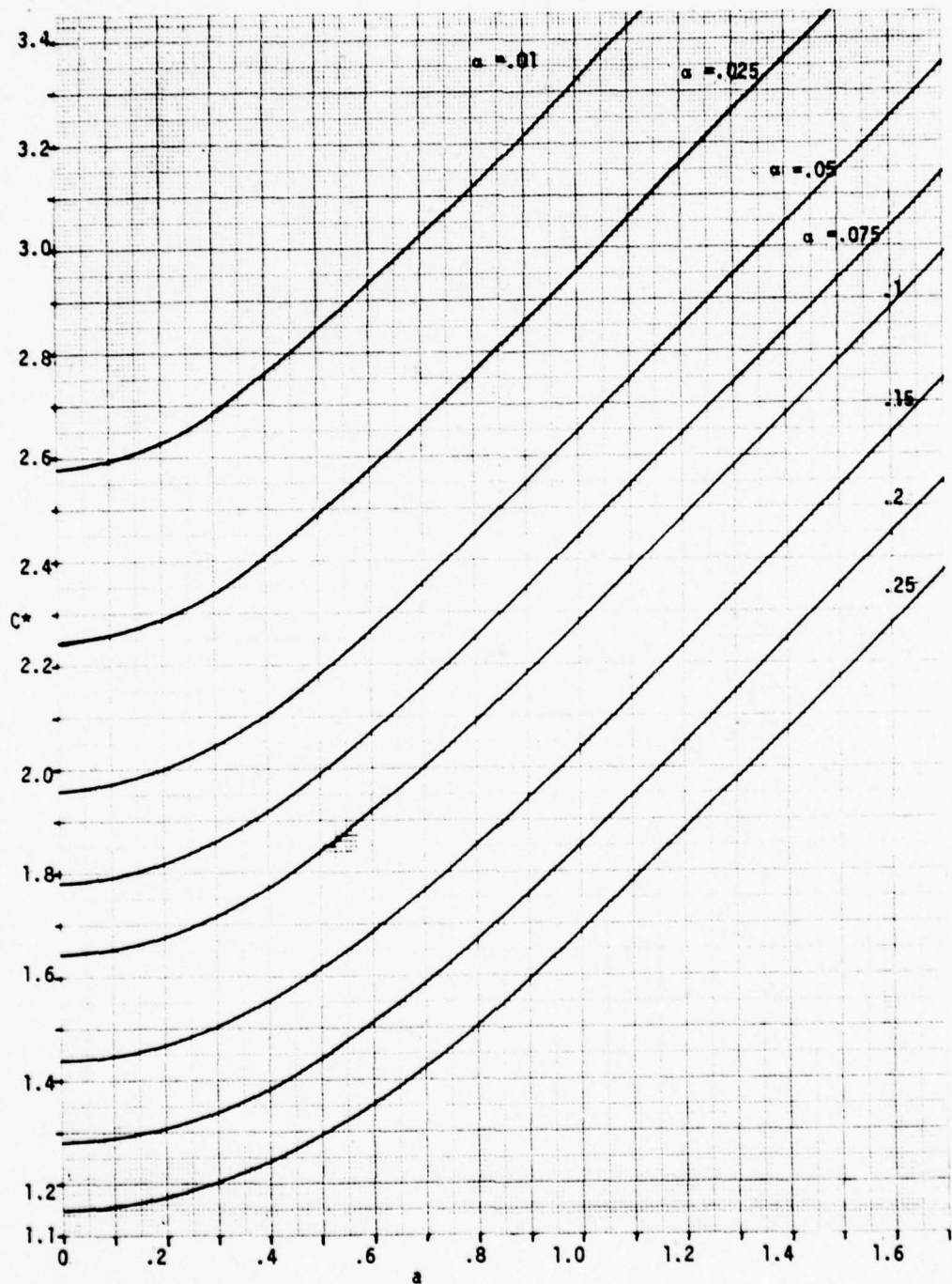
Figure A-1: C^* Values For \alpha Error Level Control With \sigma Known; ( 0 \leq \alpha \leq 1.7 )
