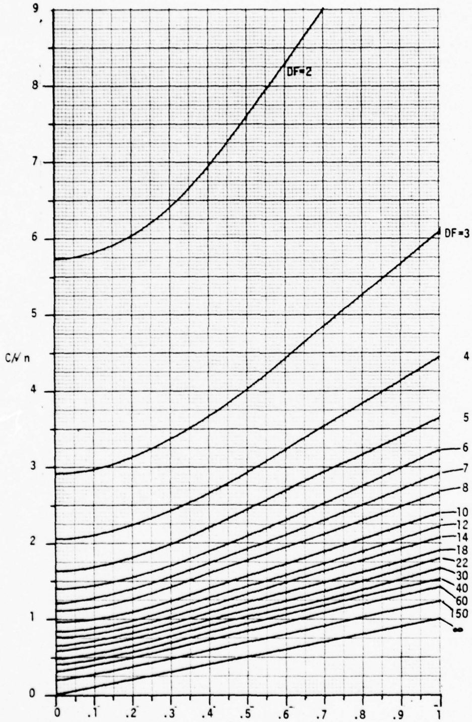
Figure A-6: C/\sqrt{n} Values For \sigma Unknown With \alpha, P_T , or 1-\beta = .01 ; ( r \leq 1 )
