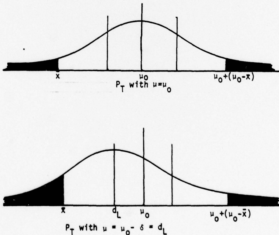
Figure C-3: Dependence of P_T on Location of True \mu Value
