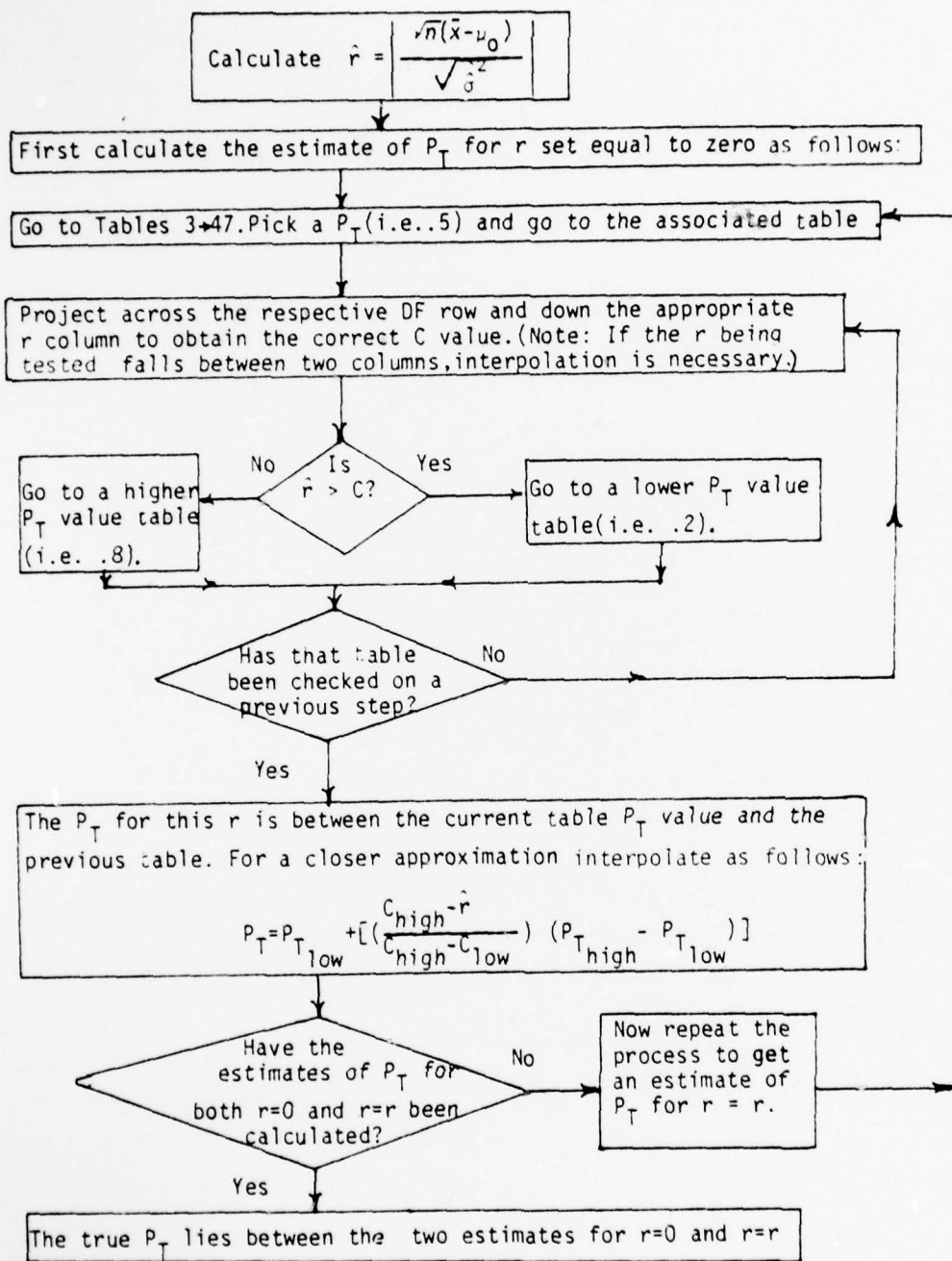
Figure 5: Algorithm For Estimating P_T For \sigma Unknown
